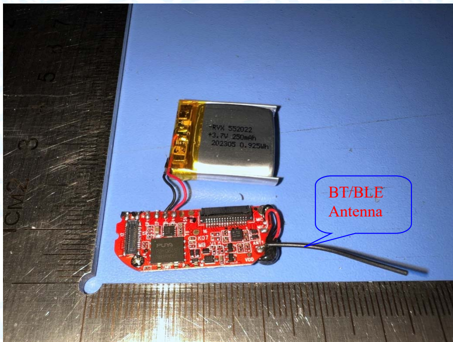
Photo 5 Appearance of PCB & Battery
