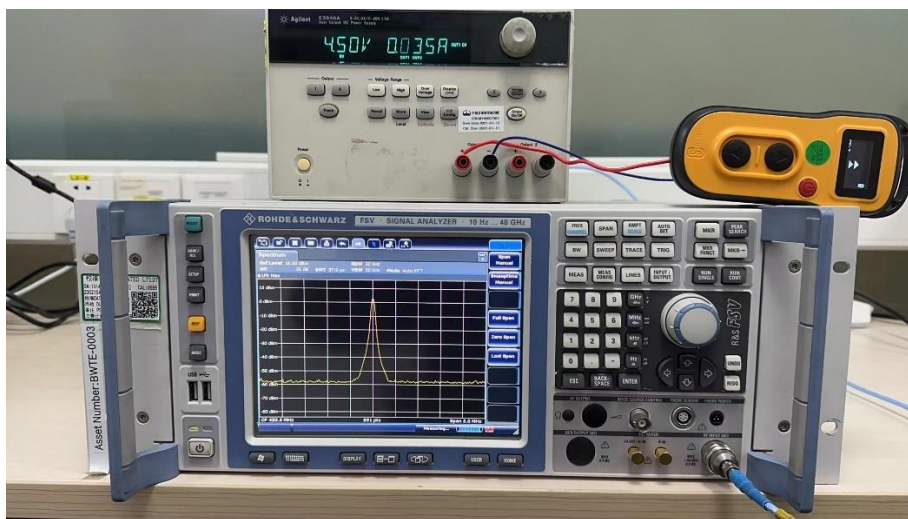
RF Conducted Test Setup
