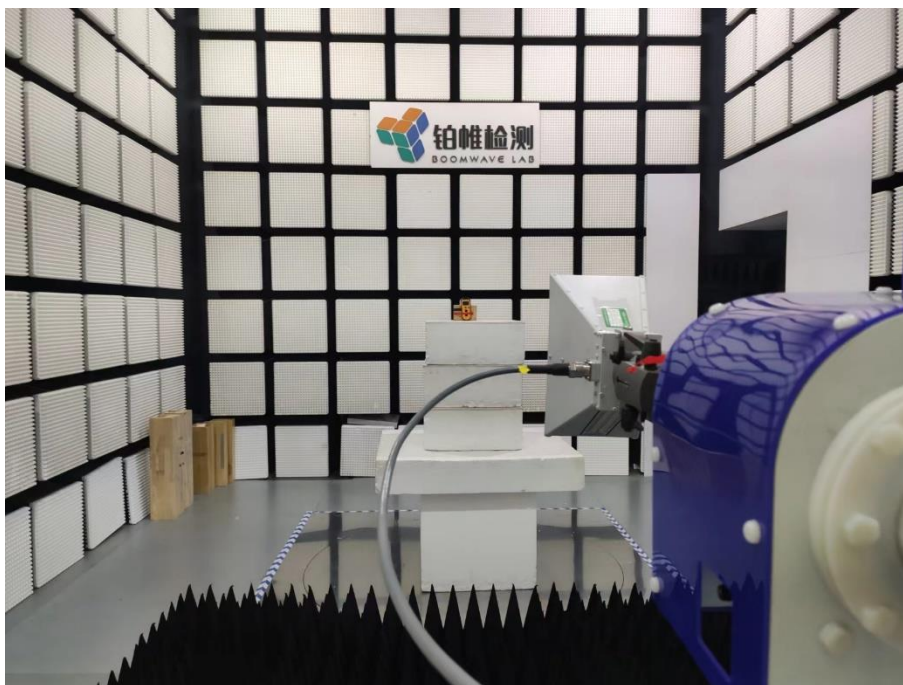
Spurious Radiated Emissions Test Setup (1GHz - 6GHz)
