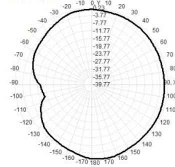
Total(H-XY), Max=-0.42dBi, CrD=14.35
