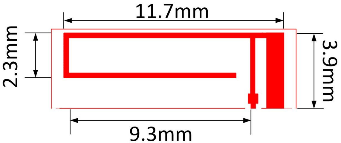
Antenna Photo & Length (mm)
