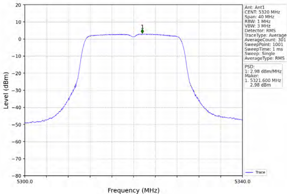
802.11ac(VHT20)_HCH_5320MHz_Ant1_NTNV
