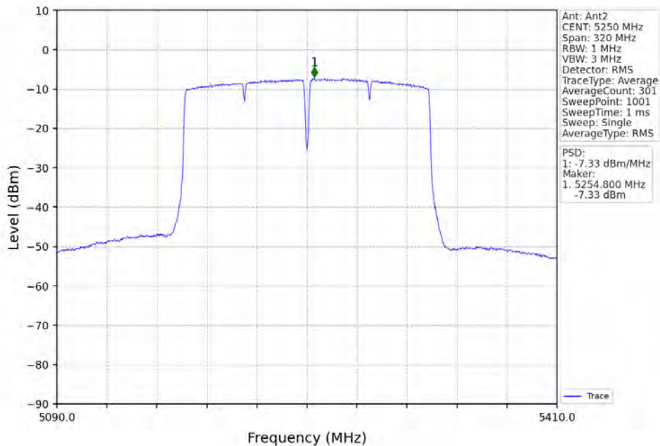
802.11ac(VHT160)_MCH_5250MHz_MIMO_NTNV
