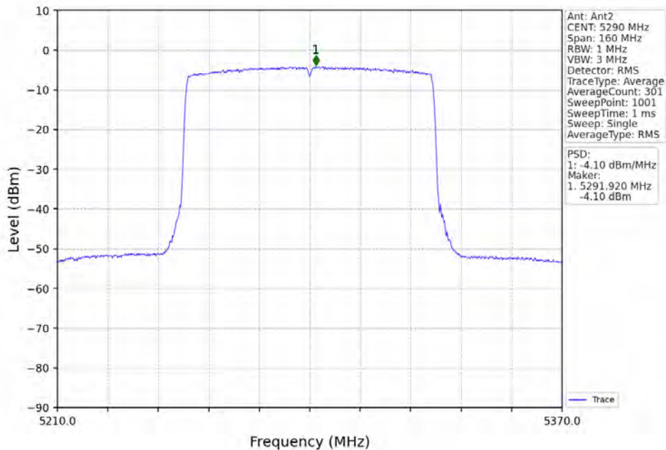
802.11ax(HEW80)_MCH_5290MHz_RU996_Left_MIMO_NTNV
