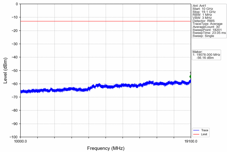
Band2_15MHz_16QAM_MCH_1880MHz_RB_1_0_NTNV
