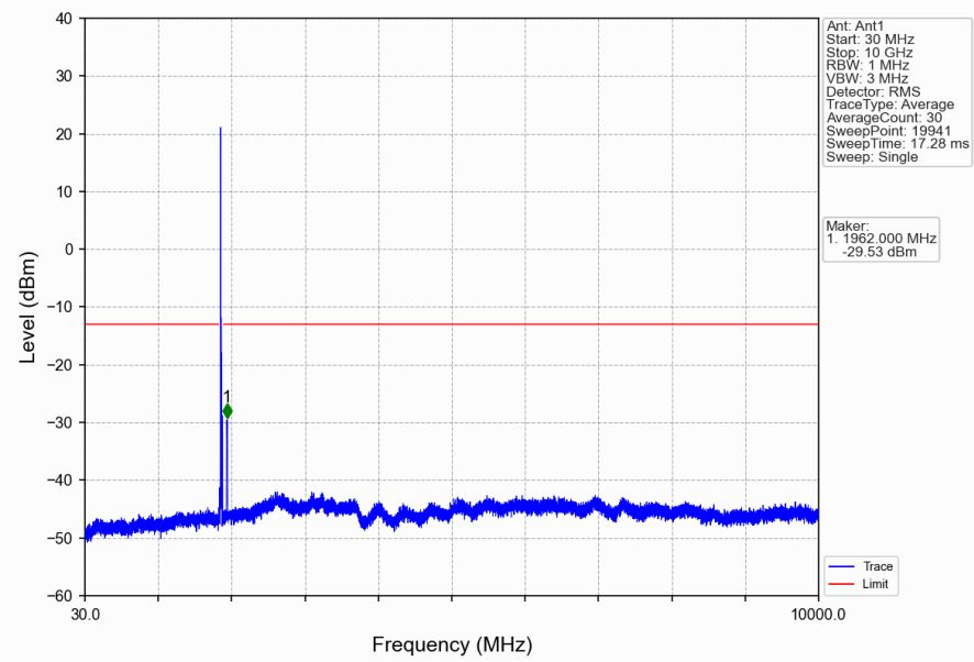
Band2_15MHz_16QAM_MCH_1880MHz_RB_1_0_NTNV
