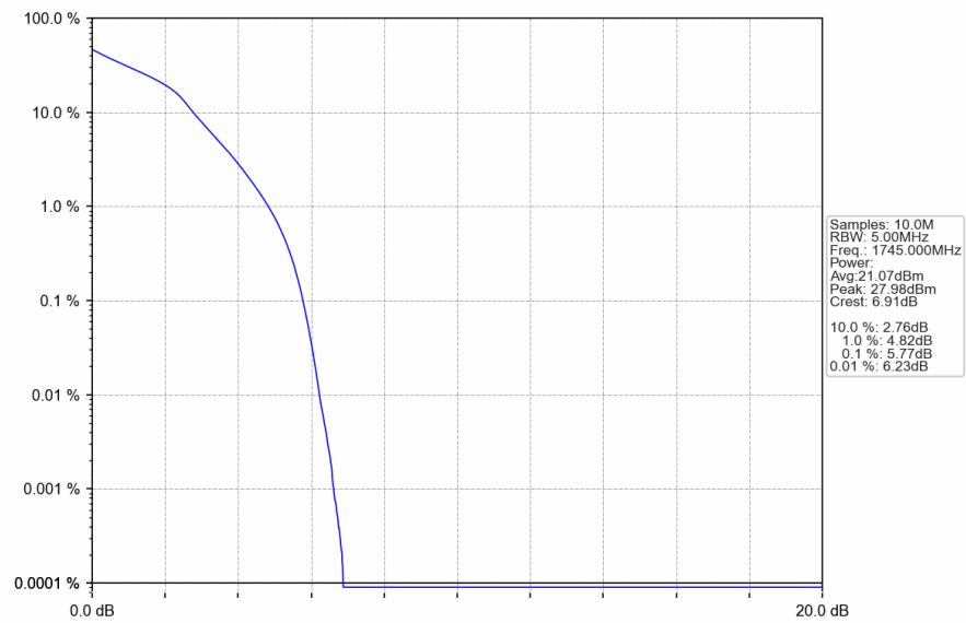
Band66_5MHz_16QAM_MCH_1745MHz_RB_25_0_NTNV
