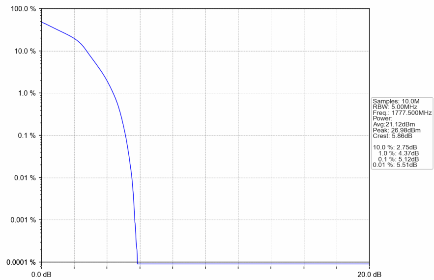
Band66_5MHz_16QAM_HCH_1777.5MHz_RB_25_0_NTNV
