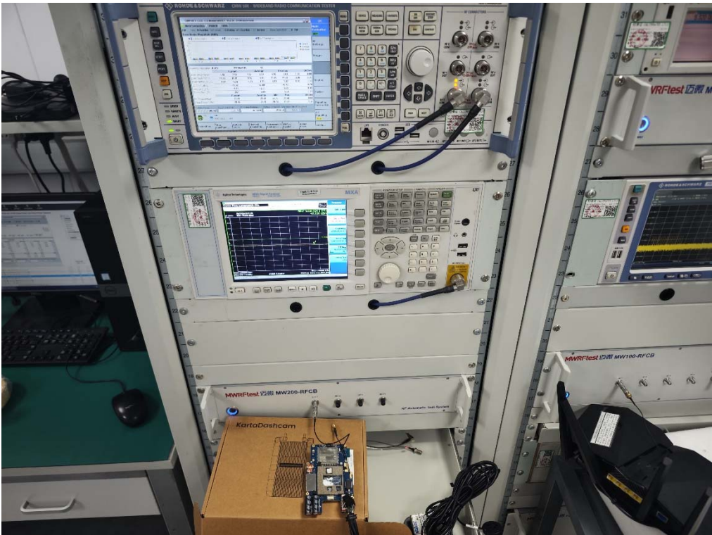
RF Conducted Measurement Photos
