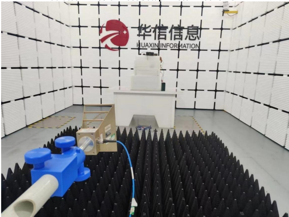
Radiated Emission Test Setup Photo - Above 1GHz
