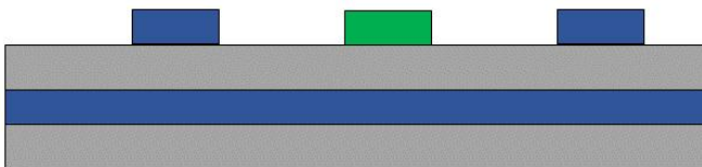
MODE 1 - Reference ground is the second layer PCB coplanar transmission line
