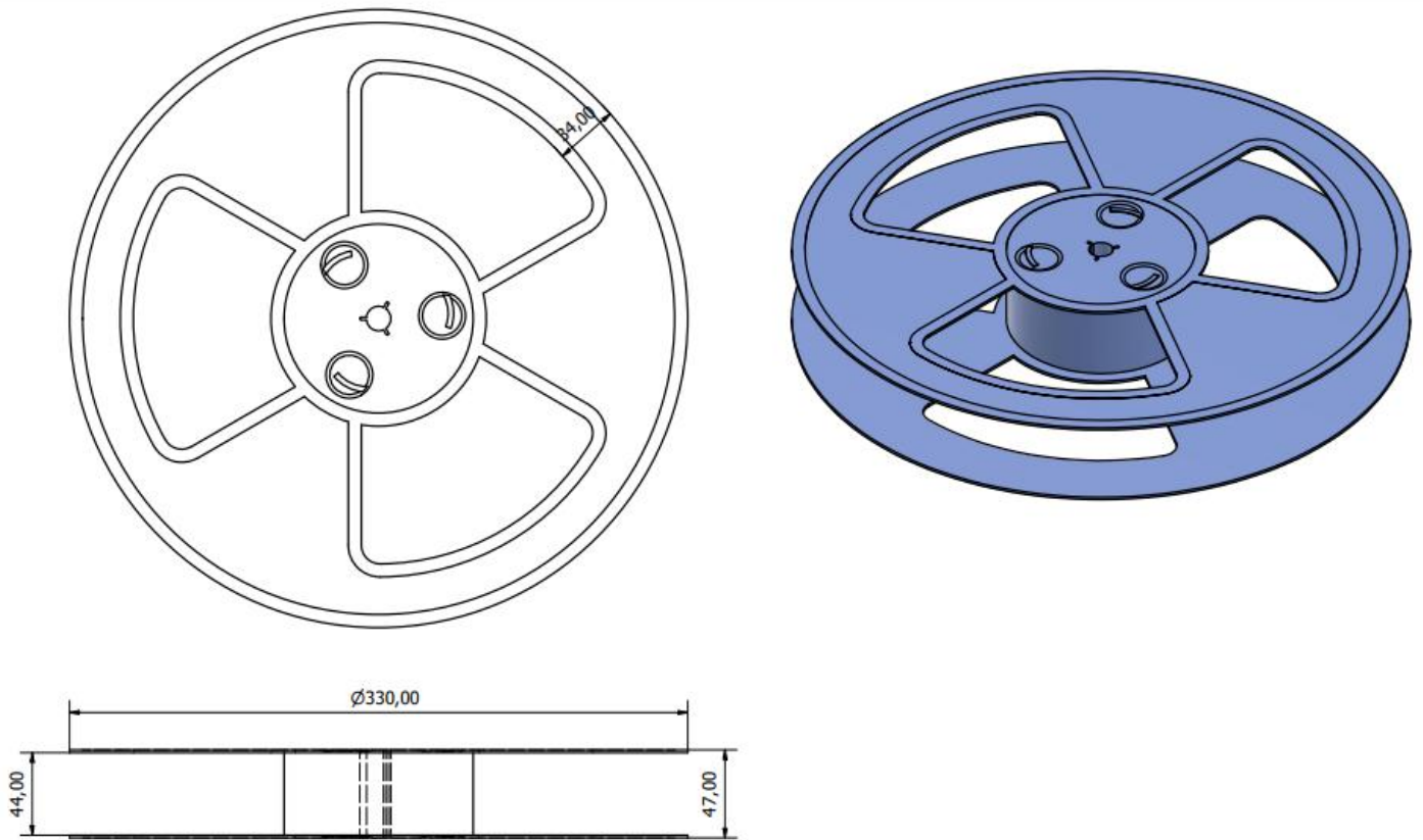
Figure 31 Reel Dimensions of C16QS (in mm)
