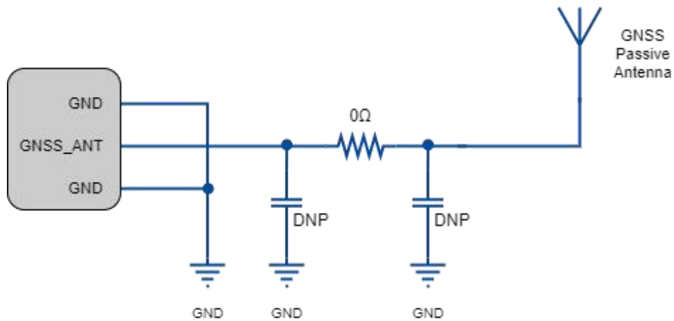
Figure 17 GNSS passive antenna matching circuit
