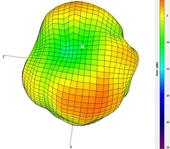
Pattern 2445Mhz
