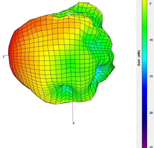
Pattern 5240Mhz
