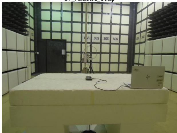
WLAN 2.4G_Radiated_Setup
