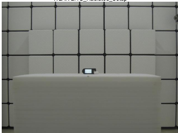
WLAN 2.4G_Radiated_Setup
