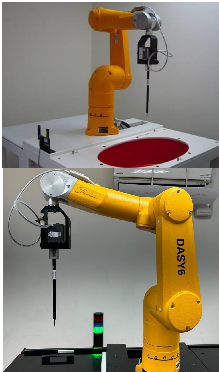
Fig.1 Photograph of the SAR measurement system
