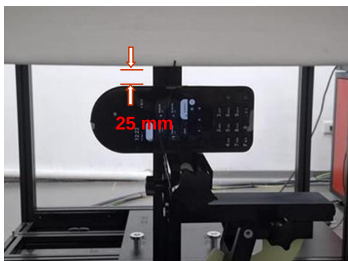
Photograph 1. Body, Right Edge, 25mm
