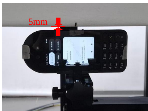
Photograph 11. Body, Right Edge, 5mm
