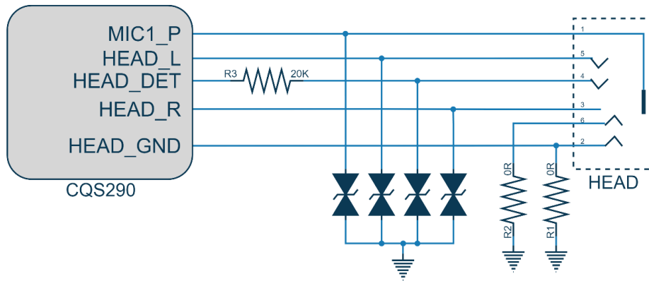
Figure 23 Head Jack
