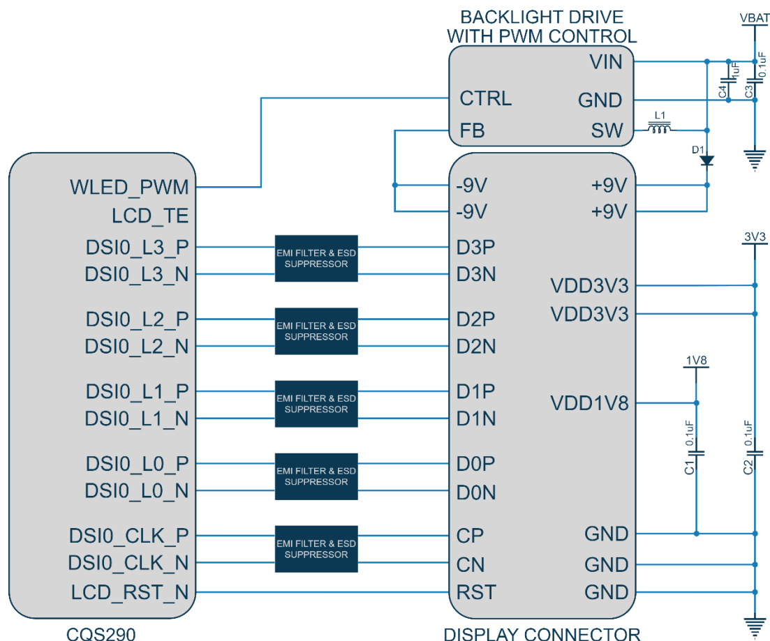
Figure 19 MIPI-DSI interface
