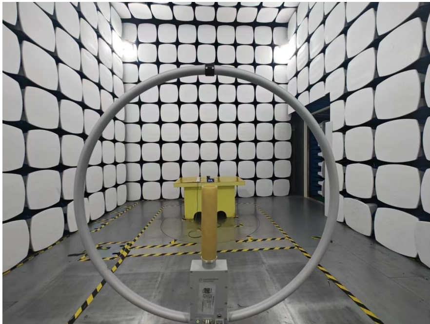
Radiated spurious emissions 9kHz–30MHz for mode 2 to mode 5
