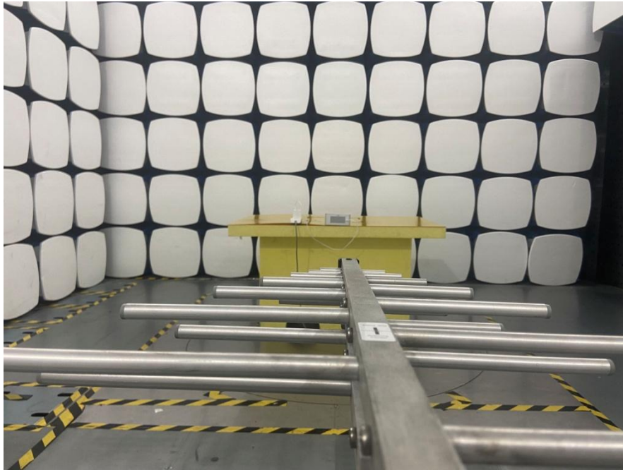
Radiated spurious emissions 30MHz to 1GHz for mode 1
