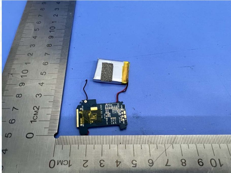
Photo 7 Appearance of PCB & Battery
