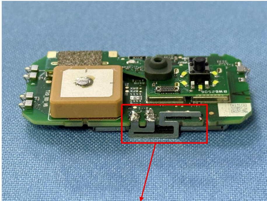
2.4G WIFI RX Antenna
