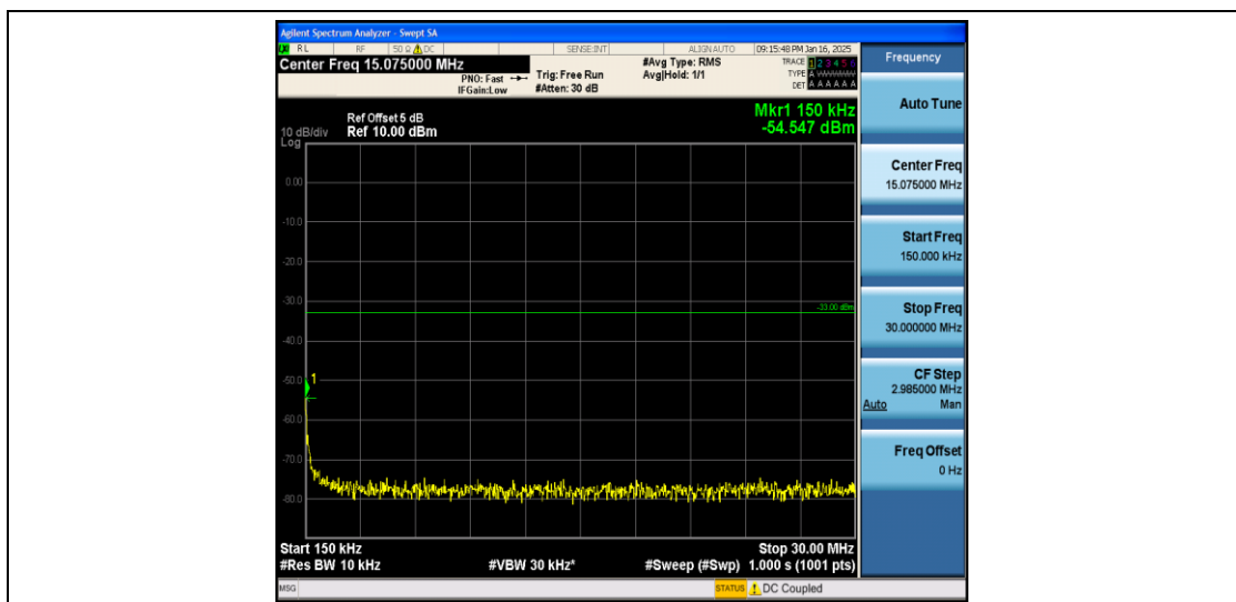
Band2_5MHz_QPSK_18625_1RB#0_0.15~30_0.15~30
