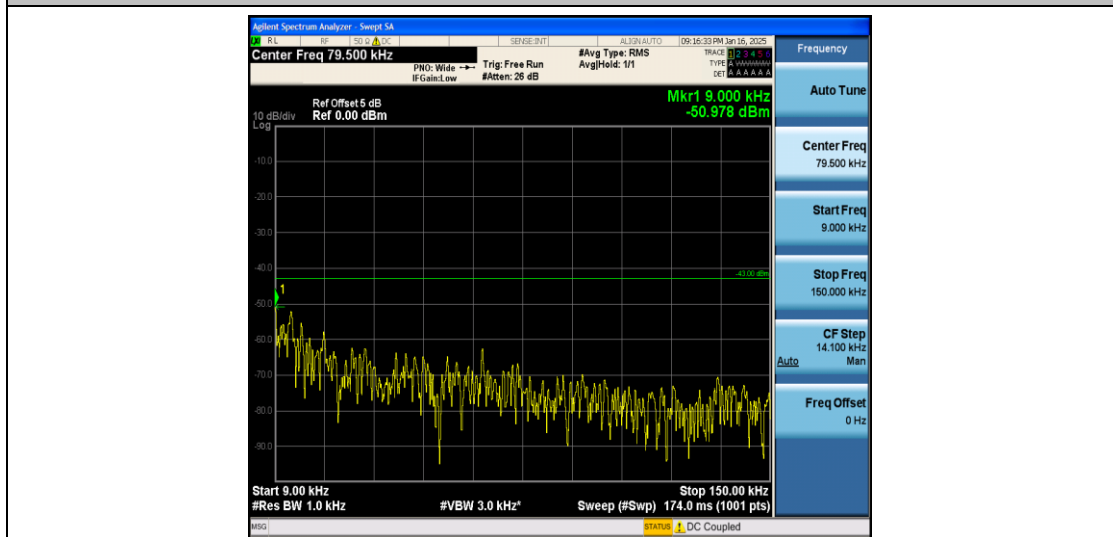
Band2_5MHz_16QAM_18625_1RB#0_0.009~0.15_0.009~0.15
