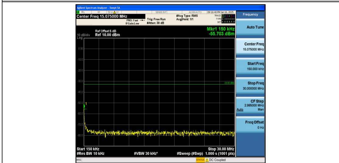
Band2_5MHz_16QAM_18625_1RB#0_0.15~30_0.15~30
