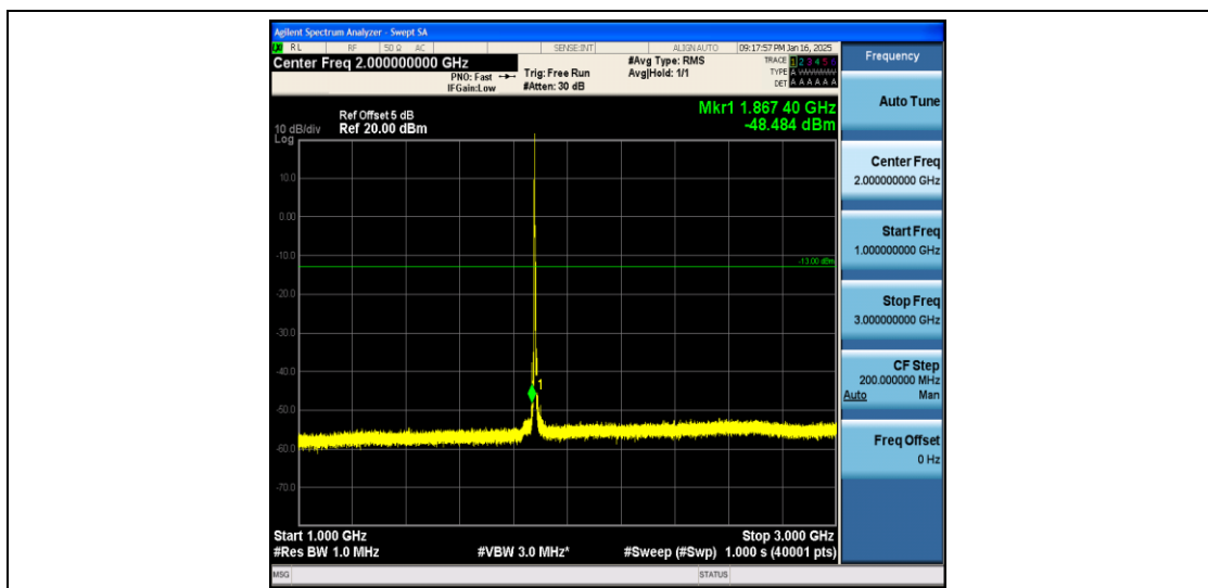
Band2_5MHz_QPSK_18900_1RB#0_1000~3000_1000~3000
