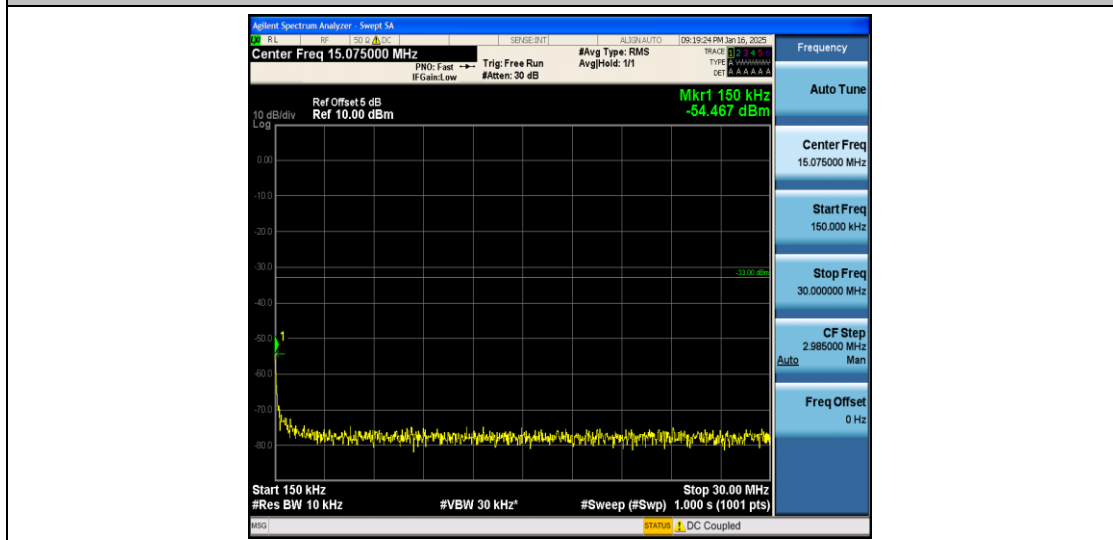
Band2_5MHz_QPSK_19175_1RB#0_0.15~30_0.15~30
