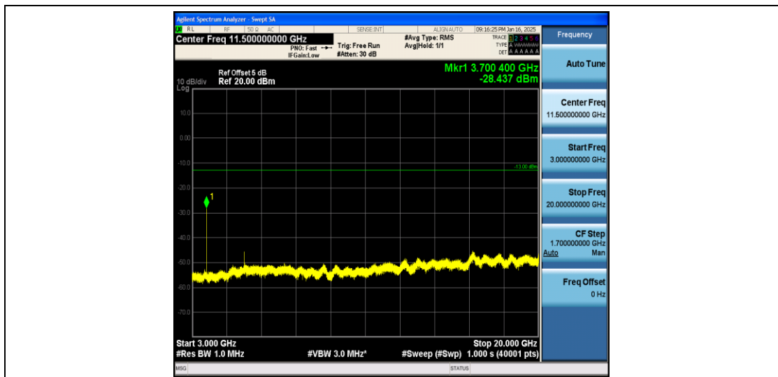
Band2_5MHz_QPSK_18625_1RB#0_3000~20000_3000~20000
