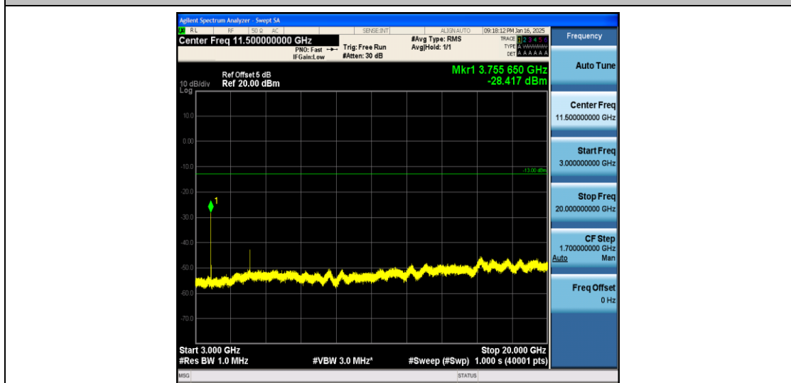
Band2_5MHz_QPSK_18900_1RB#0_3000~20000_3000~20000
