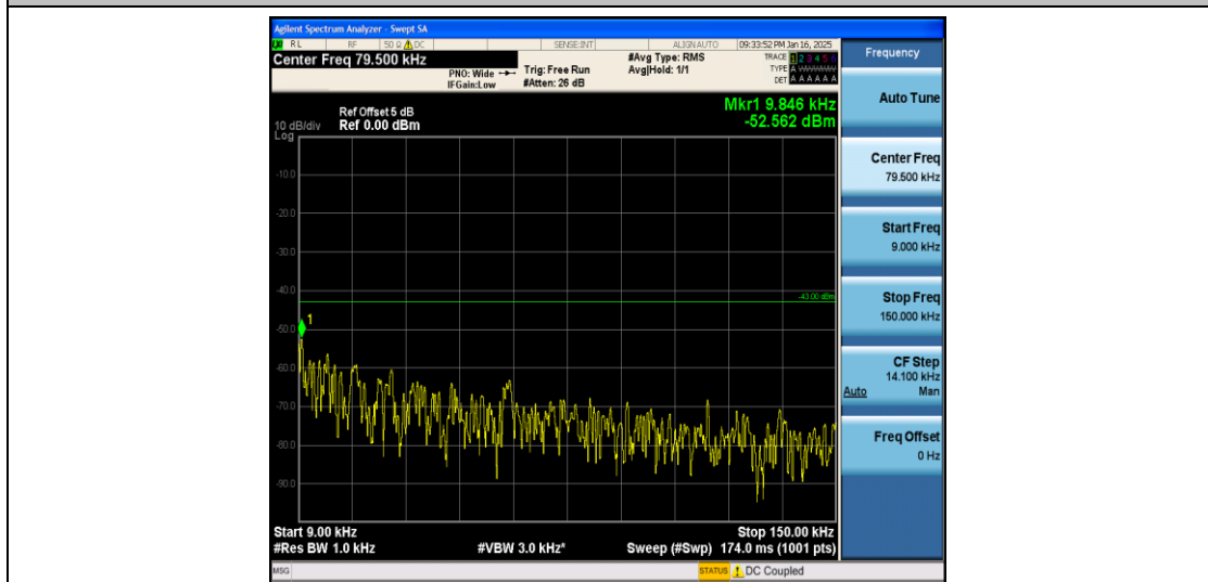
Band2_10MHz_QPSK_19150_1RB#0_0.009~0.15_0.009~0.15
