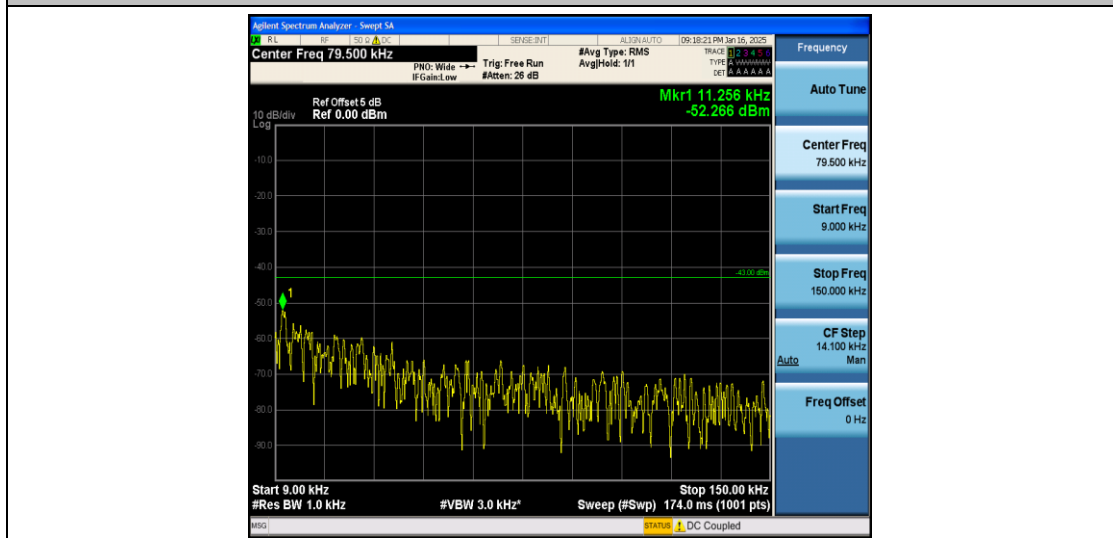
Band2_5MHz_16QAM_18900_1RB#0_0.009~0.15_0.009~0.15
