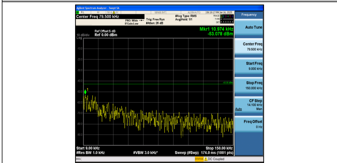
Band2_5MHz_QPSK_19175_1RB#0_0.009~0.15_0.009~0.15
