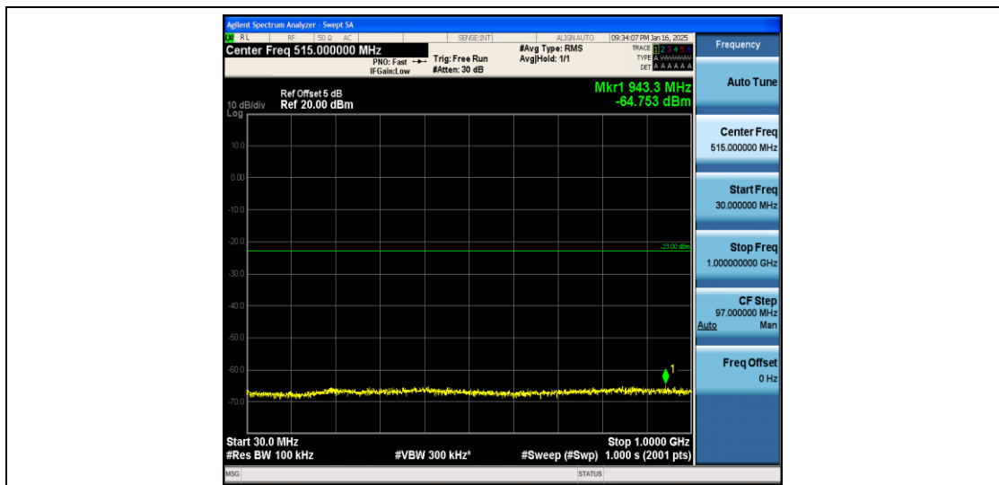
Band2_10MHz_QPSK_19150_1RB#0_30~1000_30~1000
