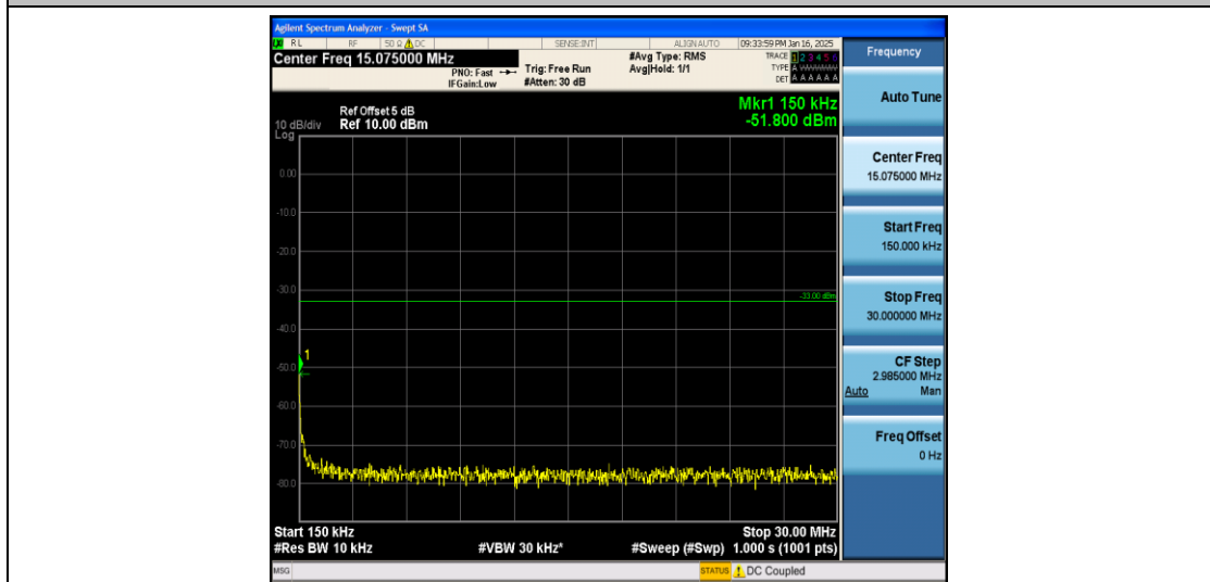
Band2_10MHz_QPSK_19150_1RB#0_0.15~30_0.15~30
