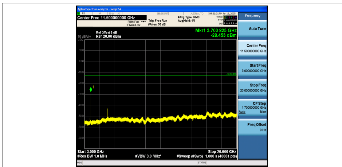
Band2_10MHz_QPSK_18650_1RB#0_3000~20000_3000~20000
