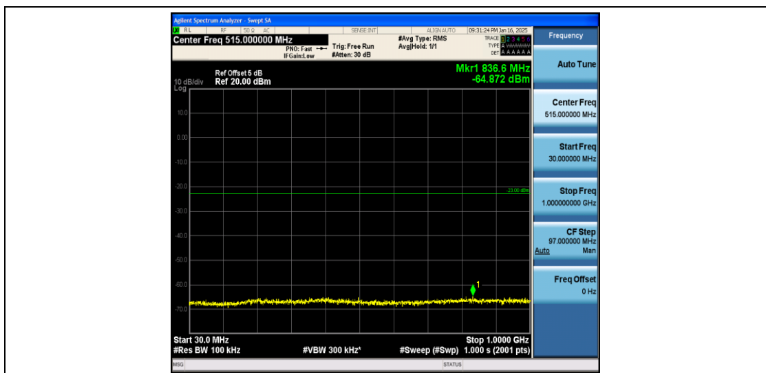
Band2_10MHz_16QAM_18650_1RB#0_30~1000_30~1000
