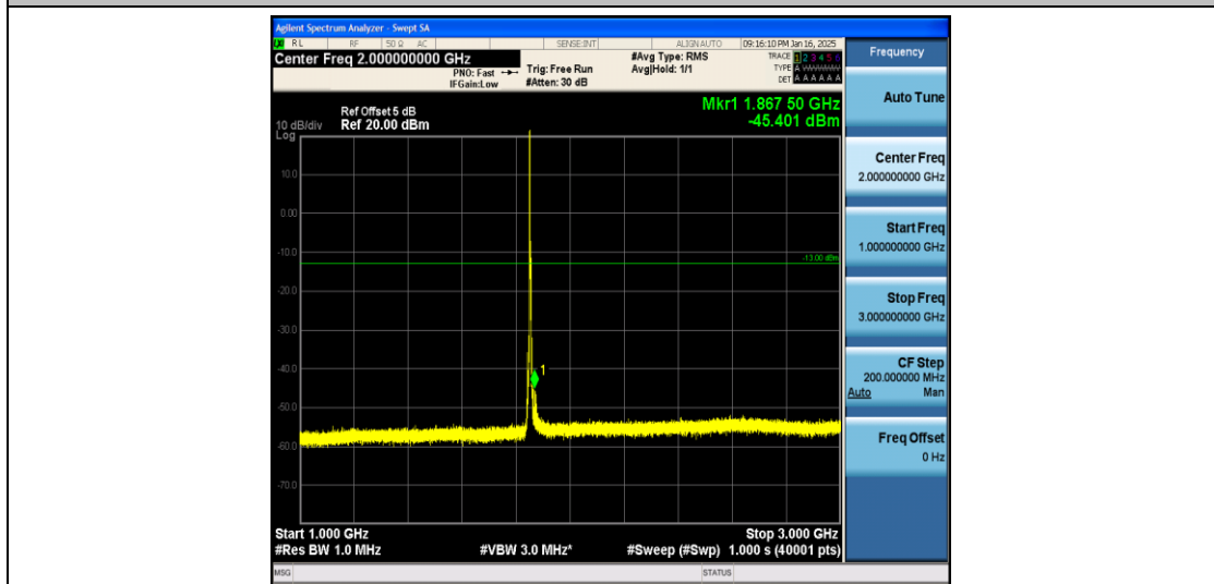
Band2_5MHz_QPSK_18625_1RB#0_1000~3000_1000~3000
