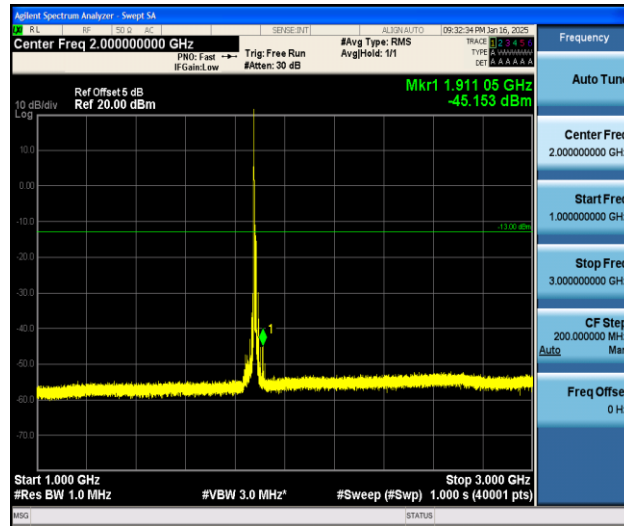
Band2_10MHz_QPSK_18900_1RB#0_1000~3000_1000~3000
