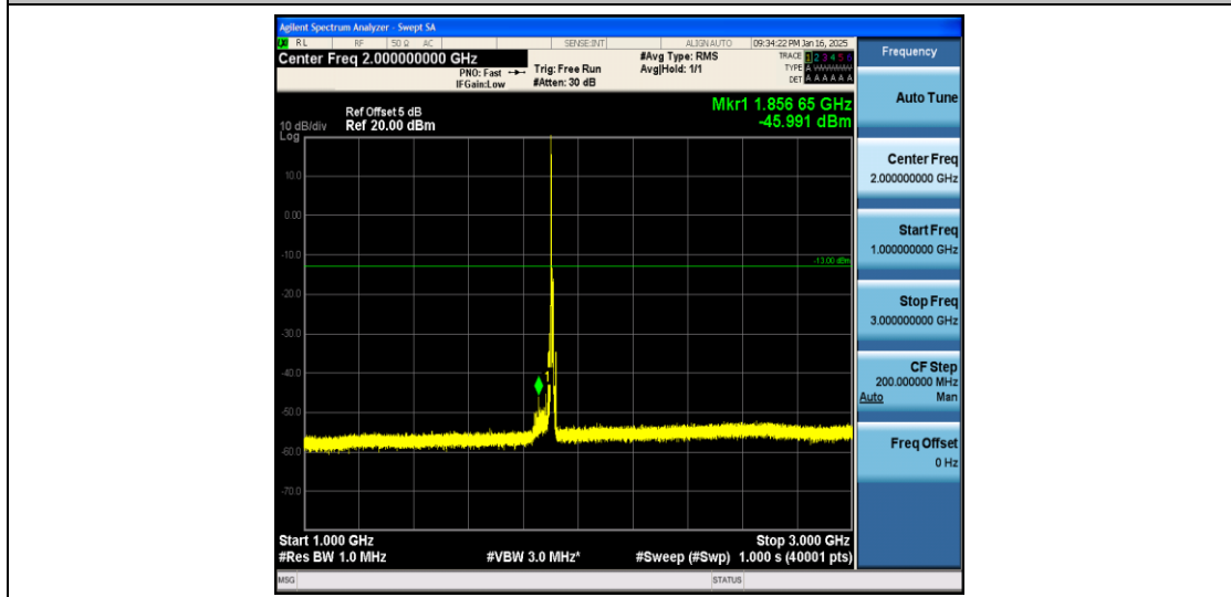
Band2_10MHz_QPSK_19150_1RB#0_1000~3000_1000~3000
