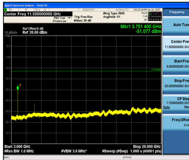
Band2_10MHz_QPSK_18900_1RB#0_3000~20000_3000~20000
