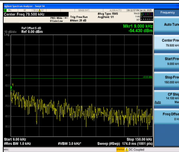
Band2_10MHz_16QAM_18900_1RB#0_0.009~0.15_0.009~0.15
