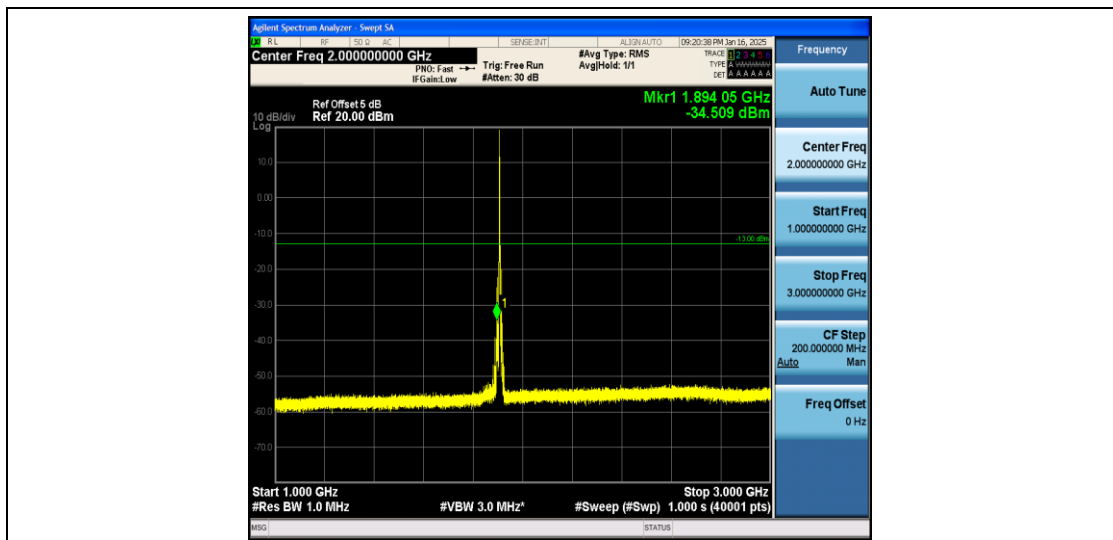
Band2_5MHz_16QAM_19175_1RB#0_1000~3000_1000~3000
