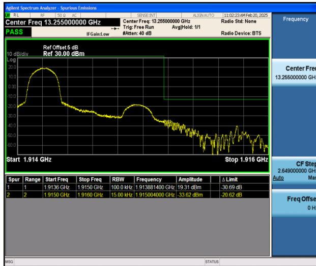
Band25_1.4MHz_QPSK_26683_1RB#0
