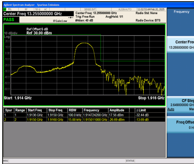
Band25_1.4MHz_16QAM_26683_1RB#5
