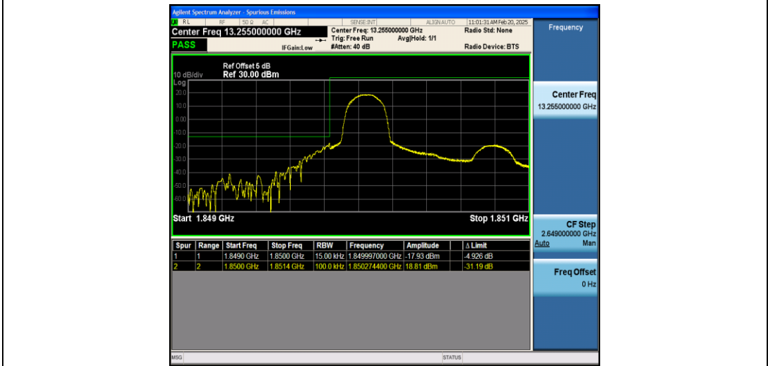
Band25_1.4MHz_16QAM_26047_1RB#0
