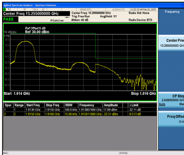
Band25_1.4MHz_16QAM_26683_1RB#0
