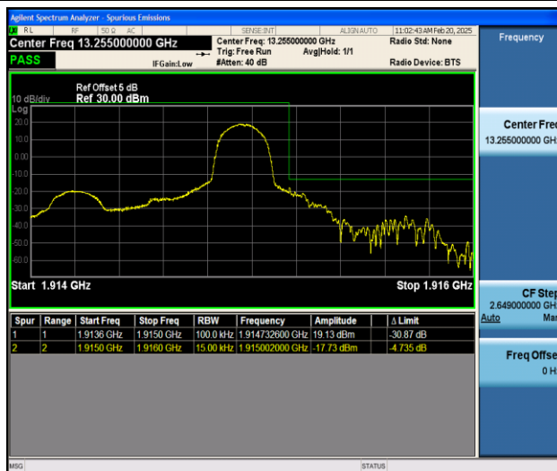
Band25_1.4MHz_QPSK_26683_1RB#5
