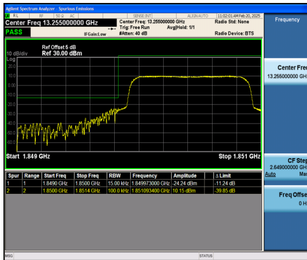
Band25_1.4MHz_QPSK_26047_6RB#0
