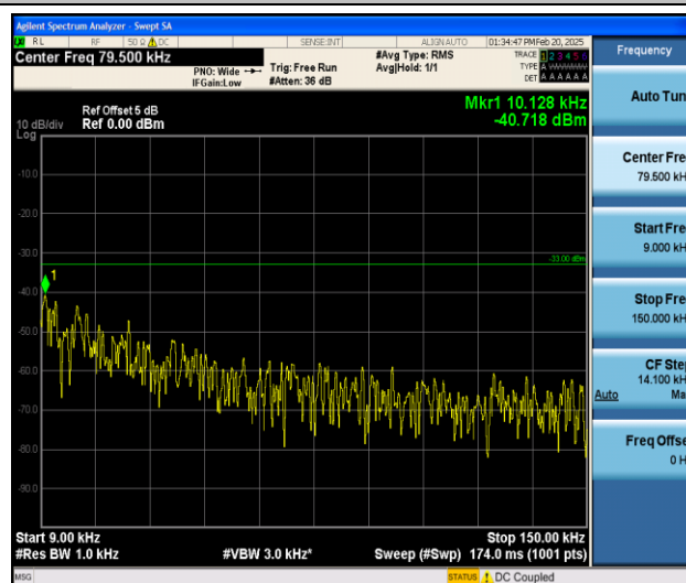
Band26_3MHz_QPSK_27025_1RB#0_0.009~0.15_0.009~0.15
