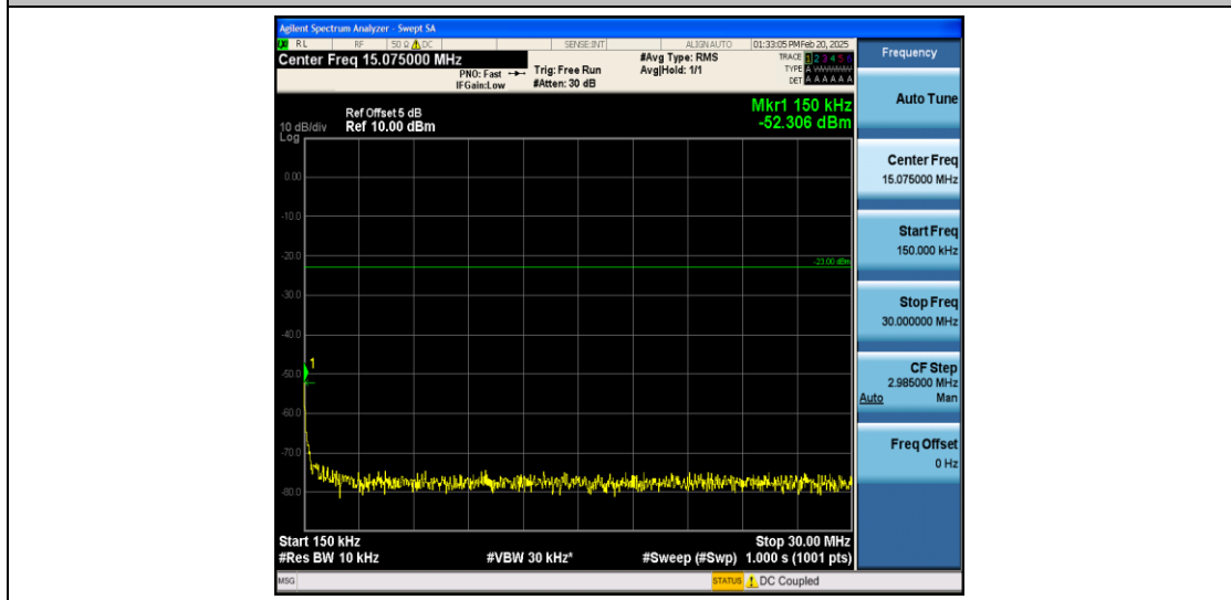
Band26_3MHz_QPSK_26915_1RB#0_0.15~30_0.15~30
