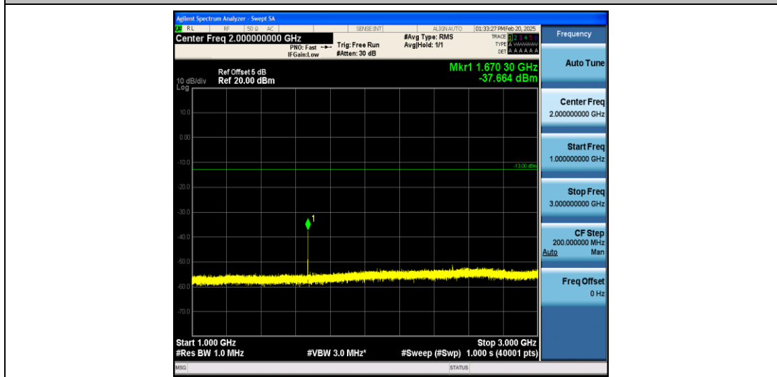
Band26_3MHz_QPSK_26915_1RB#0_1000~3000_1000~3000
