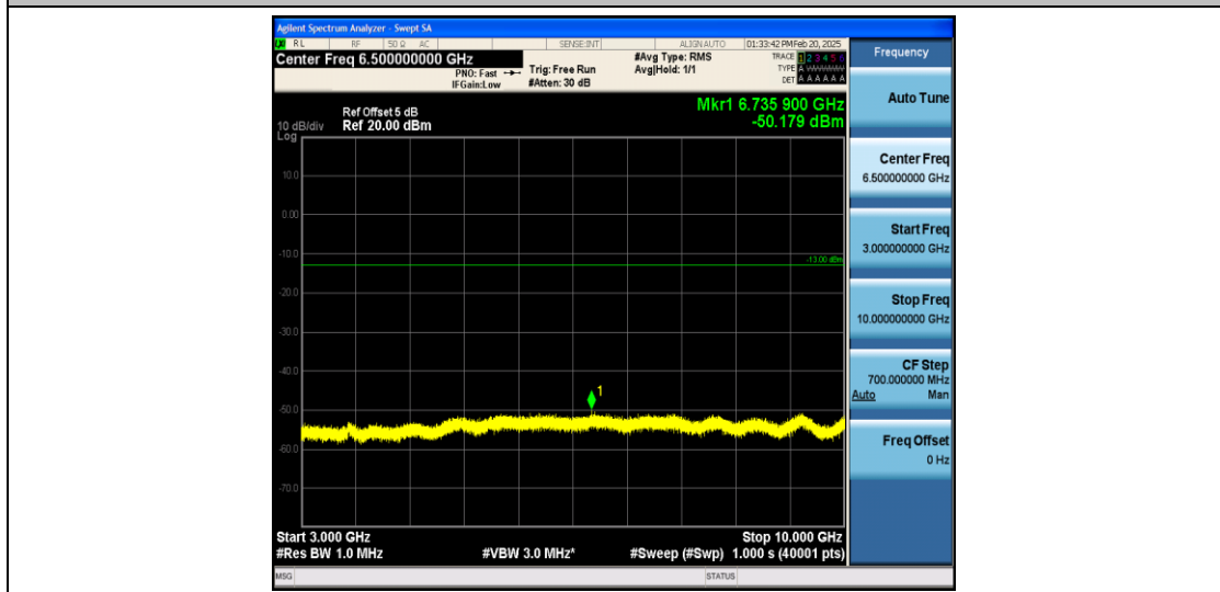
Band26_3MHz_QPSK_26915_1RB#0_3000~10000_3000~10000
