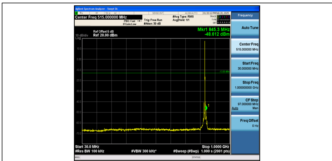
Band26_3MHz_QPSK_26915_1RB#0_30~1000_30~1000
