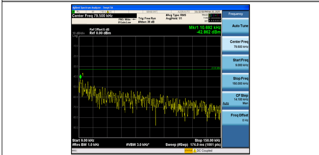
Band26_3MHz_QPSK_26915_1RB#0_0.009~0.15_0.009~0.15
