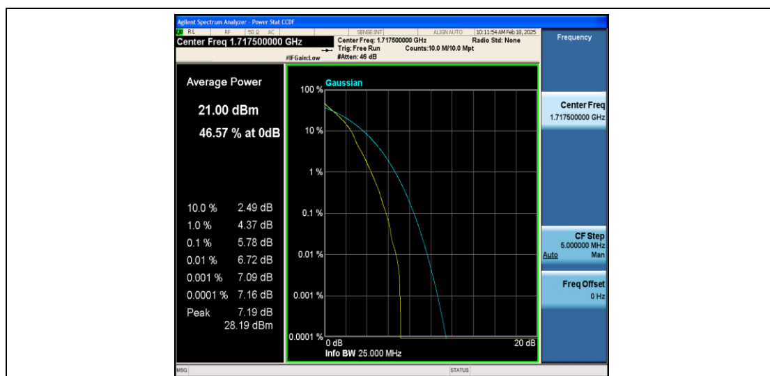
Band66-15MHz-QPSK-131047-1RB#0-PASS
