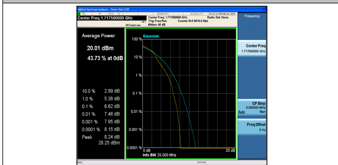
Band66-15MHz-16QAM-131047-1RB#0-PASS
