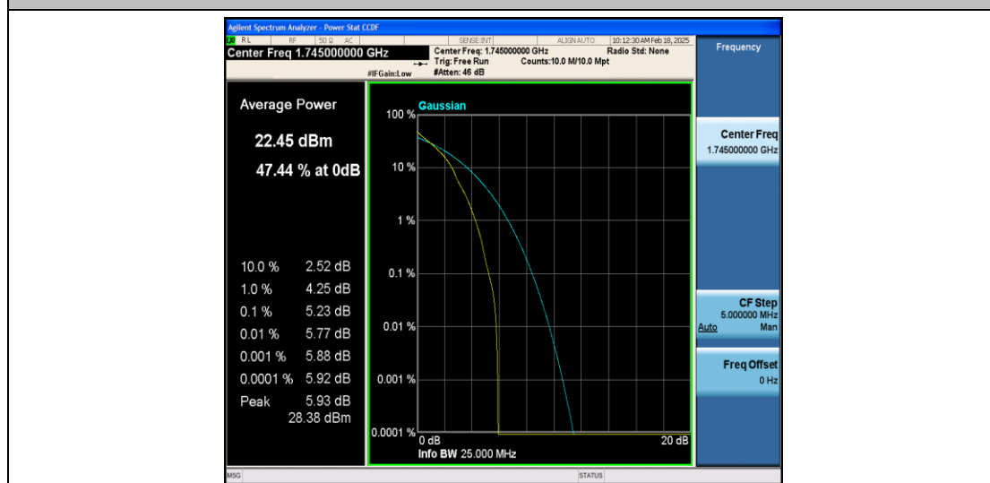
Band66-15MHz-QPSK-132322-1RB#0-PASS
