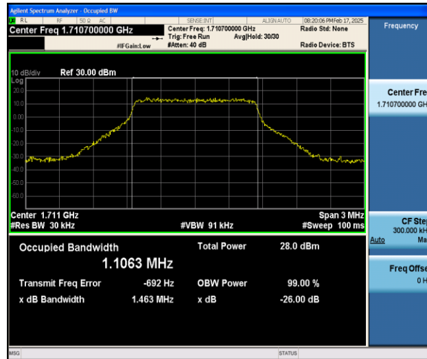
Band66-1.4MHz-QPSK-131979-6RB#0-PASS
