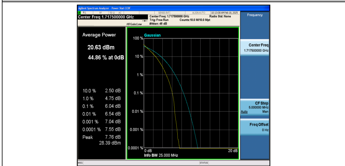
Band66-15MHz-QPSK-131047-75RB#0-PASS
