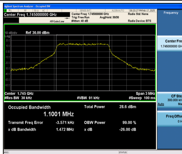
Band66-1.4MHz-QPSK-132322-6RB#0-PASS
