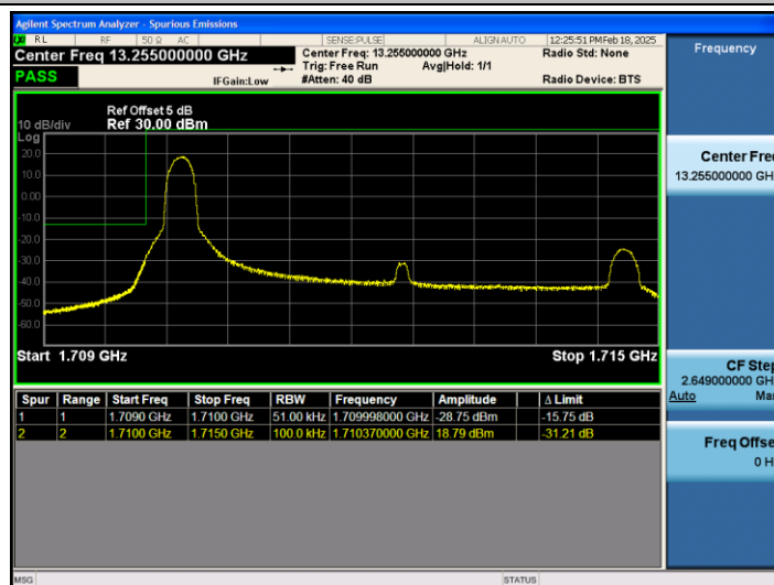
Band66_5MHz_16QAM_131997_1RB#0
