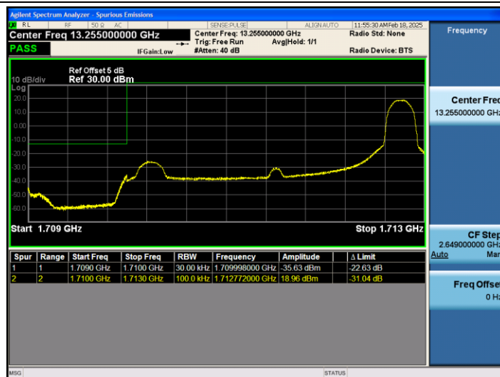
Band66_3MHz_16QAM_131987_1RB#14
