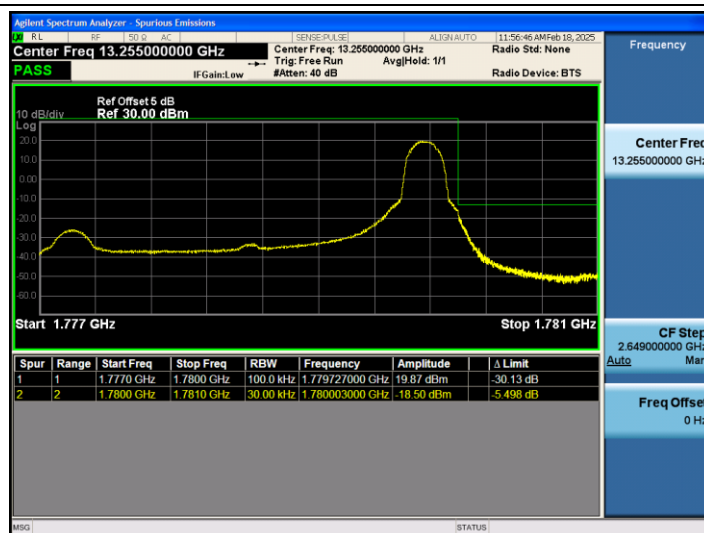
Band66_3MHz_16QAM_132657_1RB#14
