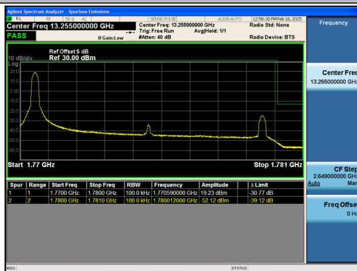
Band66_10MHz_QPSK_132622_1RB#0
