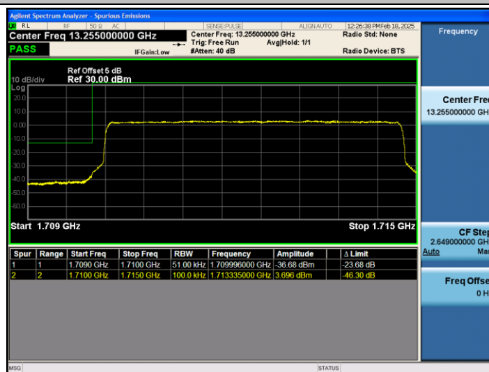
Band66_5MHz_16QAM_131997_25RB#0
