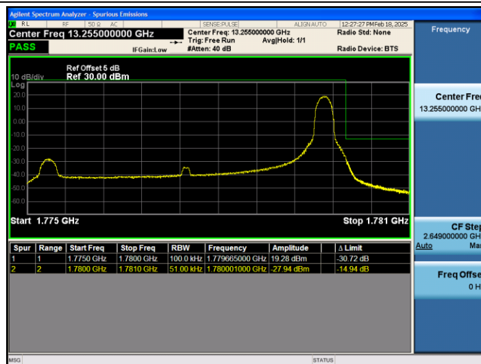
Band66_5MHz_16QAM_132647_1RB#24
