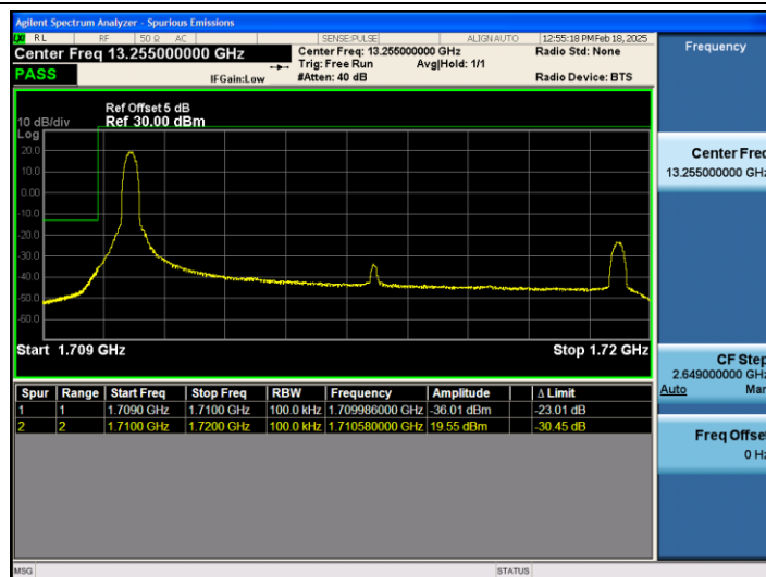
Band66_10MHz_QPSK_132022_1RB#0
