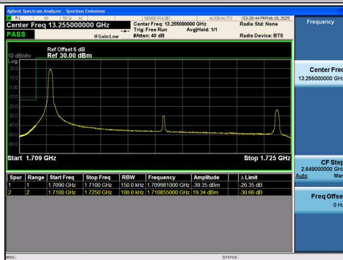
Band66_15MHz_16QAM_132047_1RB#0
