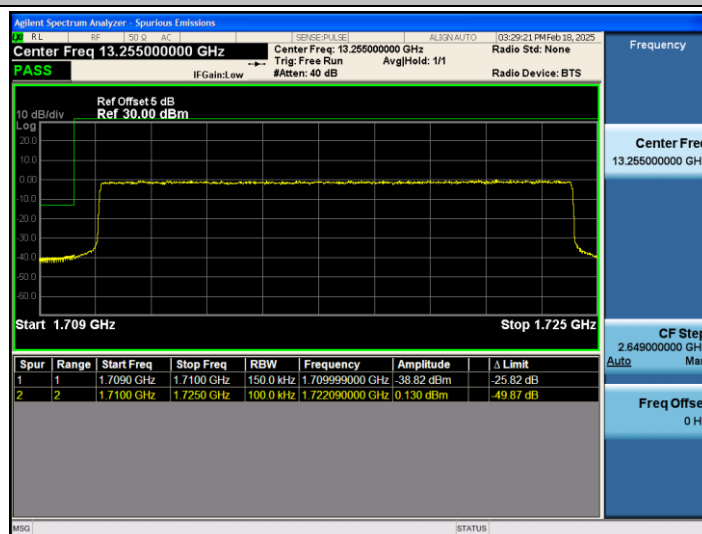
Band66_15MHz_QPSK_132047_75RB#0
