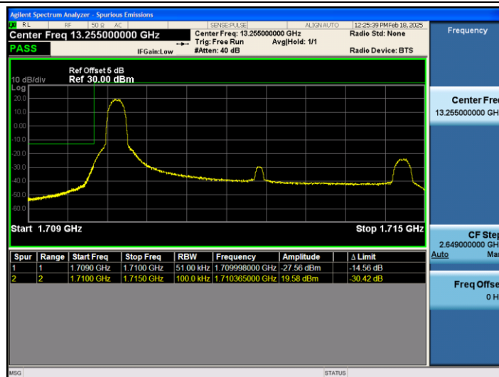
Band66_5MHz_QPSK_131997_1RB#0
