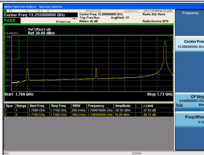
Band66_20MHz_16QAM_132072_1RB#99
