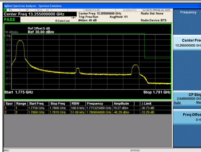
Band66_5MHz_QPSK_132647_1RB#0
