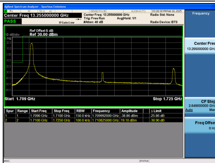
Band66_15MHz_QPSK_132047_1RB#0
