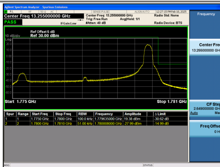
Band66_5MHz_QPSK_132647_1RB#24
