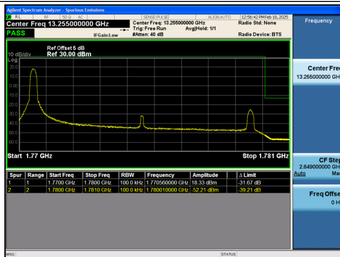
Band66_10MHz_16QAM_132622_1RB#0
