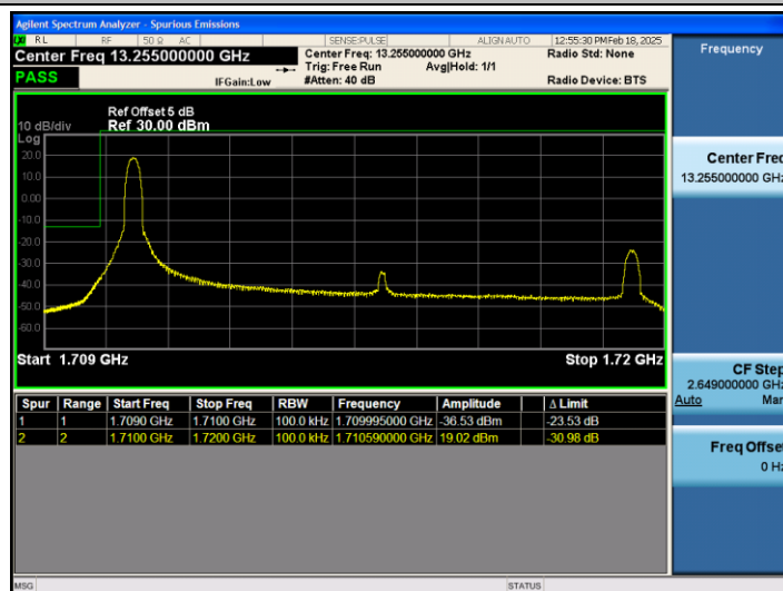
Band66_10MHz_16QAM_132022_1RB#0
