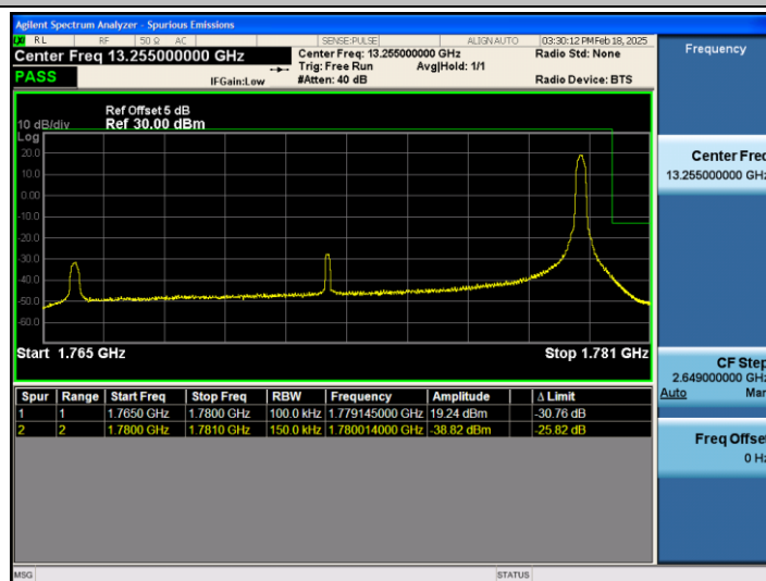
Band66_15MHz_QPSK_132597_1RB#74
