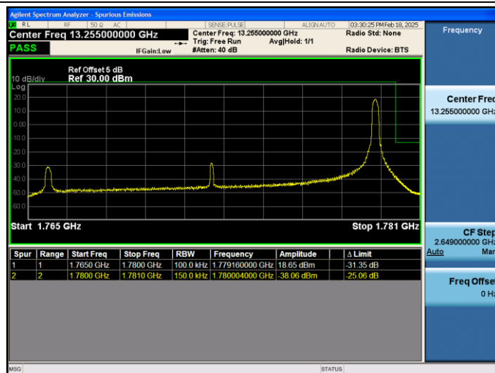
Band66_15MHz_16QAM_132597_1RB#74
