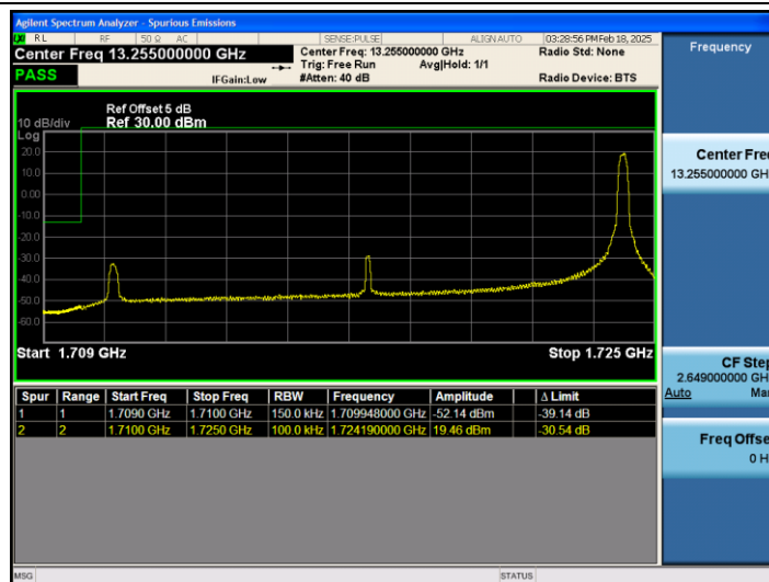
Band66_15MHz_QPSK_132047_1RB#74
