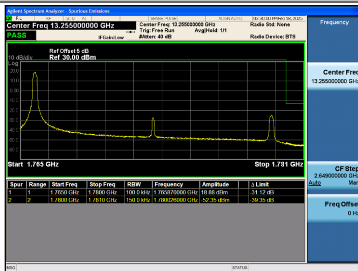
Band66_15MHz_16QAM_132597_1RB#0
