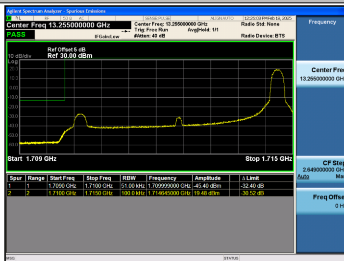
Band66_5MHz_QPSK_131997_1RB#24
