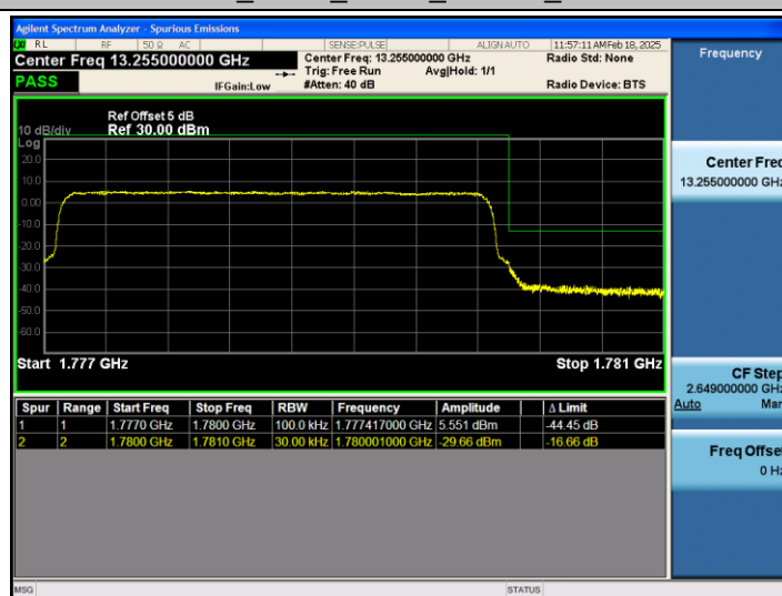
Band66_3MHz_16QAM_132657_15RB#0
