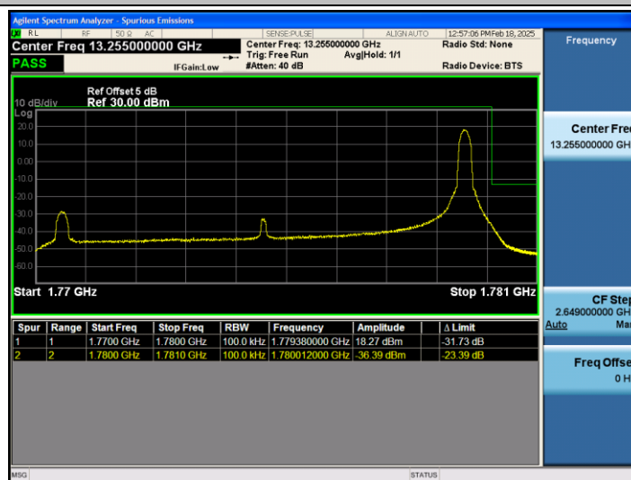
Band66_10MHz_16QAM_132622_1RB#49
