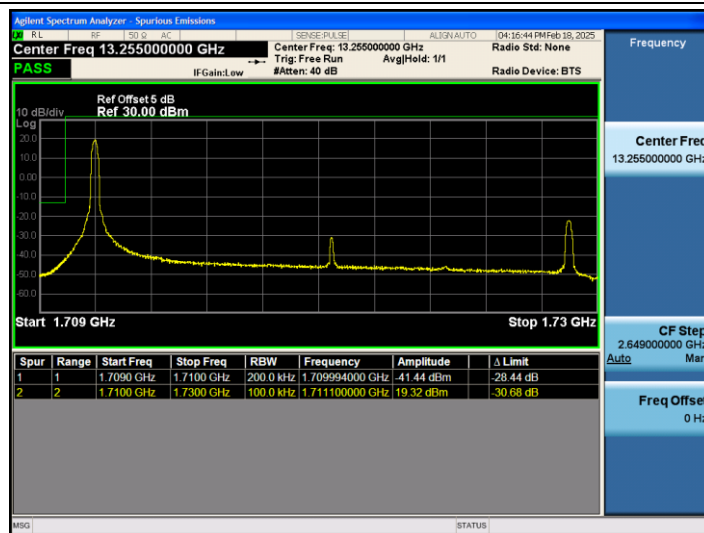
Band66_20MHz_16QAM_132072_1RB#0
