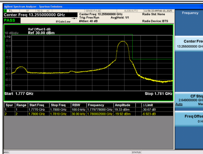
Band66_3MHz_QPSK_132657_1RB#14
