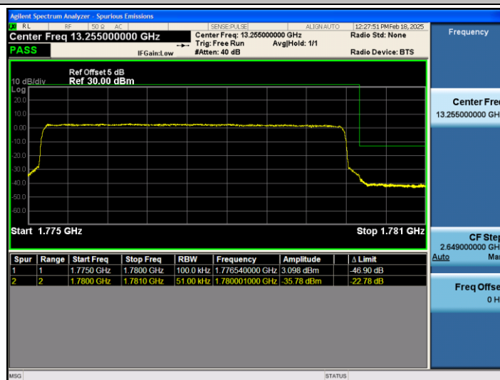
Band66_5MHz_16QAM_132647_25RB#0
