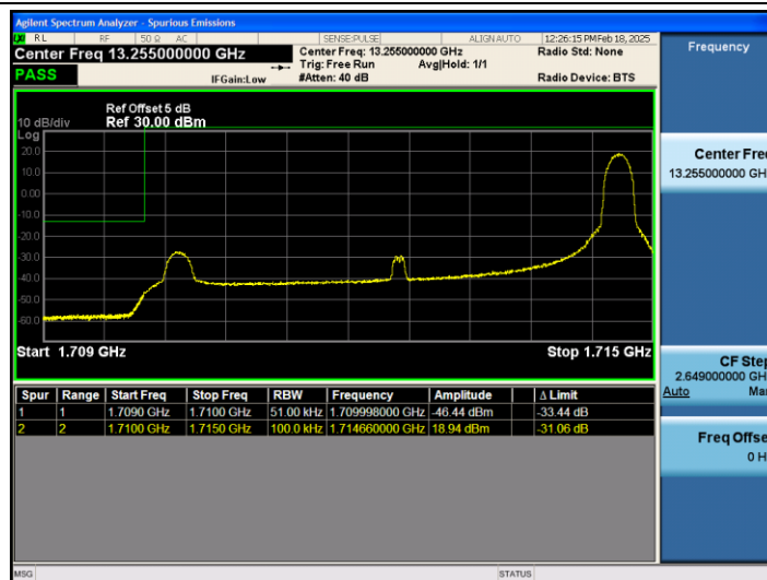
Band66_5MHz_16QAM_131997_1RB#24
