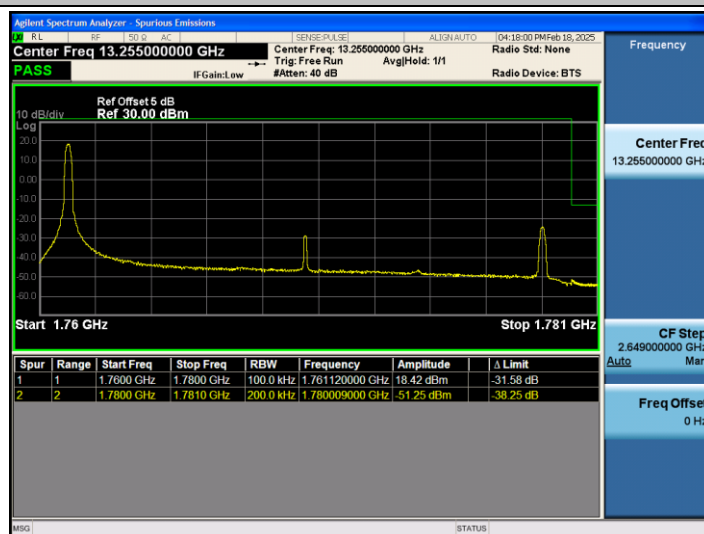
Band66_20MHz_16QAM_132572_1RB#0
