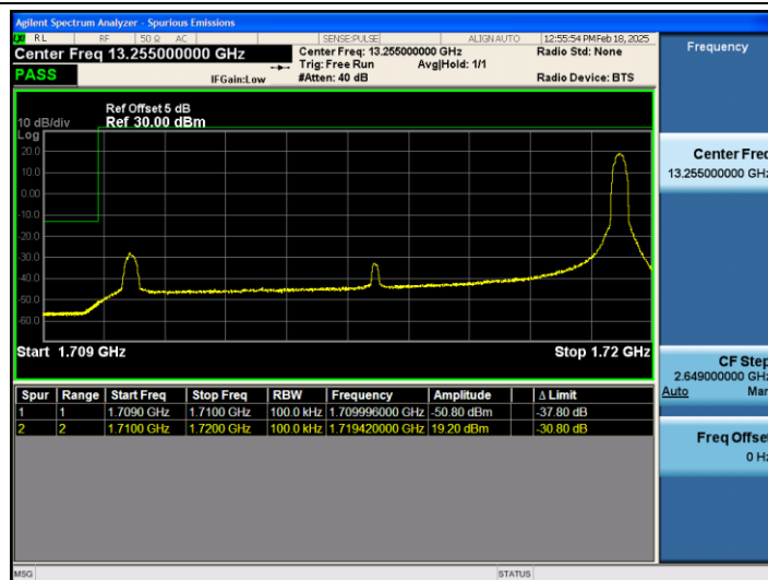
Band66_10MHz_16QAM_132022_1RB#49
