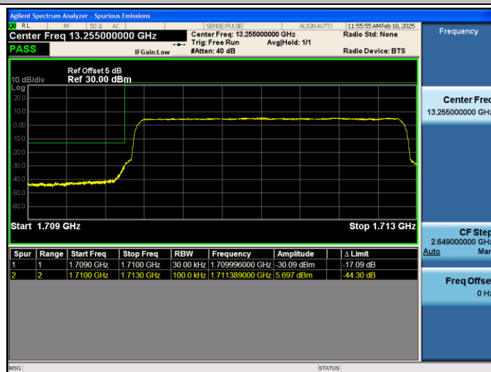
Band66_3MHz_16QAM_131987_15RB#0
