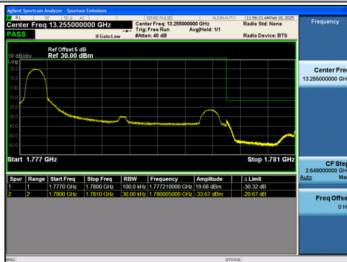
Band66_3MHz_16QAM_132657_1RB#0
