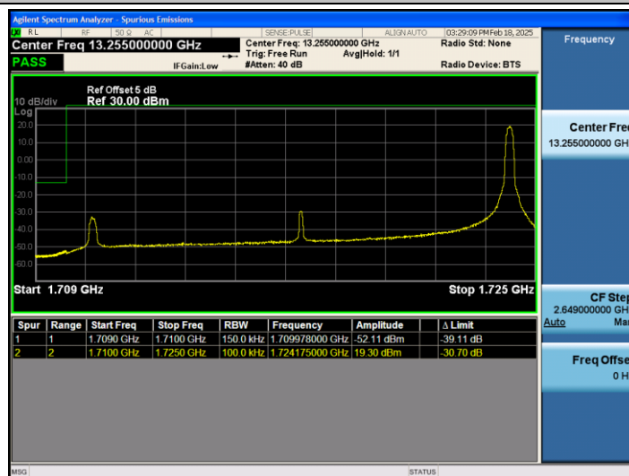
Band66_15MHz_16QAM_132047_1RB#74
