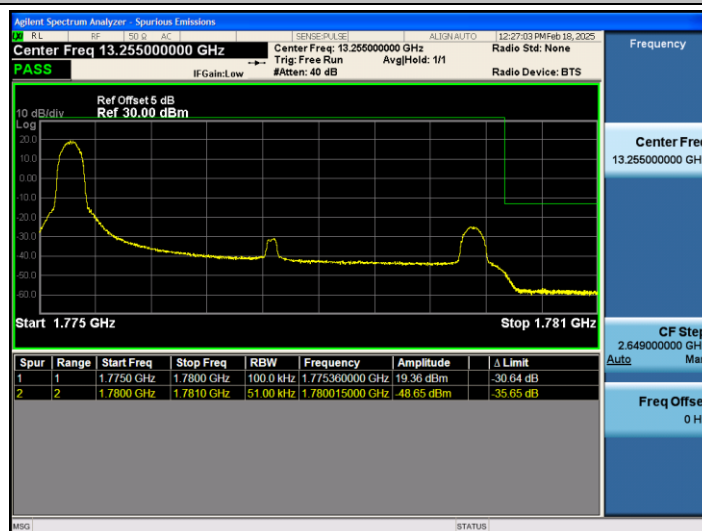
Band66_5MHz_16QAM_132647_1RB#0
