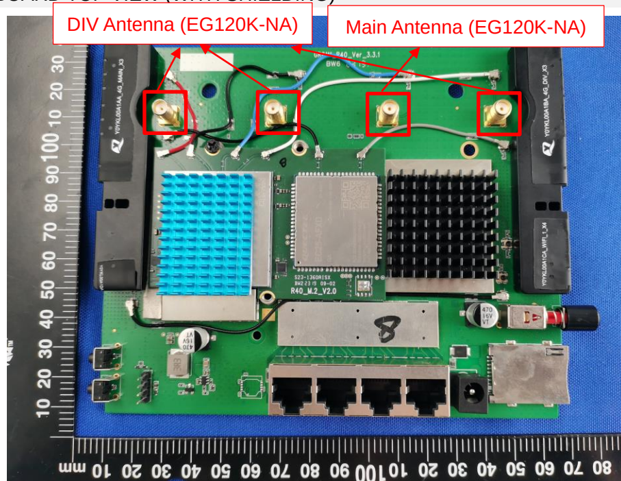
MAIN BOARD TOP VIEW (WITH SHIELDING)
