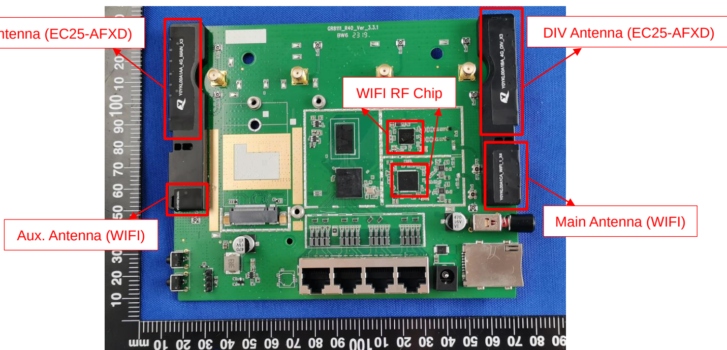
MAIN BOARD TOP VIEW (WITHOUT SHIELDING)
