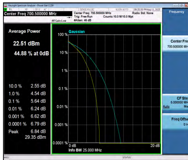
Band12-3MHz-QPSK-23025-15RB#0-PASS
