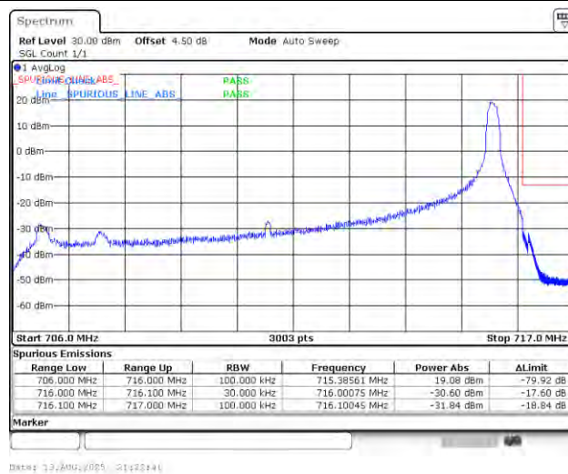
Band12_10MHz_16QAM_23130_1RB#49
