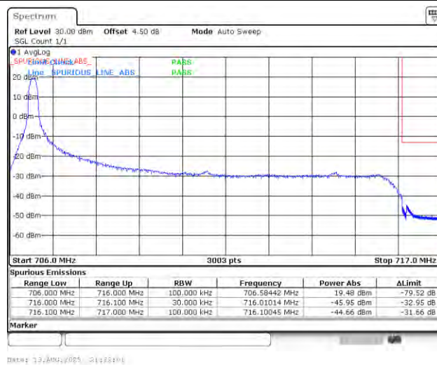
Band12_10MHz_QPSK_23130_1RB#0
