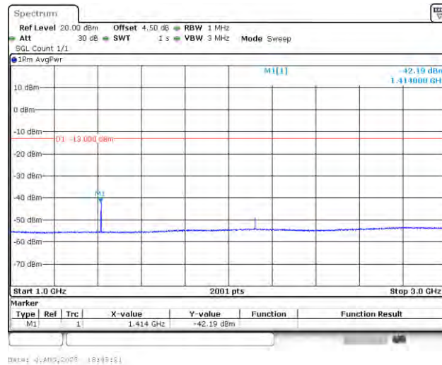
Band12_1.4MHz_16QAM_23095_1RB#0_1000~3000_1000~3000
