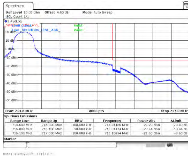
Band12_1.4MHz_QPSK_23173_1RB#0
