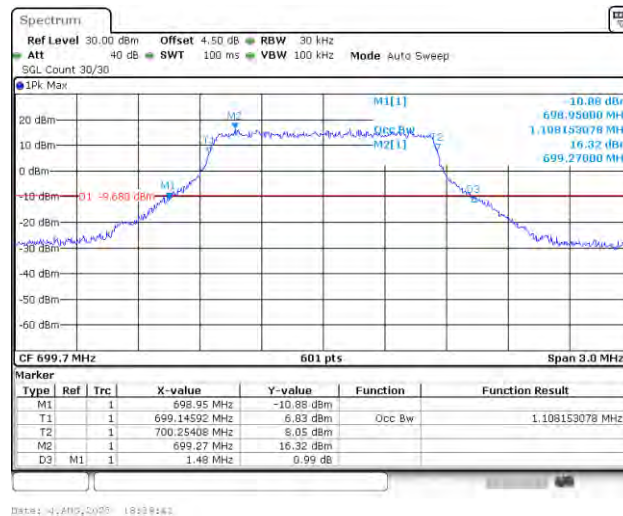
Band12-1.4MHz-QPSK-23017-6RB#0-PASS
