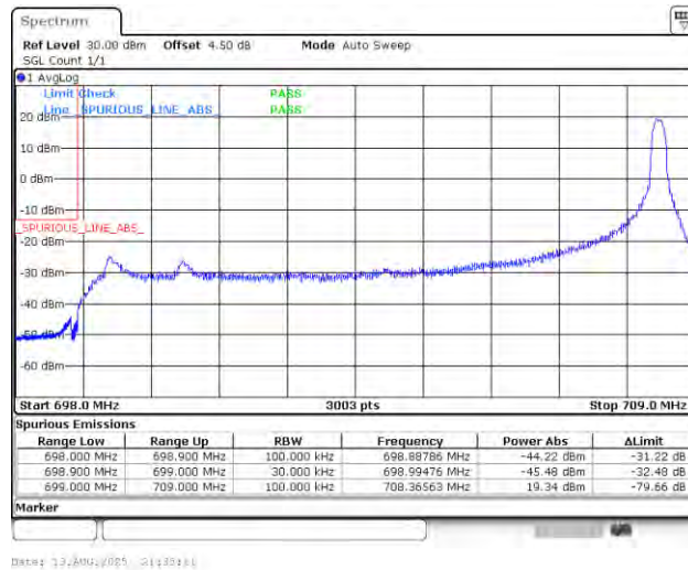
Band12_10MHz_16QAM_23060_1RB#49
