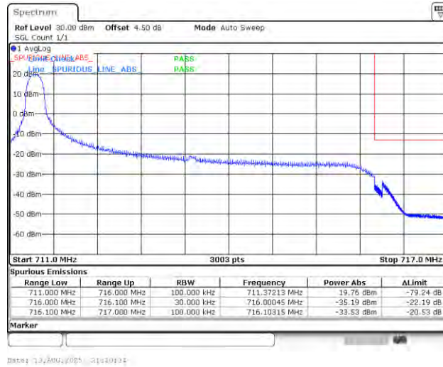
Band12_5MHz_QPSK_23155_1RB#0
