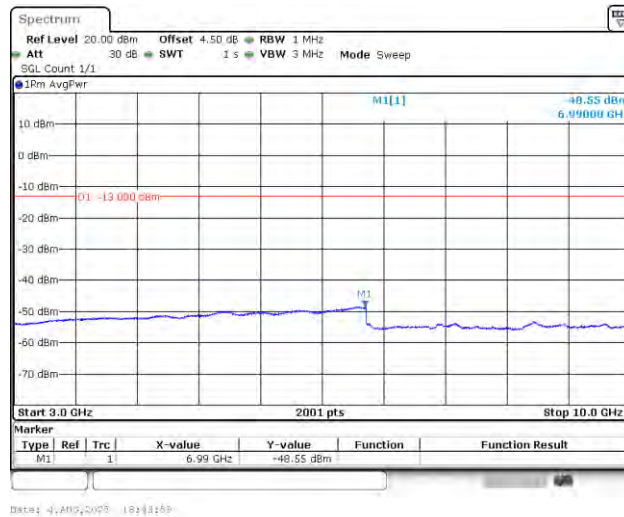
Band12_1.4MHz_QPSK_23017_1RB#0_3000~10000_3000~10000
