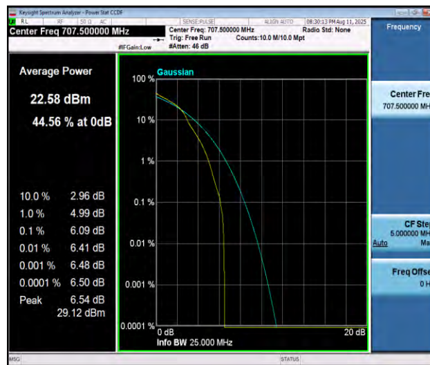
Band12-10MHz-16QAM-23095-1RB#0-PASS
