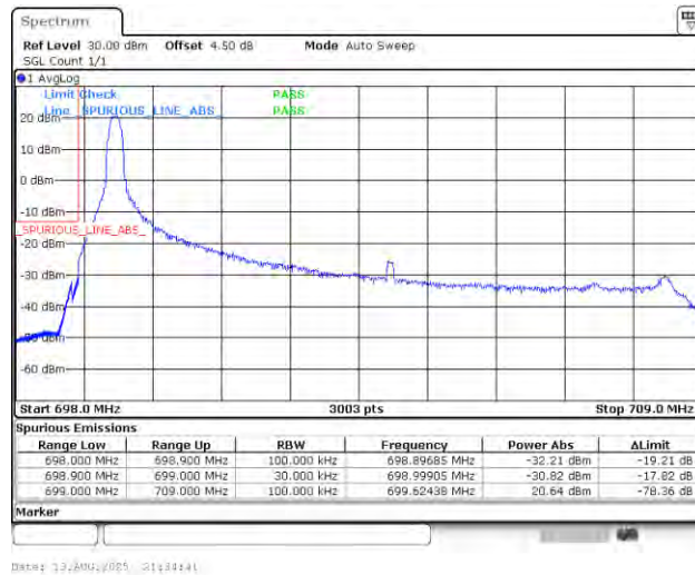
Band12_10MHz_QPSK_23060_1RB#0
