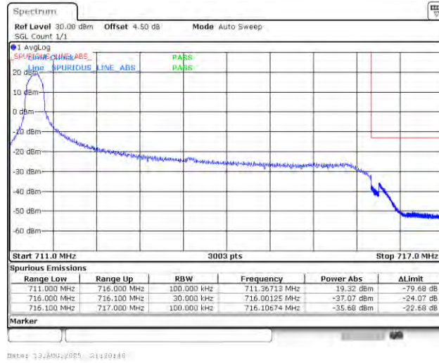
Band12_5MHz_16QAM_23155_1RB#0
