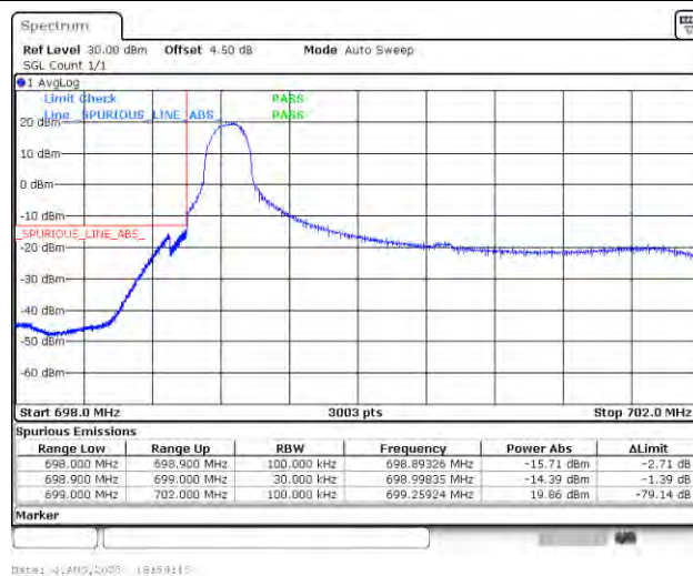
Band12_3MHz_16QAM_23025_1RB#0
