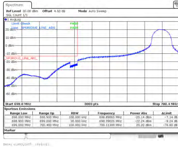
Band12_1.4MHz_QPSK_23017_1RB#5
