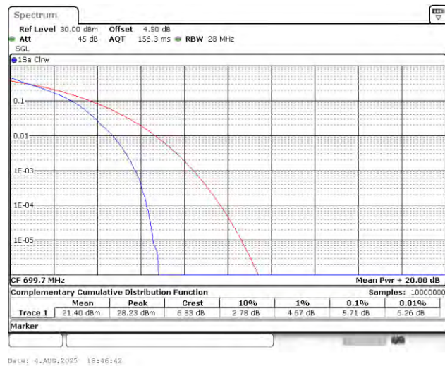
Band12-1.4MHz-QPSK-23017-6RB#0-PASS
