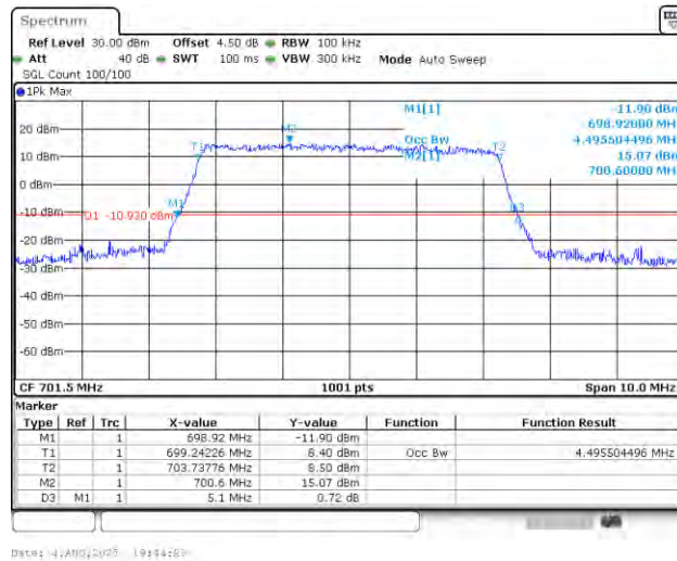
Band12-5MHz-16QAM-23035-25RB#0-PASS
