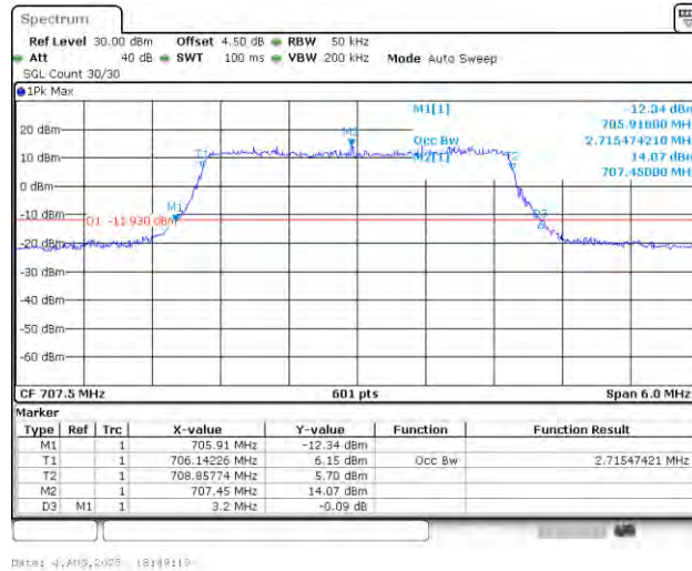
Band12-3MHz-16QAM-23095-15RB#0-PASS
