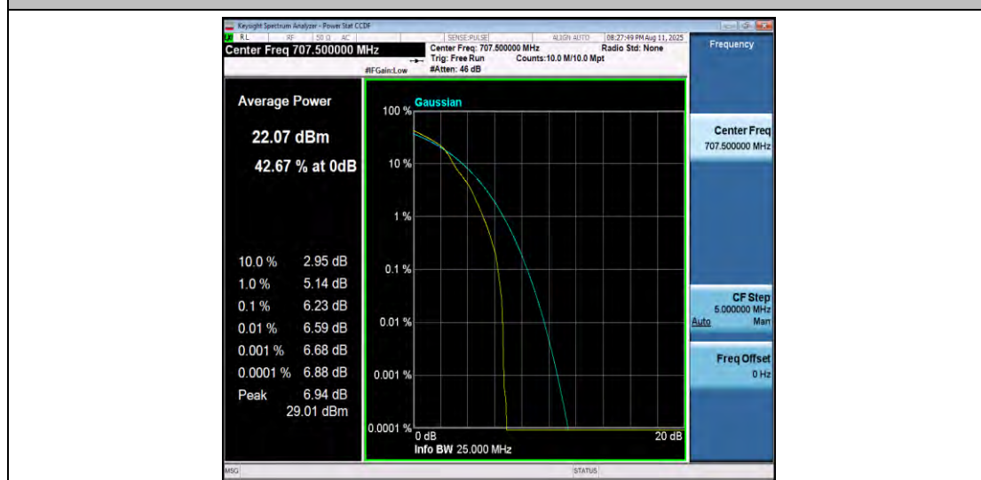
Band12-5MHz-16QAM-23095-1RB#0-PASS
