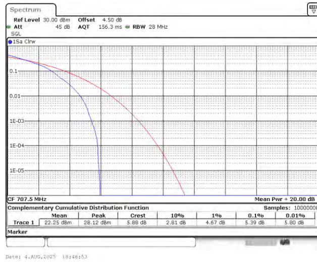
Band12-1.4MHz-QPSK-23095-1RB#0-PASS
