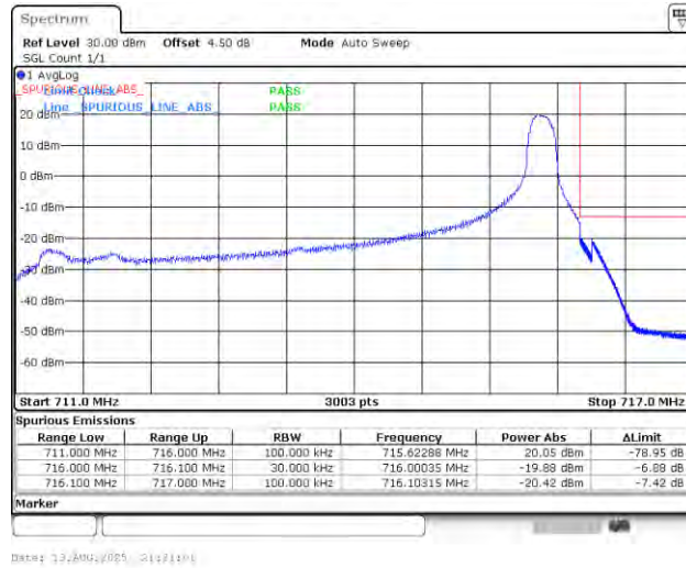
Band12_5MHz_QPSK_23155_1RB#24
