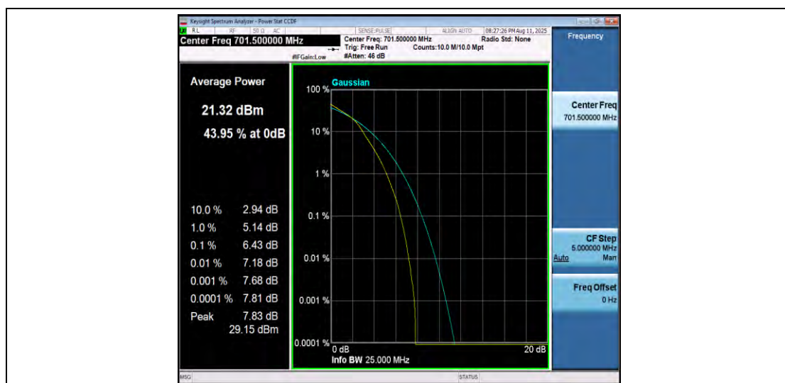
Band12-5MHz-16QAM-23035-25RB#0-PASS
