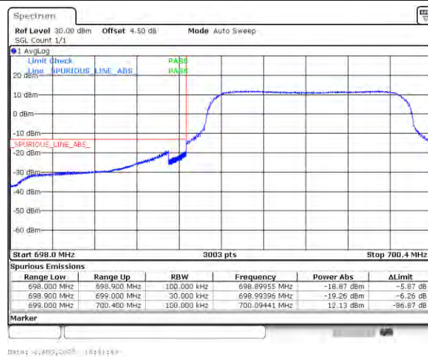
Band12_1.4MHz_QPSK_23017_6RB#0
