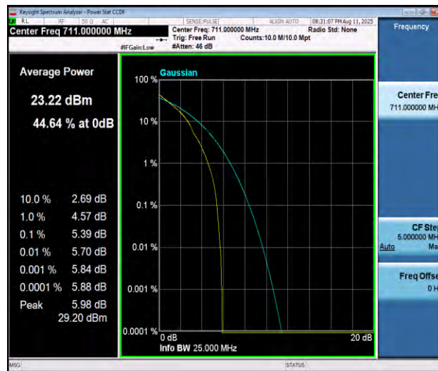
Band12-10MHz-QPSK-23130-1RB#0-PASS
