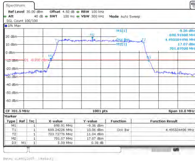
Band12-5MHz-QPSK-23035-25RB#0-PASS
