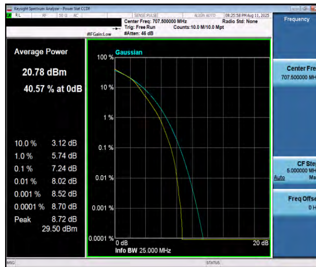
Band12-3MHz-16QAM-23095-15RB#0-PASS
