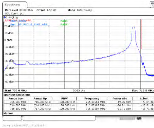
Band12_10MHz_QPSK_23130_1RB#49
