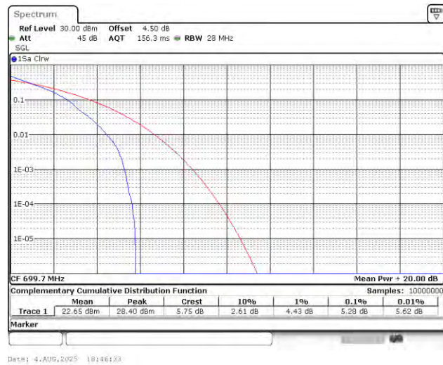
Band12-1.4MHz-QPSK-23017-1RB#0-PASS
