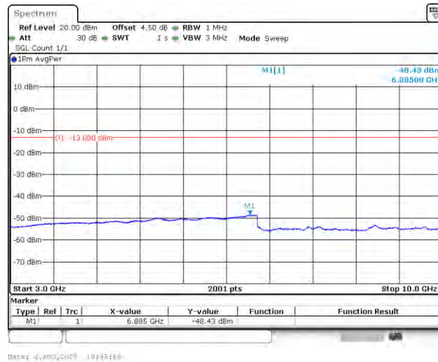
Band12_1.4MHz_16QAM_23095_1RB#0_3000~10000_3000~10000
