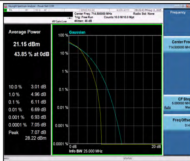
Band12-3MHz-16QAM-23165-15RB#0-PASS
