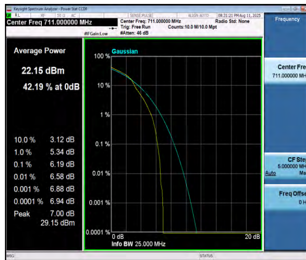
Band12-10MHz-16QAM-23130-1RB#0-PASS
