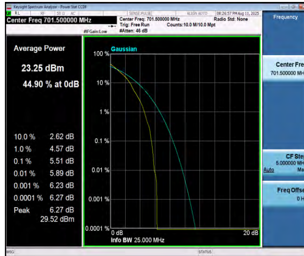
Band12-5MHz-QPSK-23035-1RB#0-PASS
