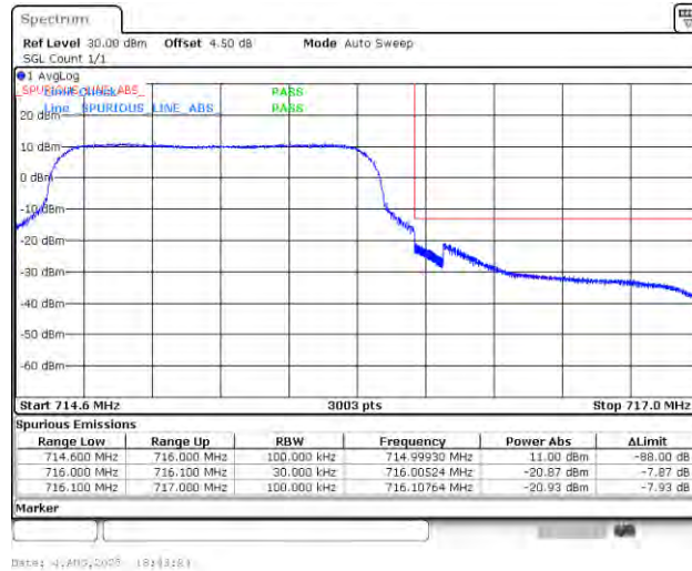
Band12_1.4MHz_16QAM_23173_6RB#0
