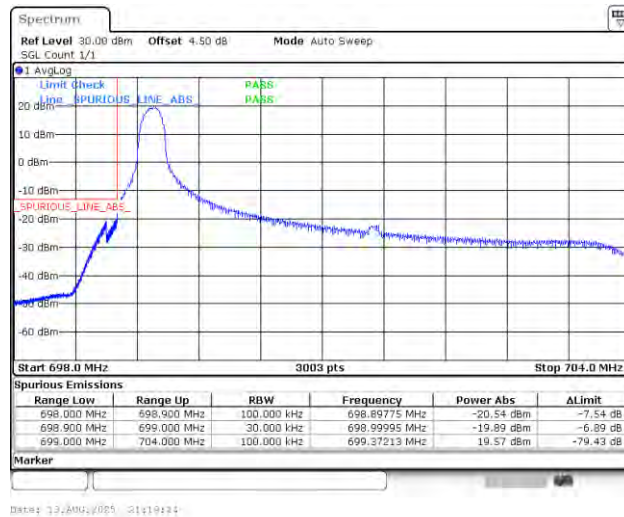
Band12_5MHz_16QAM_23035_1RB#0
