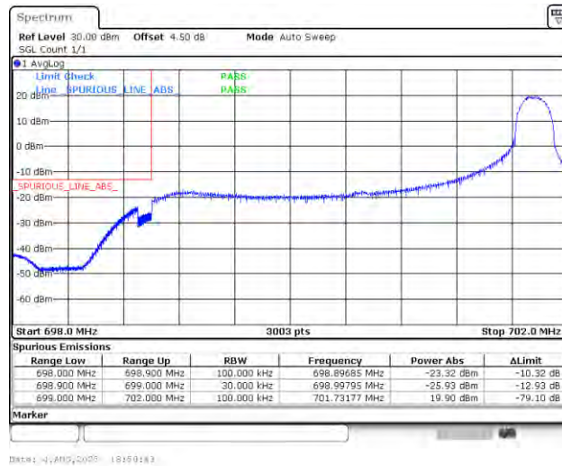
Band12_3MHz_16QAM_23025_1RB#14
