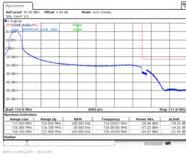
Band12_3MHz_QPSK_23165_1RB#0
