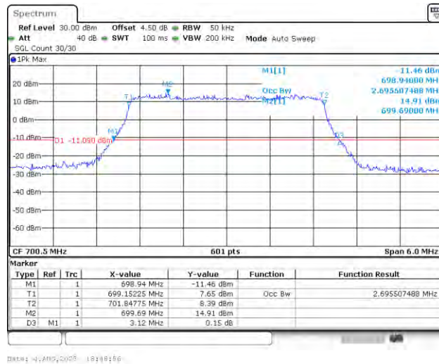
Band12-3MHz-16QAM-23025-15RB#0-PASS
