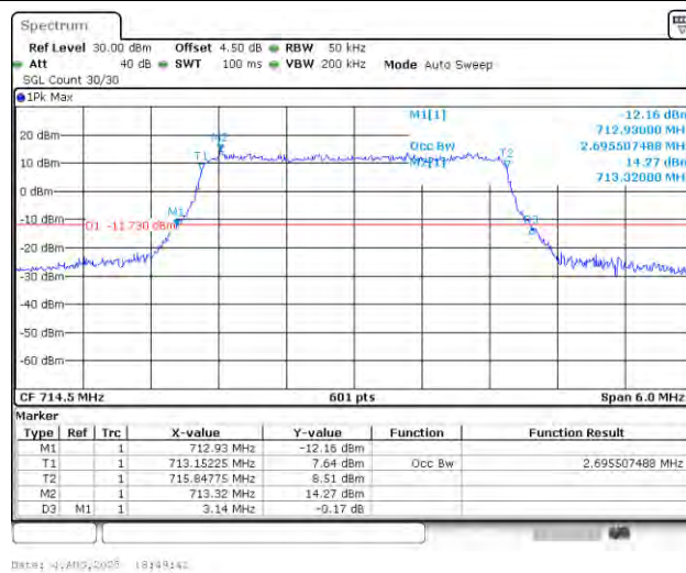
Band12-3MHz-16QAM-23165-15RB#0-PASS
