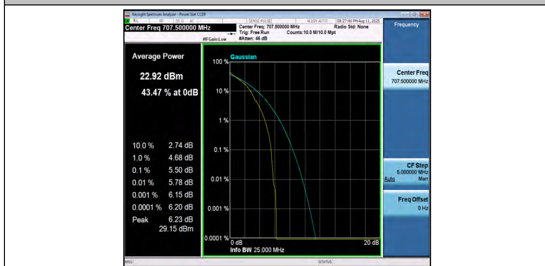
Band12-5MHz-QPSK-23095-1RB#0-PASS
