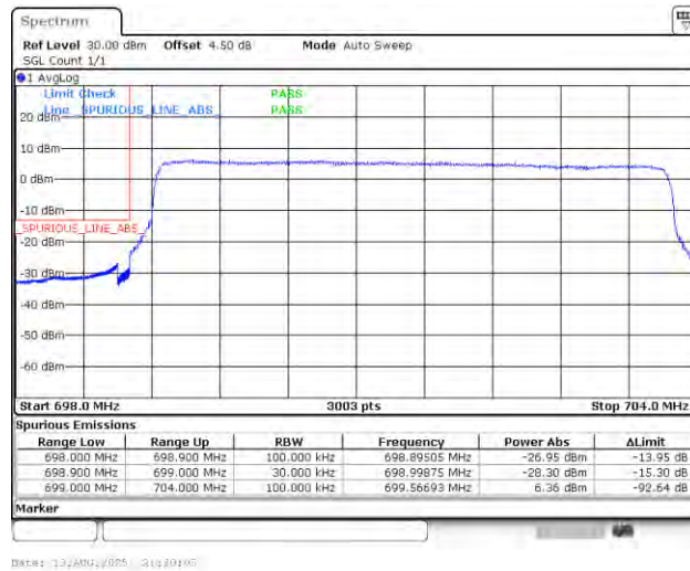
Band12_5MHz_QPSK_23035_25RB#0
