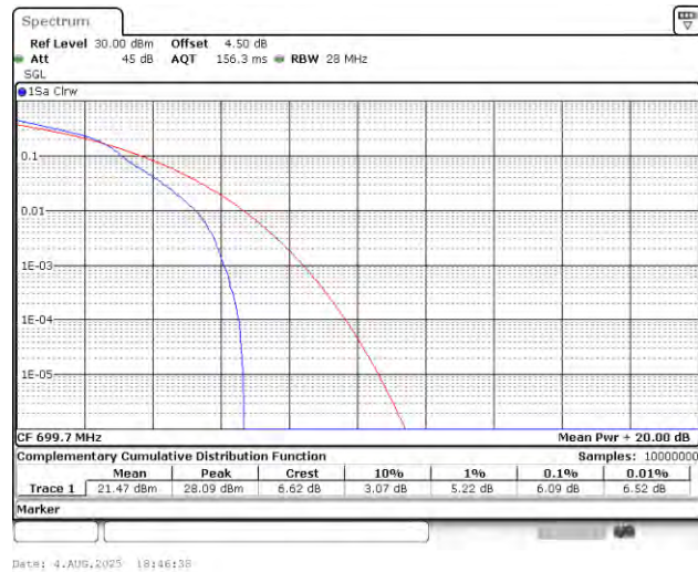
Band12-1.4MHz-16QAM-23017-1RB#0-PASS
