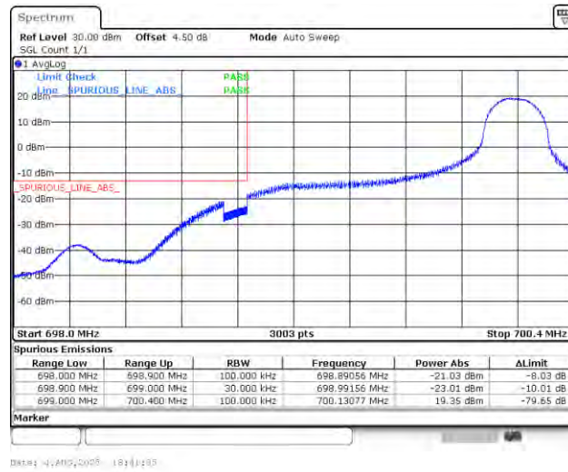
Band12_1.4MHz_16QAM_23017_1RB#5
