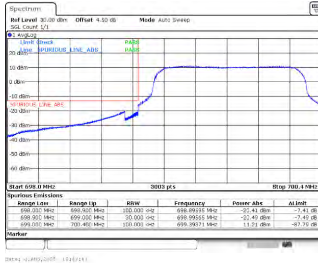
Band12_1.4MHz_16QAM_23017_6RB#0
