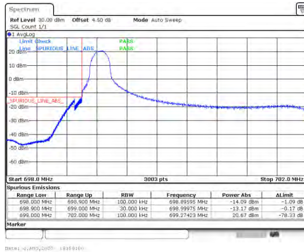
Band12_3MHz_QPSK_23025_1RB#0
