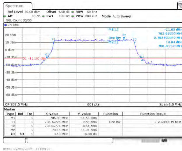
Band12-3MHz-QPSK-23095-15RB#0-PASS
