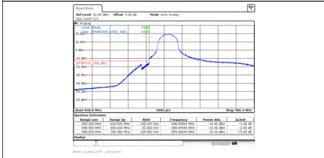
Band12_1.4MHz_16QAM_23017_1RB#0
