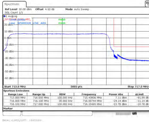
Band12_3MHz_16QAM_23165_15RB#0
