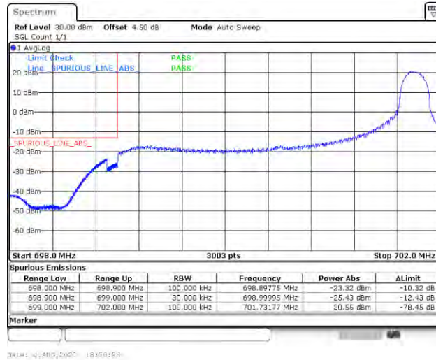
Band12_3MHz_QPSK_23025_1RB#14
