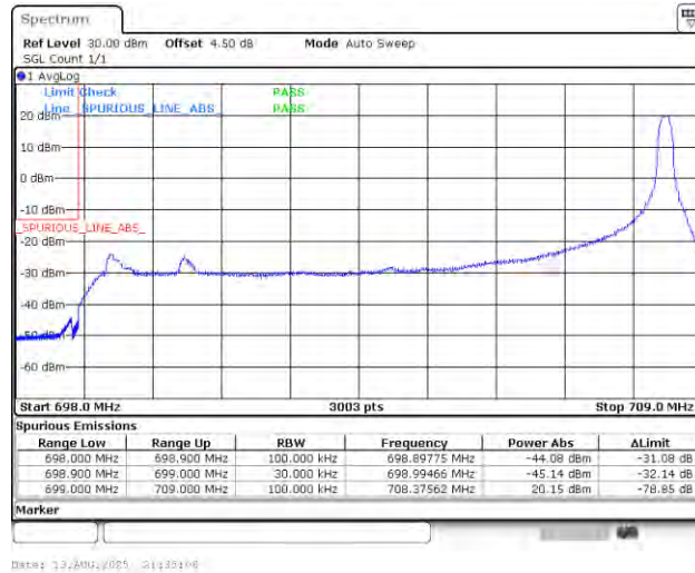
Band12_10MHz_QPSK_23060_1RB#49
