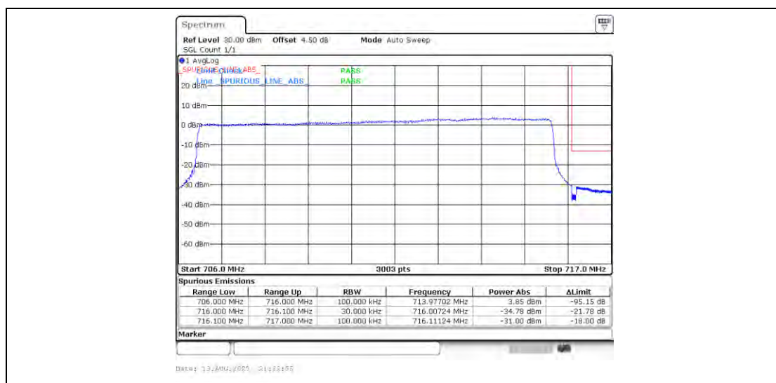
Band12_10MHz_QPSK_23130_50RB#0
