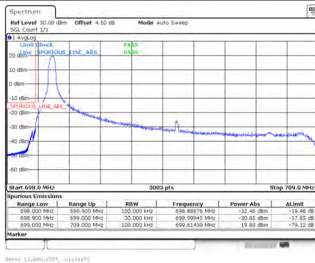
Band12_10MHz_16QAM_23060_1RB#0
