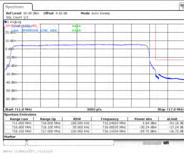
Band12_5MHz_QPSK_23155_25RB#0
