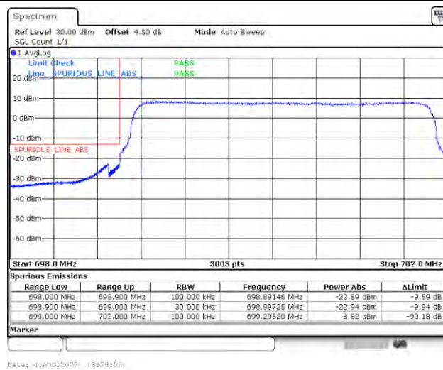
Band12_3MHz_QPSK_23025_15RB#0
