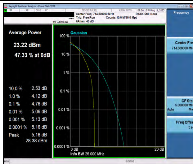
Band12-3MHz-QPSK-23165-1RB#0-PASS
