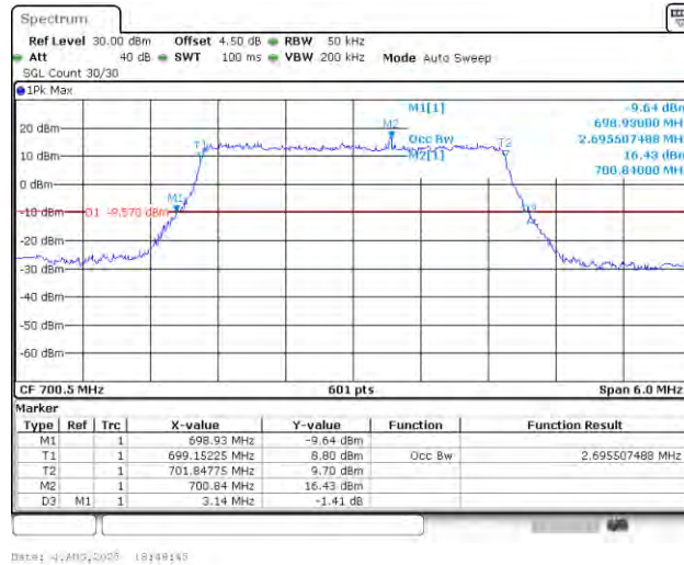
Band12-3MHz-QPSK-23025-15RB#0-PASS
