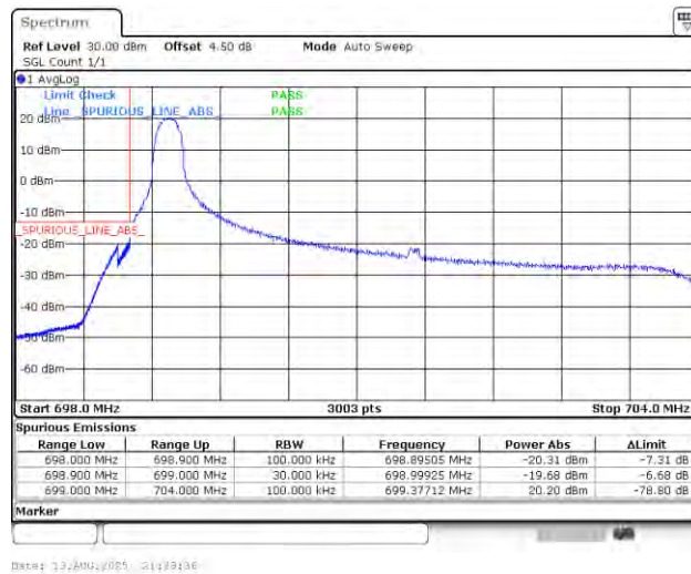
Band12_5MHz_QPSK_23035_1RB#0
