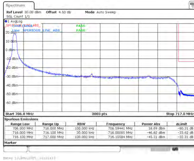
Band12_10MHz_16QAM_23130_1RB#0
