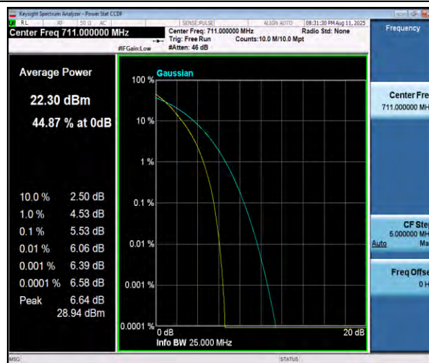
Band12-10MHz-QPSK-23130-50RB#0-PASS
