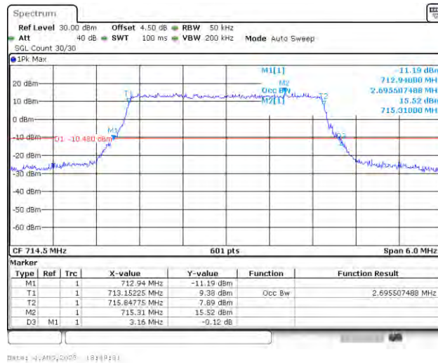
Band12-3MHz-QPSK-23165-15RB#0-PASS
