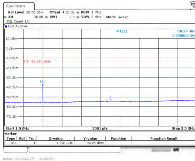
Band12_1.4MHz_QPSK_23017_1RB#0_1000~3000_1000~3000
