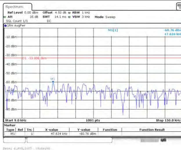
Band12_1.4MHz_16QAM_23017_1RB#0_0.009~0.15_0.009~0.15
