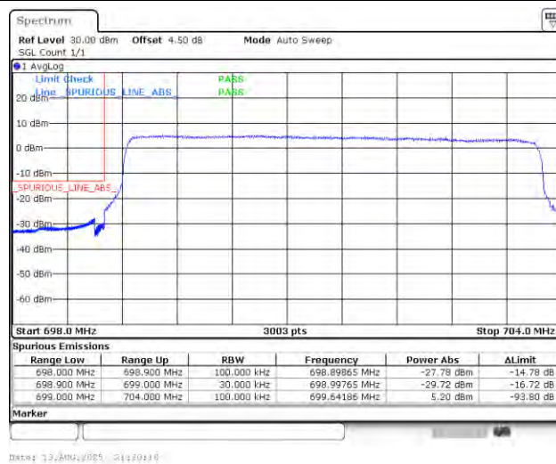
Band12_5MHz_16QAM_23035_25RB#0
