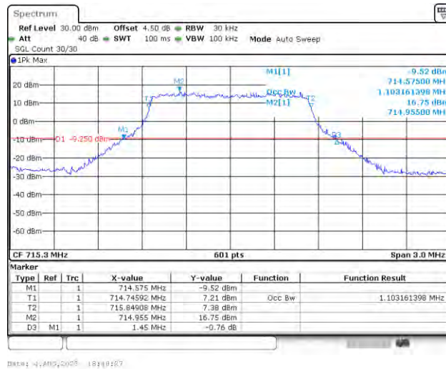
Band12-1.4MHz-QPSK-23173-6RB#0-PASS
