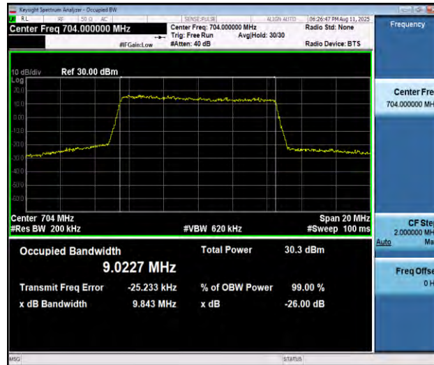
Band12-10MHz-QPSK-23060-50RB#0-PASS
