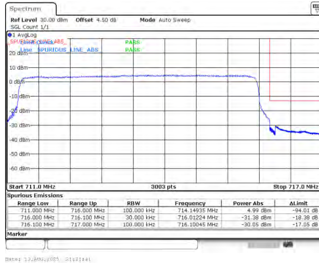
Band12_5MHz_16QAM_23155_25RB#0
