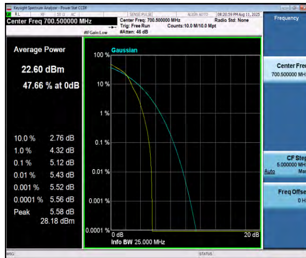
Band12-3MHz-16QAM-23025-1RB#0-PASS
