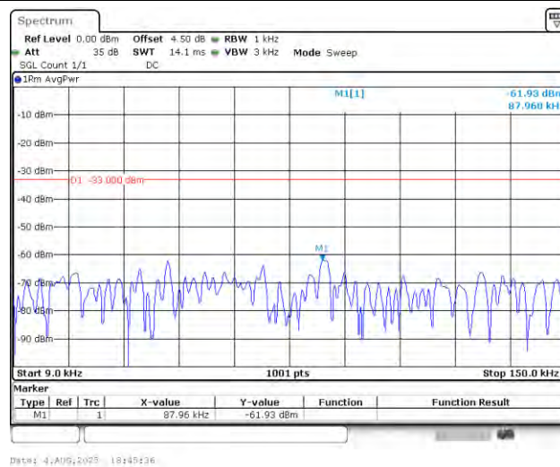
Band12_1.4MHz_QPSK_23173_1RB#0_0.009~0.15_0.009~0.15
