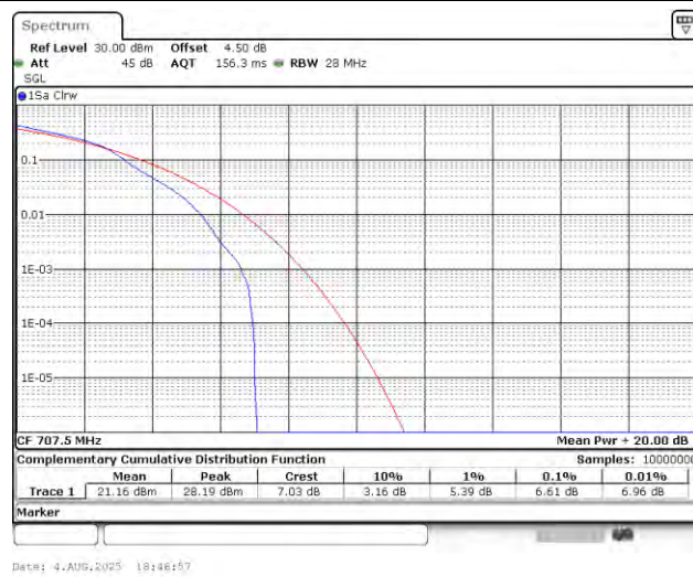
Band12-1.4MHz-16QAM-23095-1RB#0-PASS
