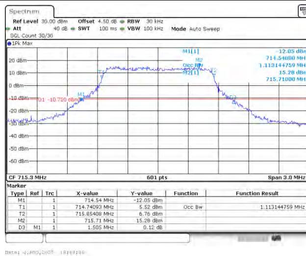
Band12-1.4MHz-16QAM-23173-6RB#0-PASS
