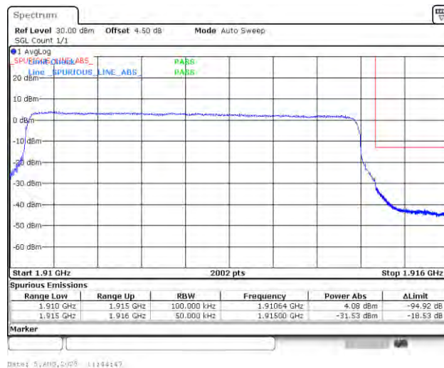
Band25_5MHz_16QAM_26665_25RB#0
