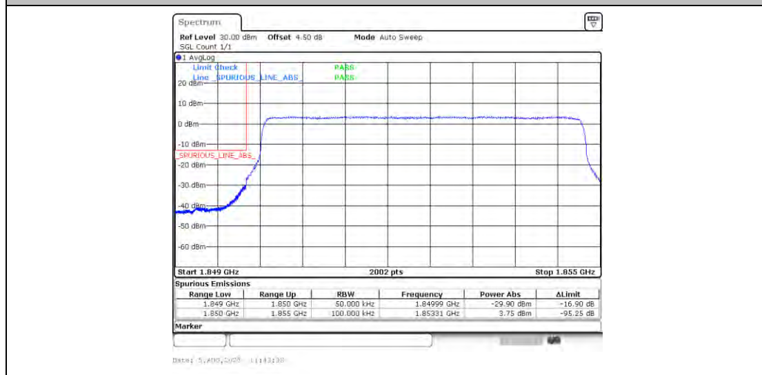
Band25_5MHz_16QAM_26065_25RB#0
