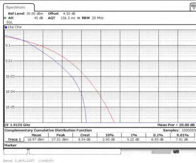
Band25-5MHz-16QAM-26665-25RB#0-PASS
