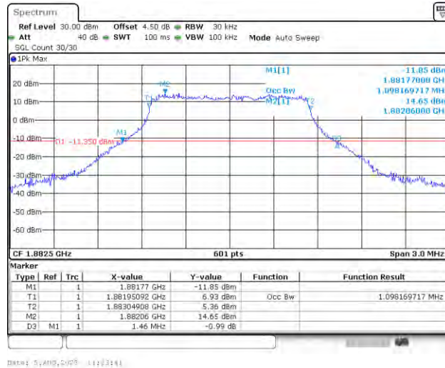
Band25-1.4MHz-16QAM-26365-6RB#0-PASS
