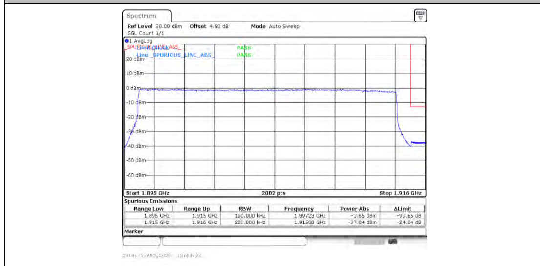
Band25_20MHz_QPSK_26590_100RB#0
