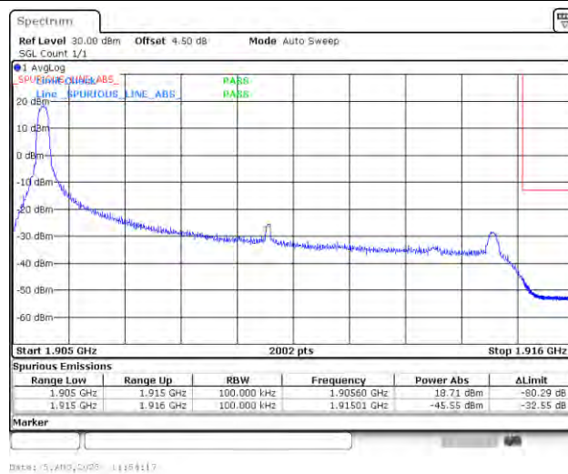
Band25_10MHz_16QAM_26640_1RB#0
