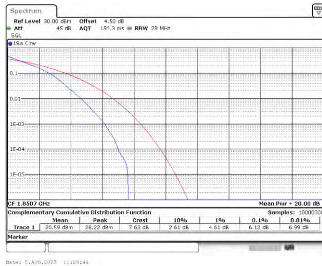
Band25-1.4MHz-QPSK-26047-6RB#0-PASS
