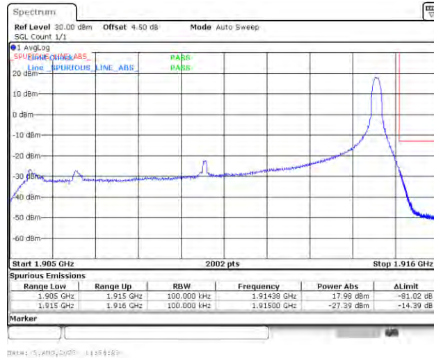
Band25_10MHz_QPSK_26640_1RB#49
