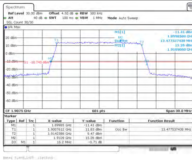
Band25-15MHz-QPSK-26615-75RB#0-PASS
