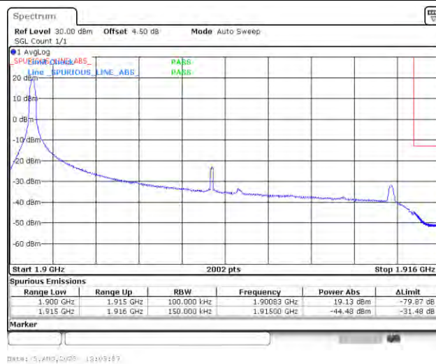
Band25_15MHz_QPSK_26615_1RB#0
