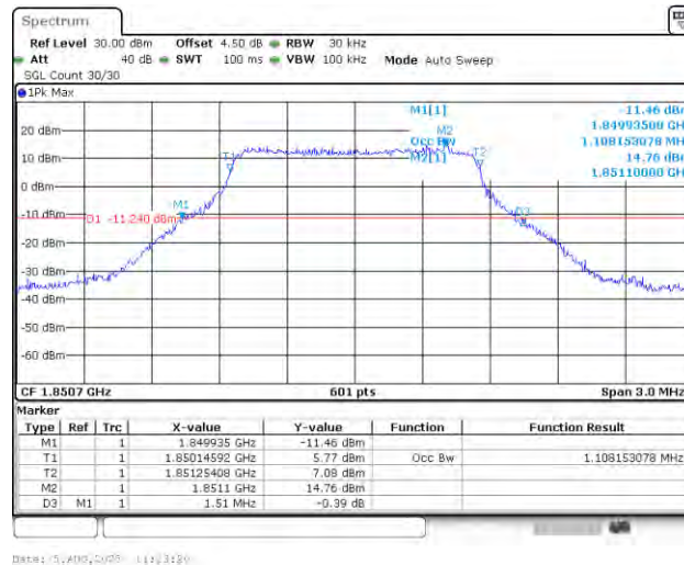
Band25-1.4MHz-16QAM-26047-6RB#0-PASS
