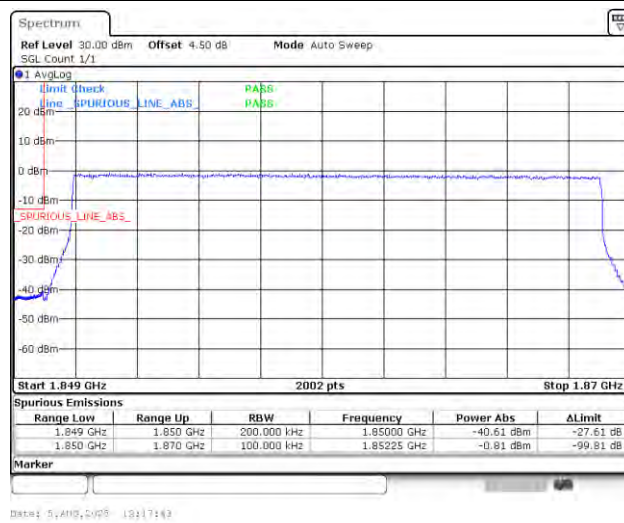
Band25_20MHz_QPSK_26140_100RB#0
