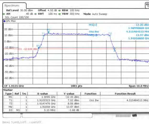
Band25-5MHz-16QAM-26665-25RB#0-PASS
