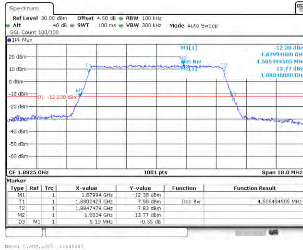
Band25-5MHz-16QAM-26365-25RB#0-PASS
