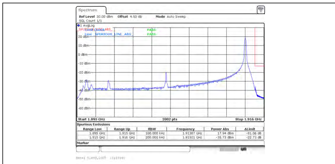
Band25_20MHz_16QAM_26590_1RB#99
