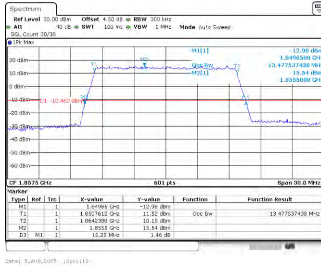
Band25-15MHz-QPSK-26115-75RB#0-PASS
