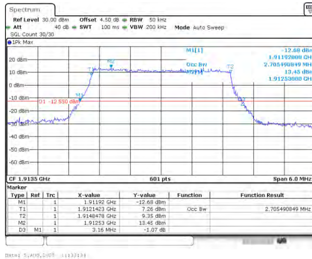
Band25-3MHz-QPSK-26675-15RB#0-PASS
