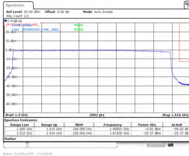
Band25_15MHz_QPSK_26615_75RB#0
