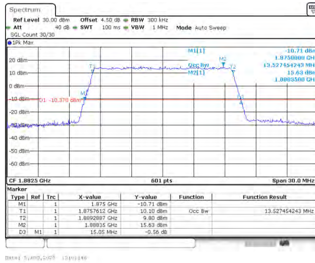
Band25-15MHz-QPSK-26365-75RB#0-PASS
