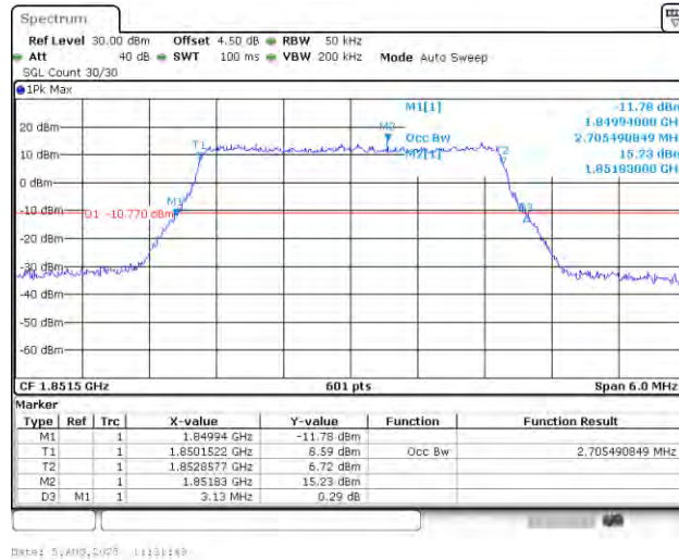
Band25-3MHz-QPSK-26055-15RB#0-PASS
