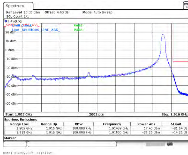
Band25_10MHz_16QAM_26640_1RB#49
