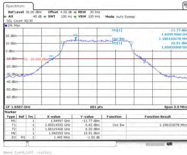
Band25-1.4MHz-QPSK-26047-6RB#0-PASS
