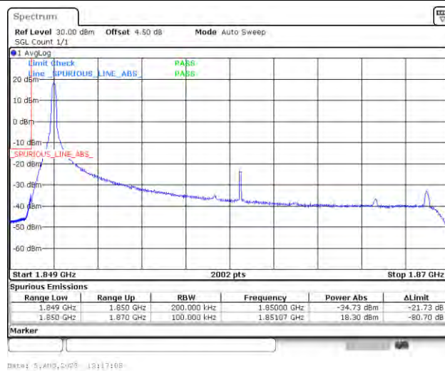
Band25_20MHz_16QAM_26140_1RB#0
