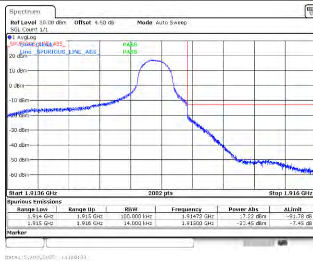
Band25_1.4MHz_16QAM_26683_1RB#5
