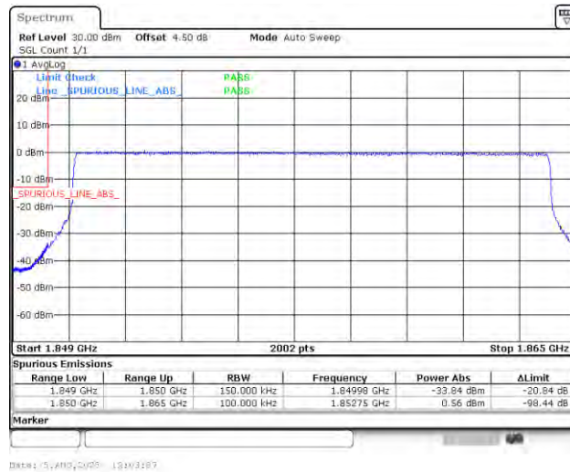
Band25_15MHz_QPSK_26115_75RB#0
