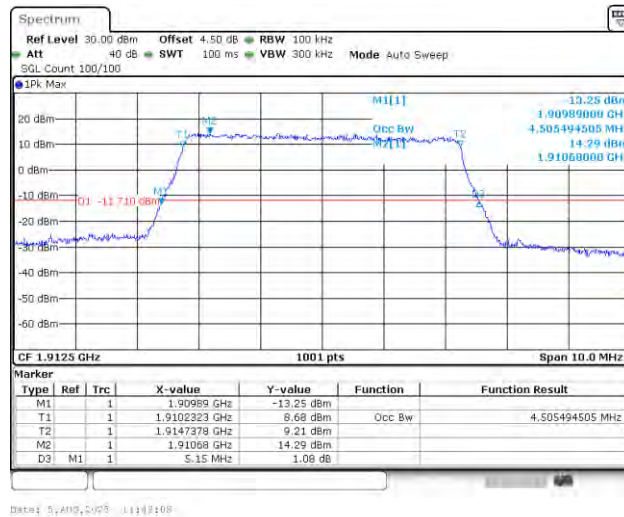
Band25-5MHz-QPSK-26665-25RB#0-PASS
