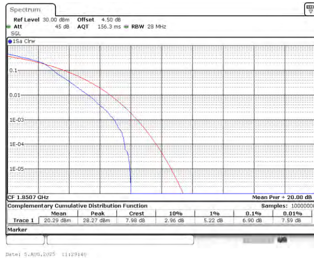
Band25-1.4MHz-16QAM-26047-1RB#0-PASS
