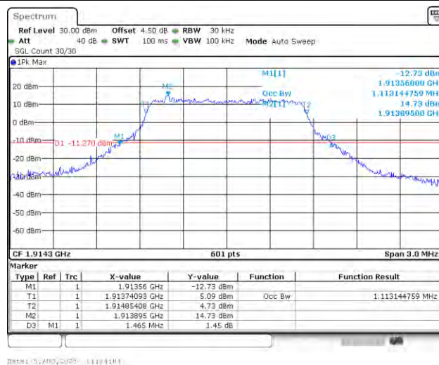
Band25-1.4MHz-16QAM-26683-6RB#0-PASS
