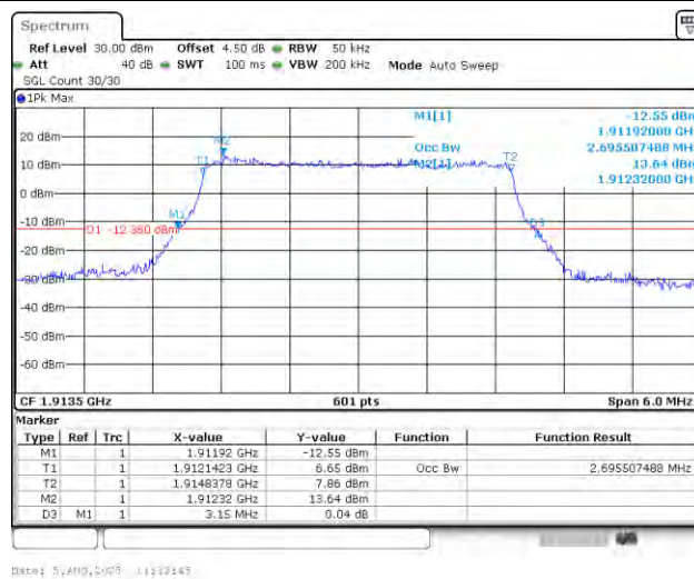
Band25-3MHz-16QAM-26675-15RB#0-PASS
