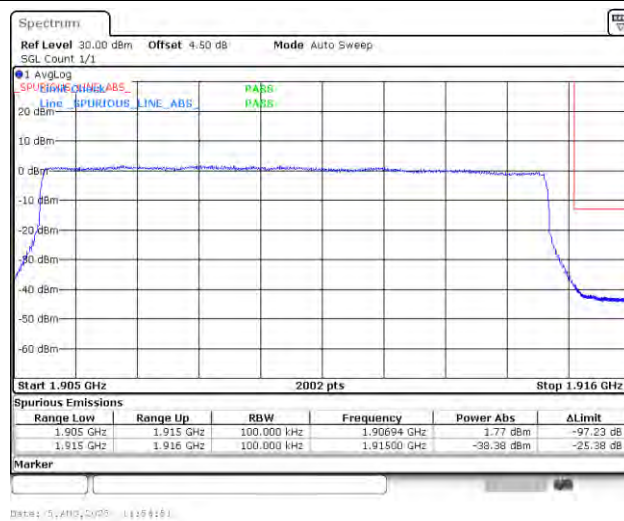
Band25_10MHz_QPSK_26640_50RB#0
