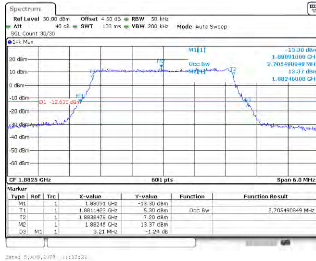
Band25-3MHz-16QAM-26365-15RB#0-PASS
