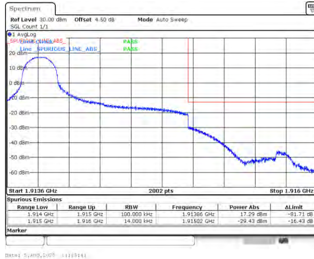
Band25_1.4MHz_16QAM_26683_1RB#0
