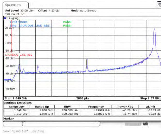
Band25_20MHz_16QAM_26140_1RB#99
