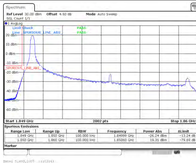
Band25_10MHz_QPSK_26090_1RB#0
