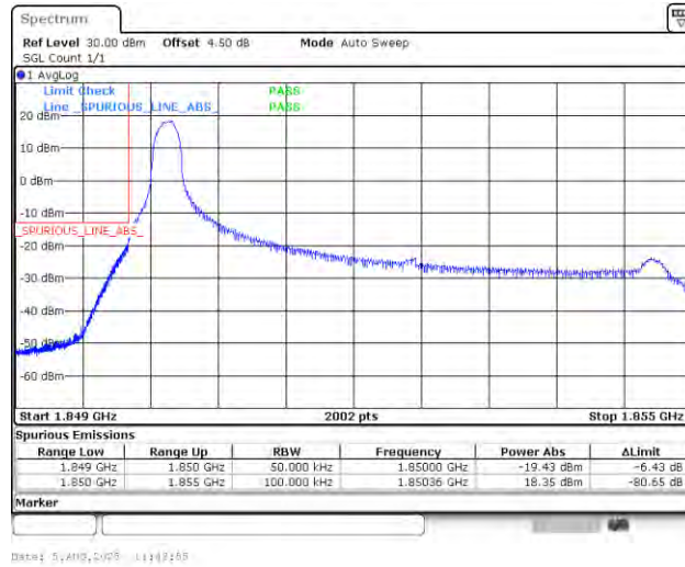
Band25_5MHz_16QAM_26065_1RB#0
