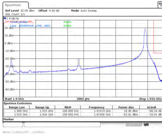
Band25_15MHz_QPSK_26615_1RB#74
