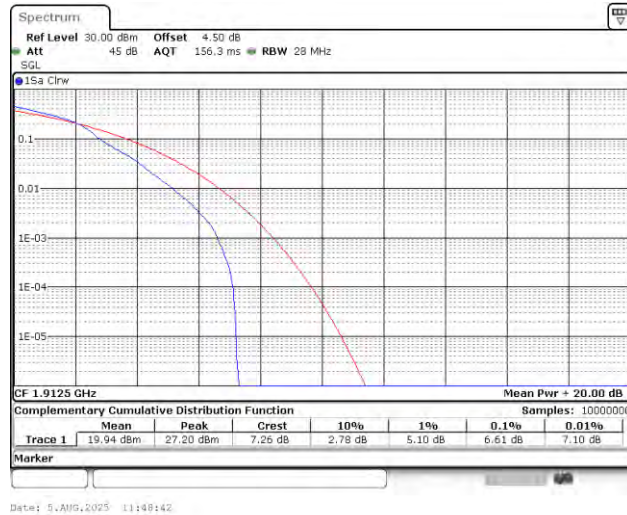
Band25-5MHz-16QAM-26665-1RB#0-PASS
