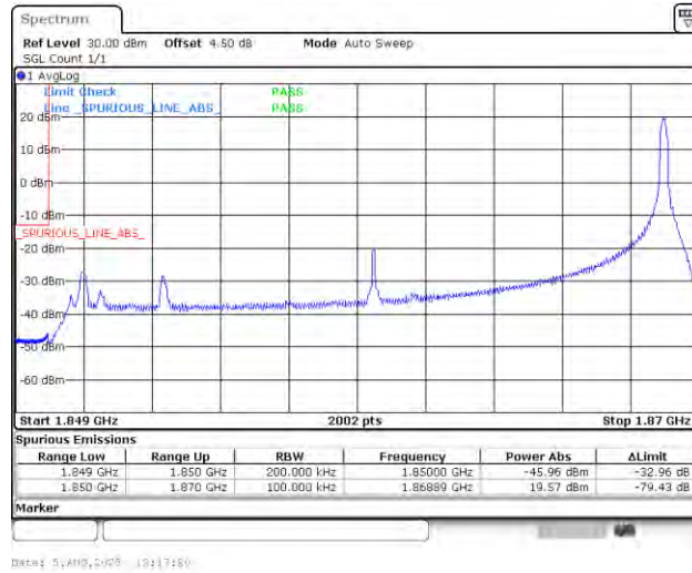
Band25_20MHz_QPSK_26140_1RB#99
