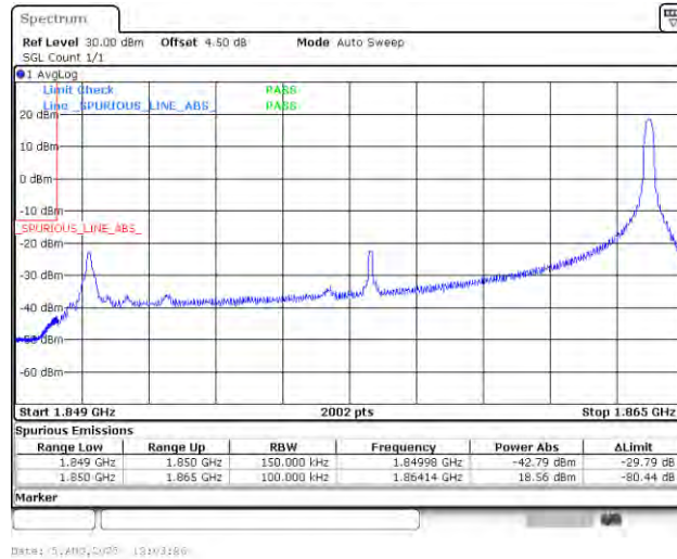
Band25_15MHz_16QAM_26115_1RB#74
