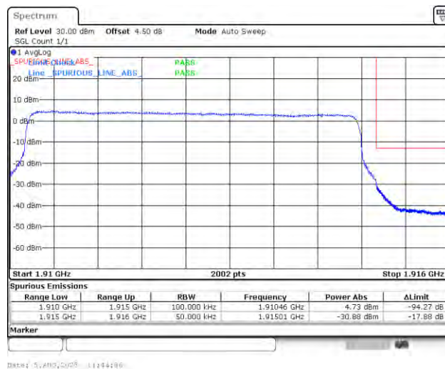
Band25_5MHz_QPSK_26665_25RB#0
