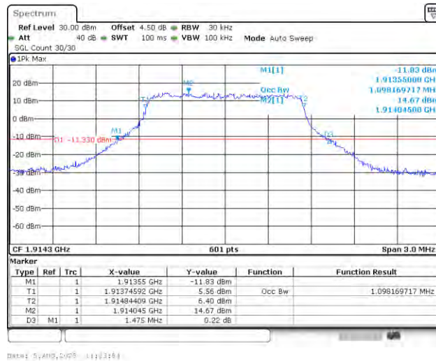
Band25-1.4MHz-QPSK-26683-6RB#0-PASS
