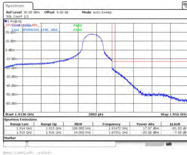
Band25_1.4MHz_QPSK_26683_1RB#5
