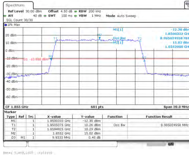
Band25-10MHz-QPSK-26090-50RB#0-PASS
