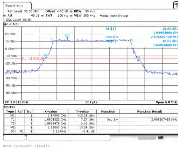
Band25-3MHz-16QAM-26055-15RB#0-PASS
