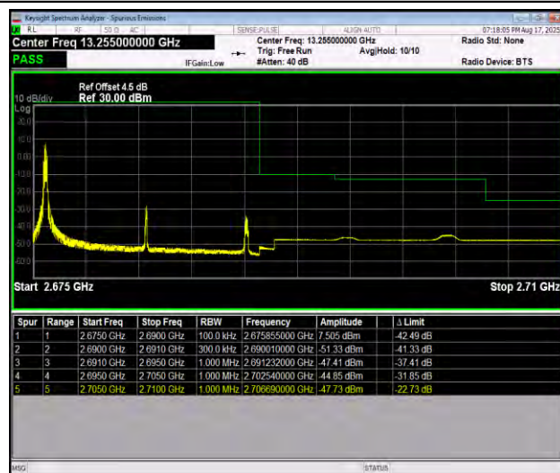
Band41_15MHz_16QAM_41515_1RB#0
