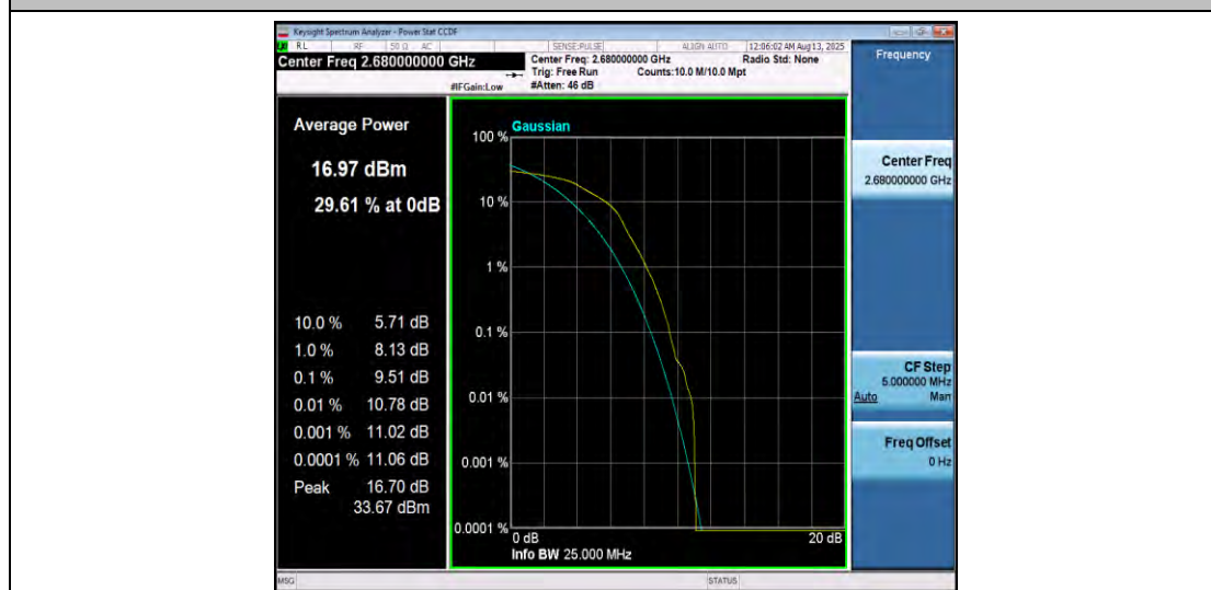
Band41-20MHz-16QAM-41490-1RB#0-PASS
