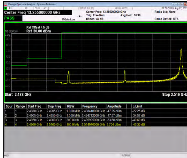
Band41_20MHz_16QAM_39750_1RB#99
