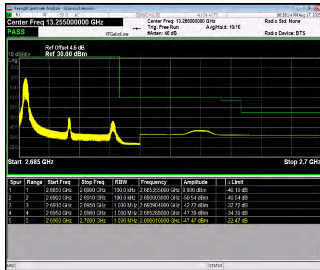
Band41_5MHz_QPSK_41565_1RB#0
