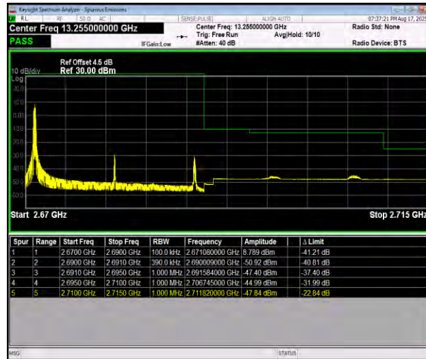
Band41_20MHz_16QAM_41490_1RB#0
