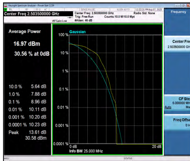
Band41-15MHz-16QAM-39725-1RB#0-PASS
