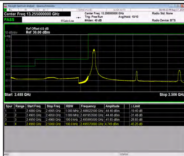
Band41_10MHz_16QAM_39700_1RB#0
