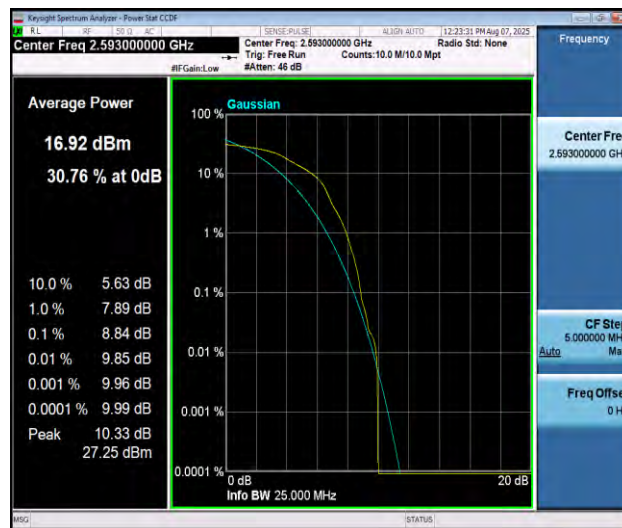
Band41-15MHz-16QAM-40620-1RB#0-PASS
