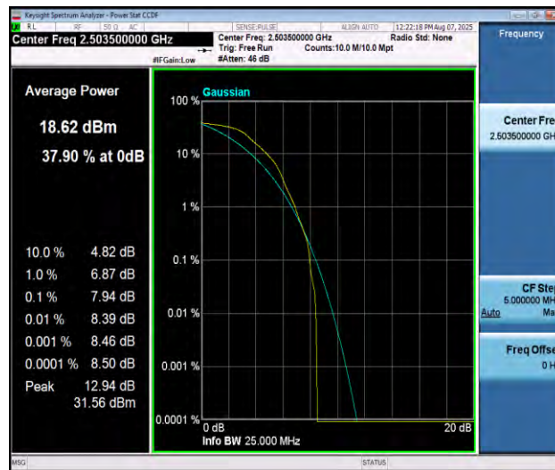
Band41-15MHz-QPSK-39725-1RB#0-PASS
