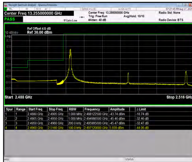
Band41_20MHz_16QAM_39750_1RB#0
