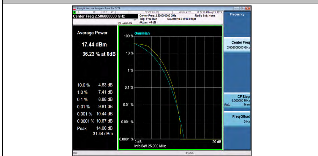
Band41-20MHz-QPSK-39750-100RB#0-PASS
