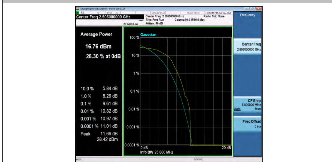
Band41-20MHz-16QAM-39750-1RB#0-PASS
