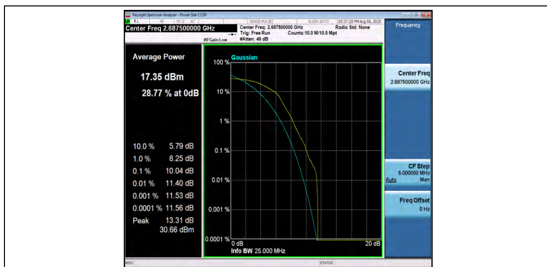
Band41-5MHz-16QAM-41565-1RB#0-PASS
