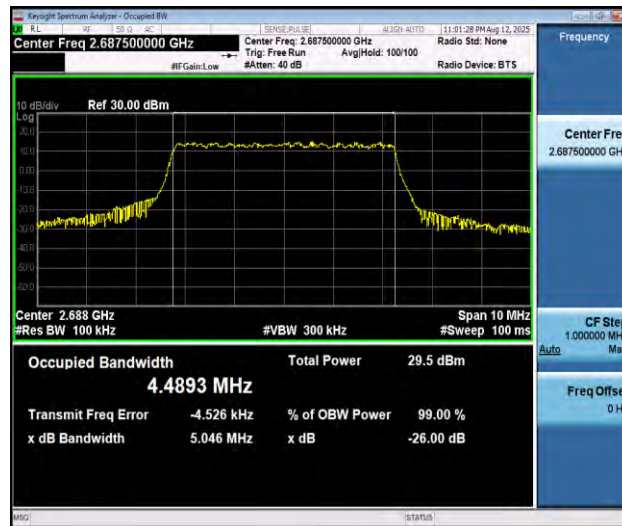
Band41-5MHz-QPSK-41565-25RB#0-PASS
