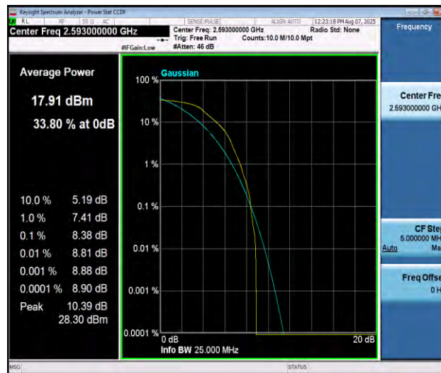
Band41-15MHz-QPSK-40620-1RB#0-PASS
