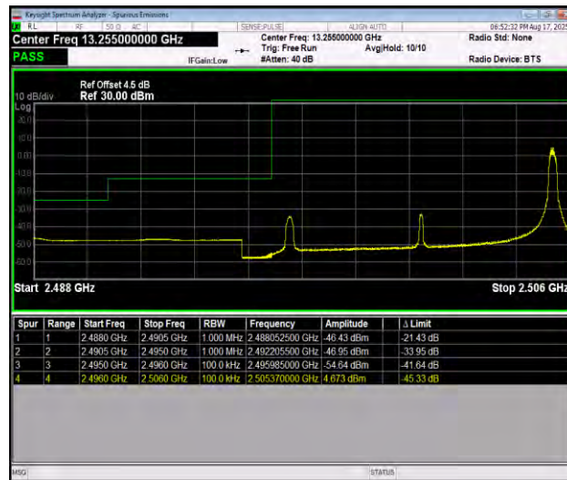
Band41_10MHz_16QAM_39700_1RB#49
