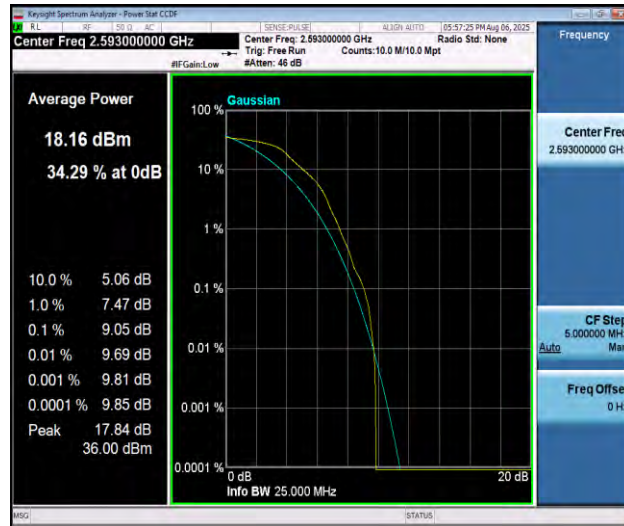
Band41-10MHz-QPSK-40620-1RB#0-PASS
