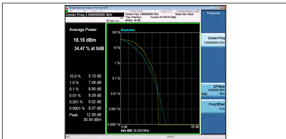
Band41-20MHz-QPSK-39750-1RB#0-PASS
