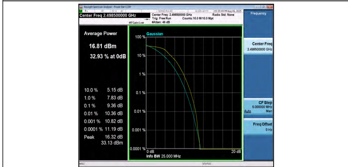
Band41-5MHz-QPSK-39675-25RB#0-PASS
