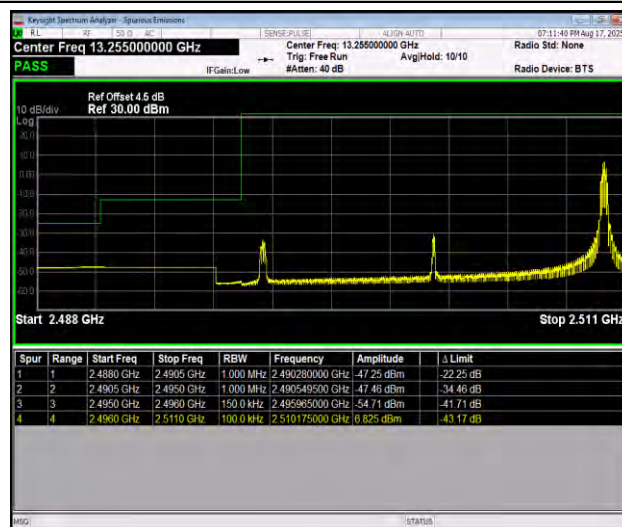
Band41_15MHz_16QAM_39725_1RB#74
