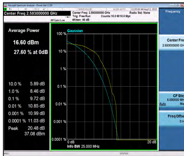
Band41-20MHz-16QAM-40620-1RB#0-PASS
