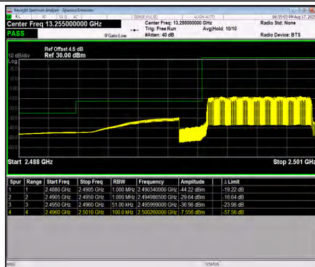
Band41_5MHz_QPSK_39675_25RB#0
