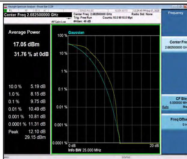
Band41-15MHz-QPSK-41515-75RB#0-PASS
