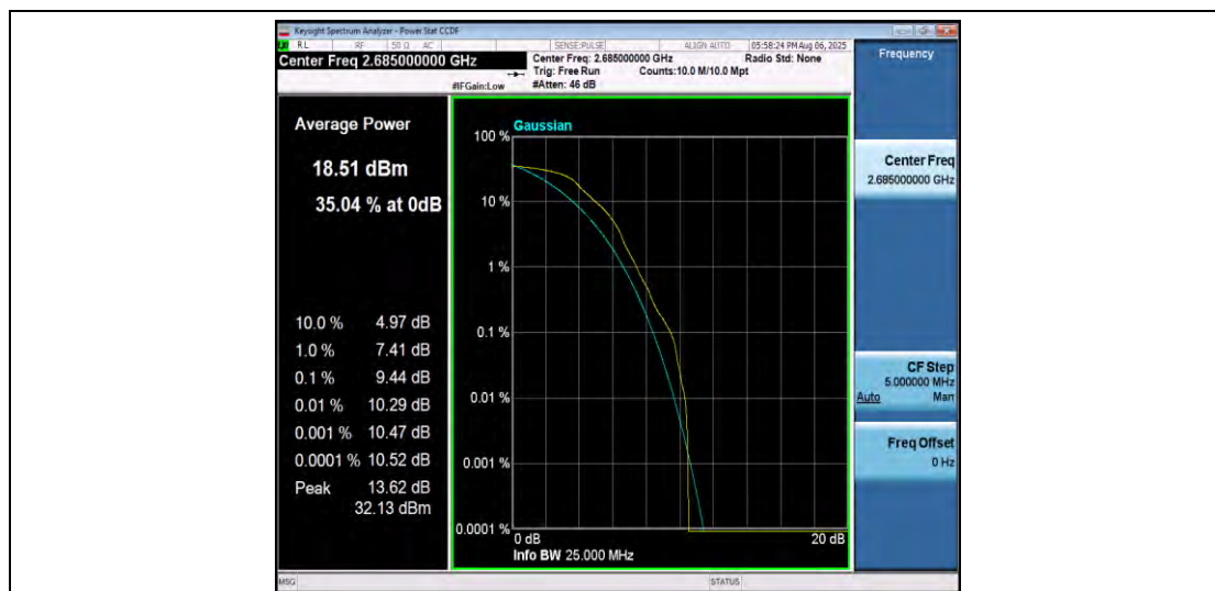
Band41-10MHz-QPSK-41540-1RB#0-PASS
