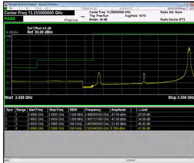
Band41_10MHz_QPSK_39700_1RB#49
