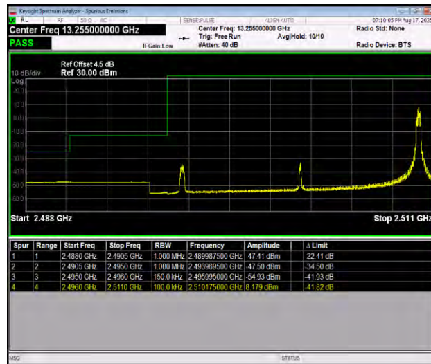
Band41_15MHz_QPSK_39725_1RB#74
