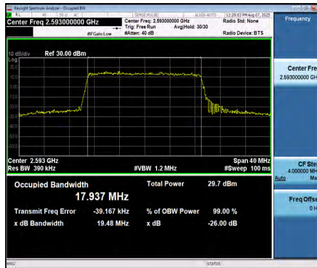
Band41-20MHz-QPSK-40620-100RB#0-PASS
