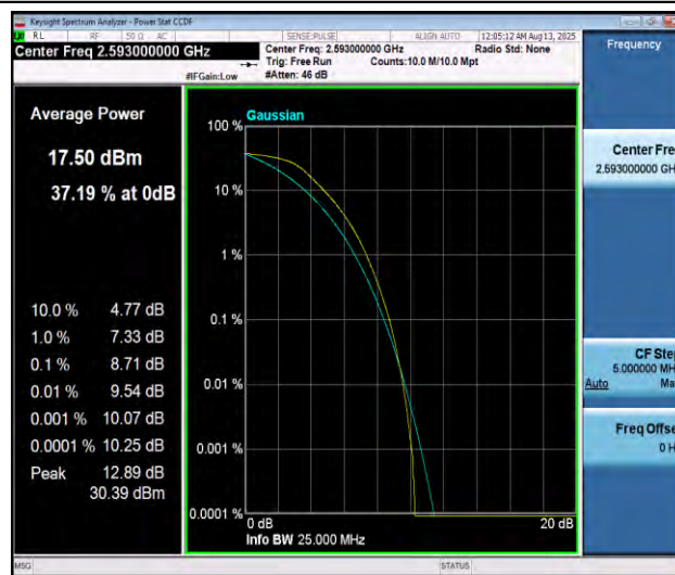
Band41-20MHz-QPSK-40620-100RB#0-PASS
