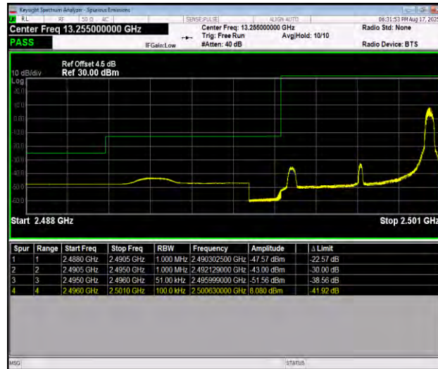
Band41_5MHz_QPSK_39675_1RB#24
