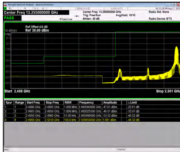
Band41_5MHz_16QAM_39675_1RB#24
