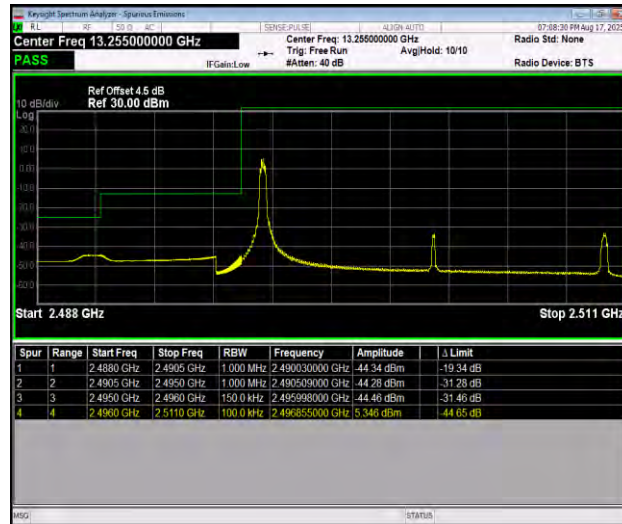
Band41_15MHz_16QAM_39725_1RB#0
