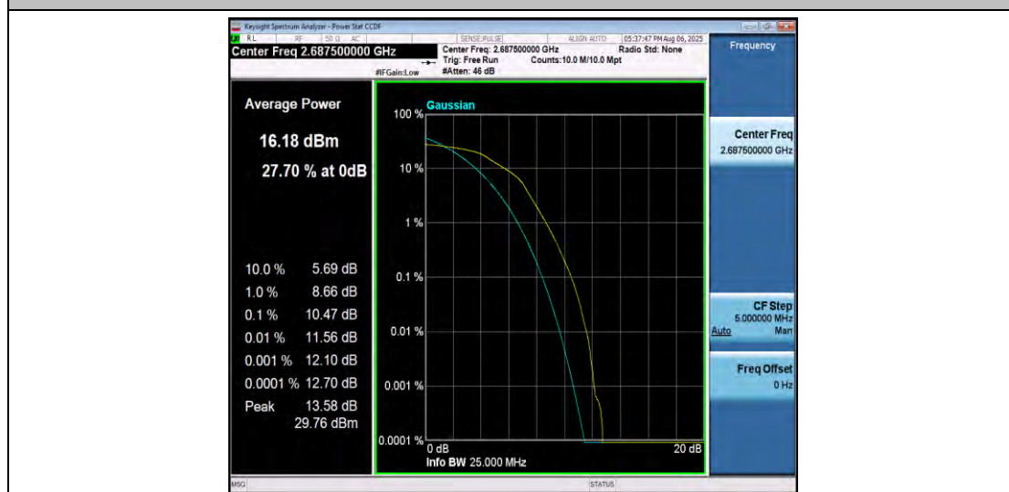
Band41-5MHz-16QAM-41565-25RB#0-PASS
