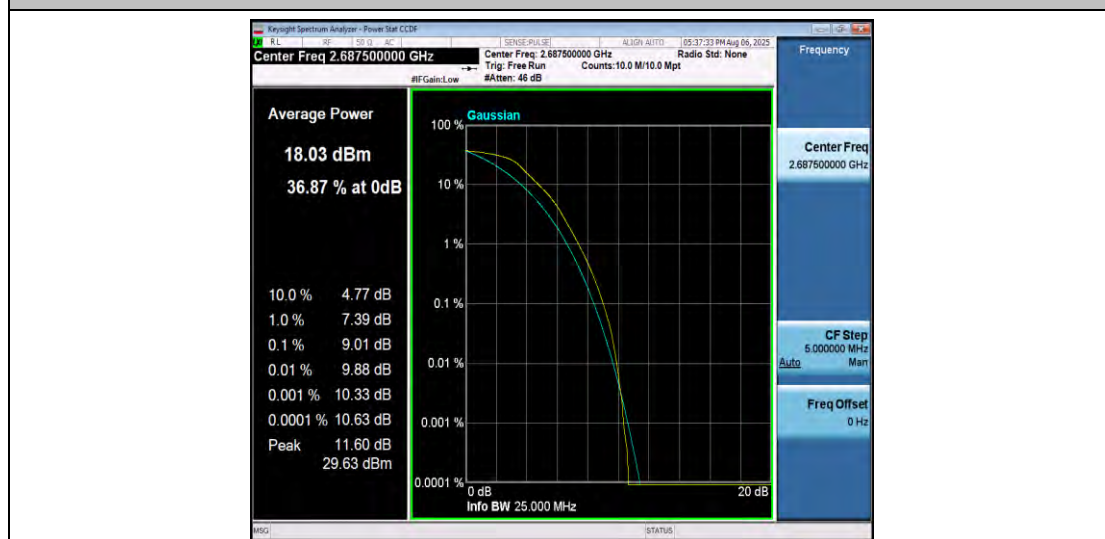
Band41-5MHz-QPSK-41565-25RB#0-PASS
