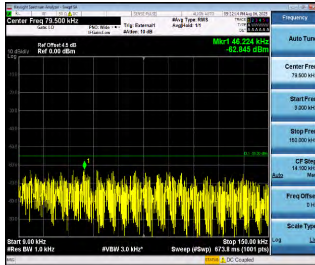
Band41_5MHz_16QAM_40620_1RB#0_0.009~0.15_0.009~0.15
