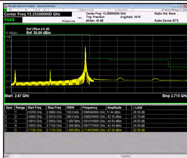
Band41_20MHz_16QAM_41490_1RB#99
