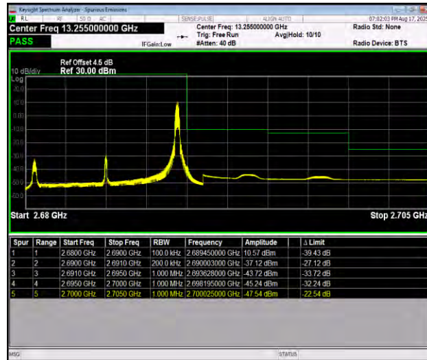
Band41_10MHz_16QAM_41540_1RB#49
