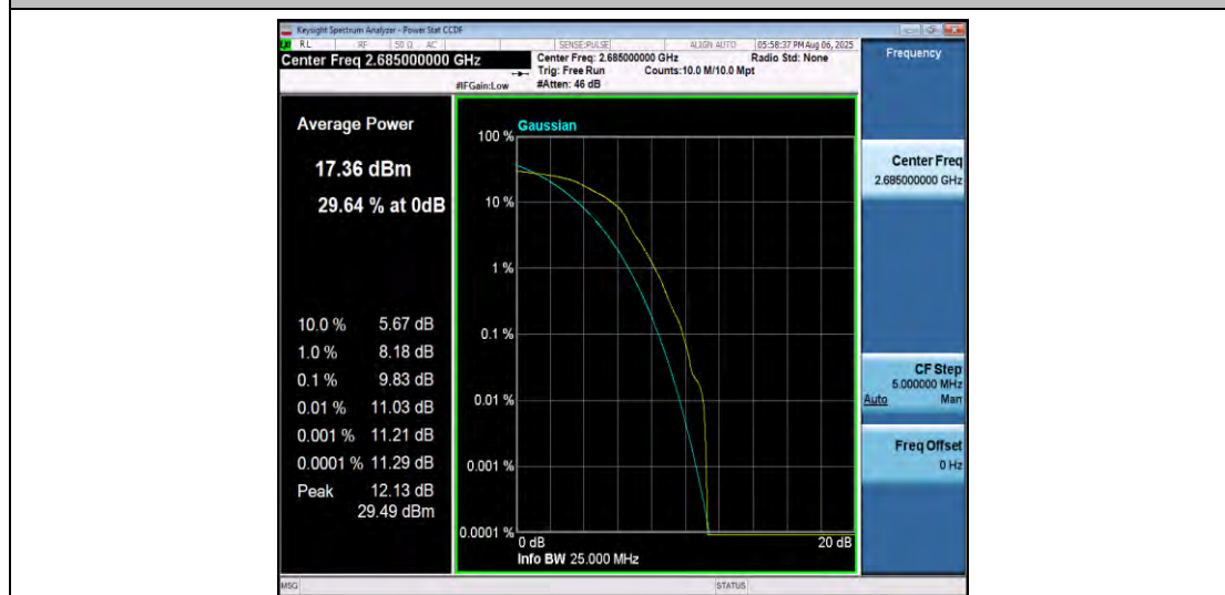
Band41-10MHz-16QAM-41540-1RB#0-PASS
