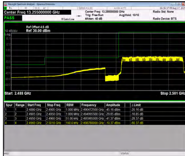
Band41_5MHz_16QAM_39675_25RB#0
