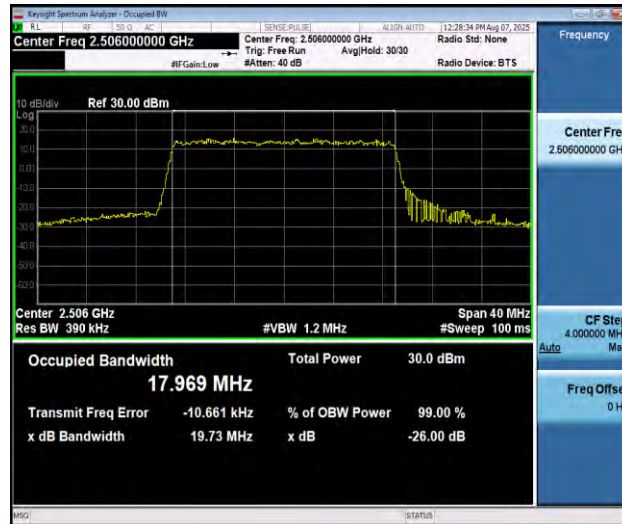
Band41-20MHz-QPSK-39750-100RB#0-PASS
