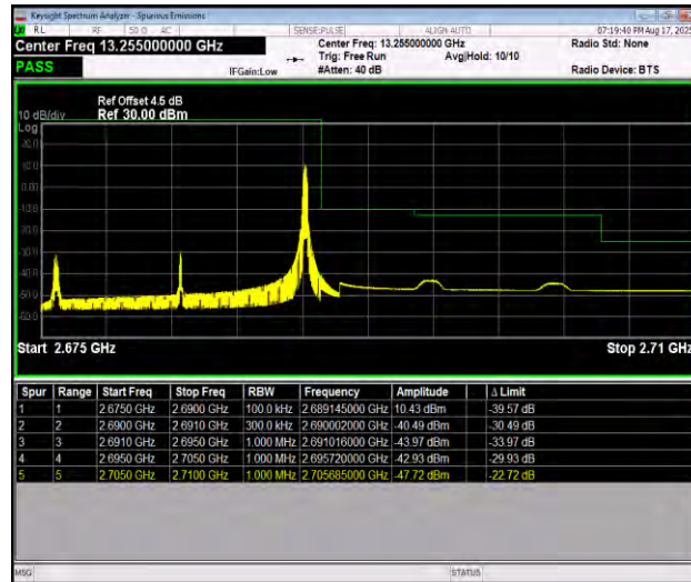
Band41_15MHz_QPSK_41515_1RB#74
