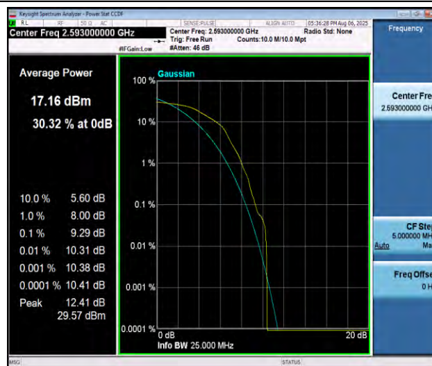
Band41-5MHz-16QAM-40620-1RB#0-PASS
