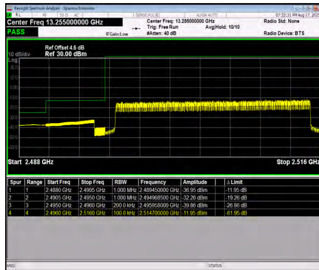
Band41_20MHz_QPSK_39750_100RB#0
