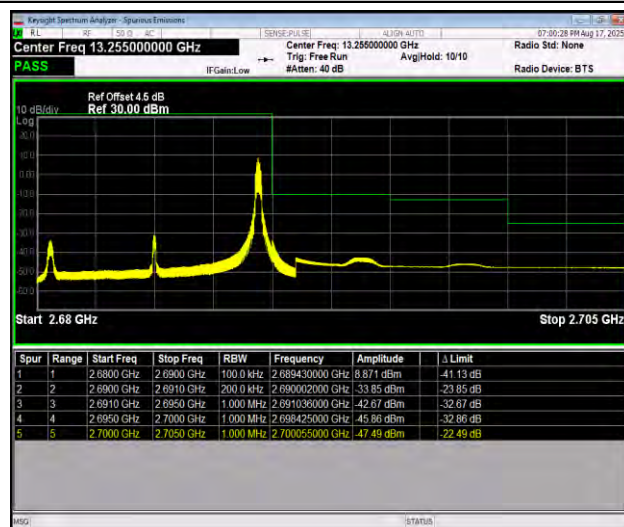
Band41_10MHz_QPSK_41540_1RB#49
