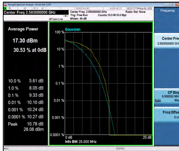
Band41-10MHz-16QAM-40620-1RB#0-PASS
