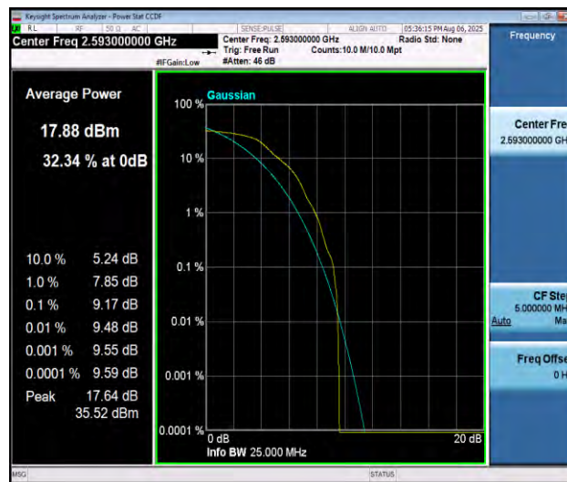
Band41-5MHz-QPSK-40620-1RB#0-PASS
