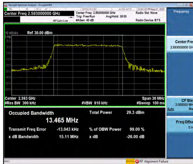
Band41-15MHz-QPSK-40620-75RB#0-PASS
