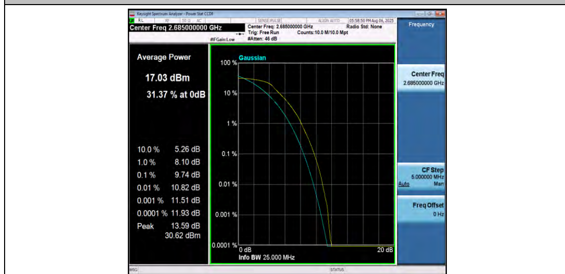
Band41-10MHz-QPSK-41540-50RB#0-PASS
