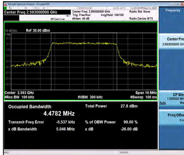
Band41-5MHz-16QAM-40620-25RB#0-PASS
