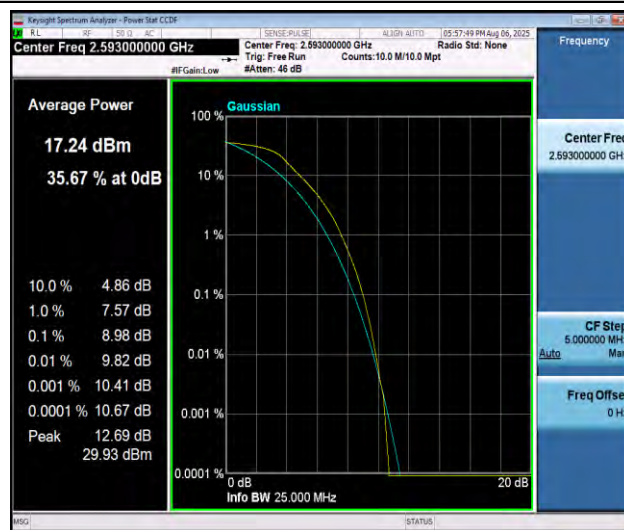
Band41-10MHz-QPSK-40620-50RB#0-PASS
