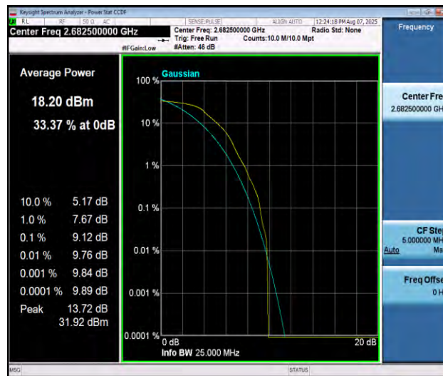
Band41-15MHz-QPSK-41515-1RB#0-PASS
