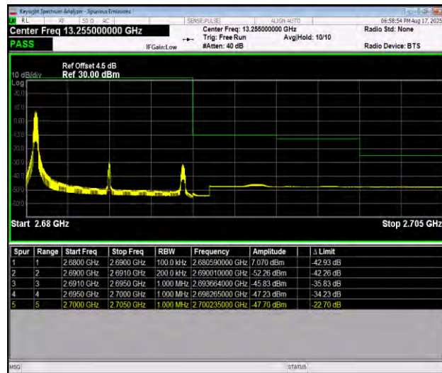
Band41_10MHz_16QAM_41540_1RB#0
