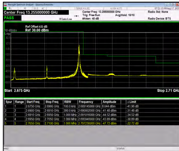
Band41_15MHz_16QAM_41515_1RB#74
