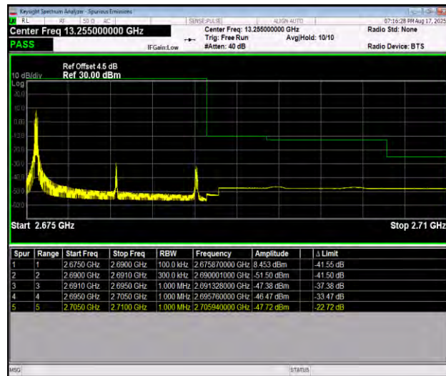
Band41_15MHz_QPSK_41515_1RB#0
