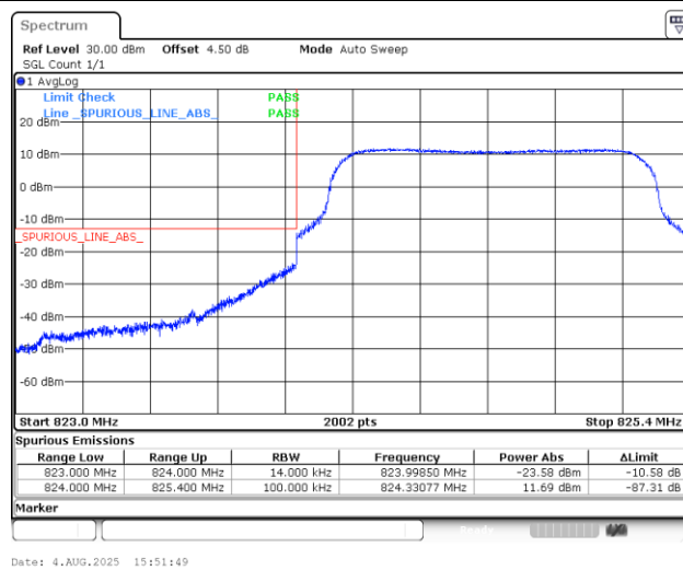
Band5_1.4MHz_QPSK_20407_6RB#0
