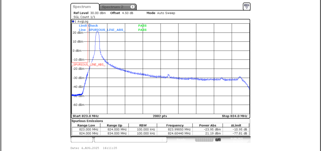
Band5_10MHz_QPSK_20450_1RB#0
