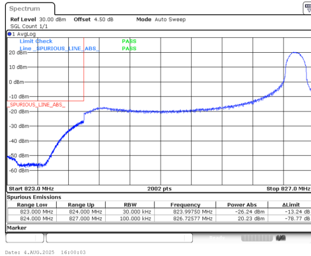
Band5_3MHz_QPSK_20415_1RB#14
