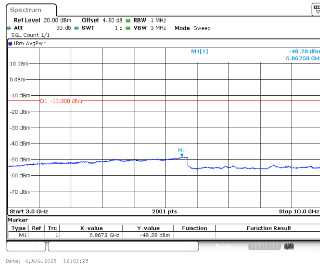
Band5_3MHz_QPSK_20415_1RB#0_3000~10000_3000~10000
