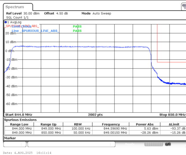
Band5_5MHz_QPSK_20625_25RB#0
