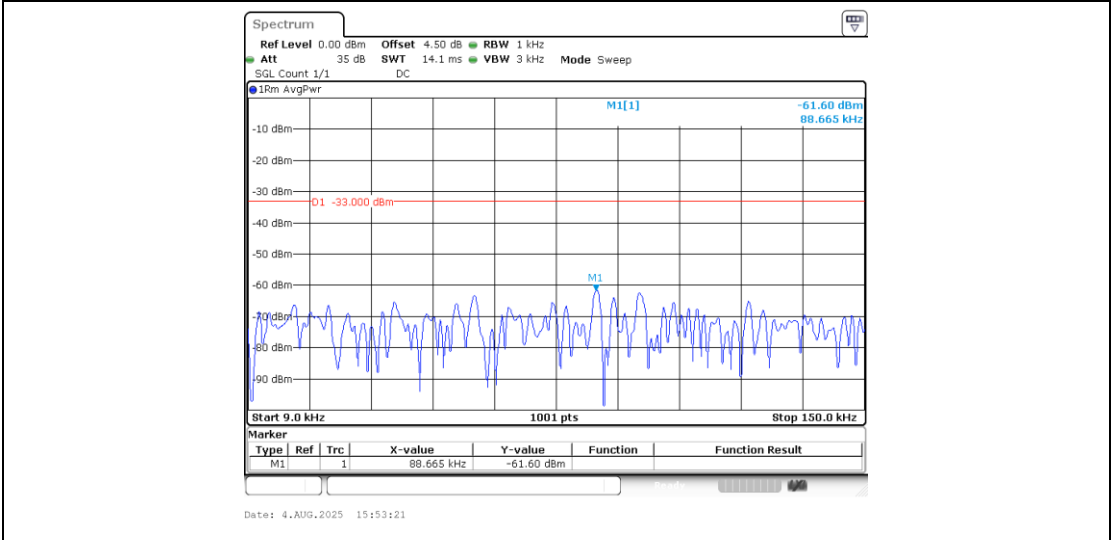
Band5_1.4MHz_QPSK_20407_1RB#0_0.009~0.15_0.009~0.15
