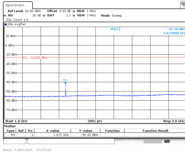
Band5_1.4MHz_16QAM_20525_1RB#0_1000~3000_1000~3000
