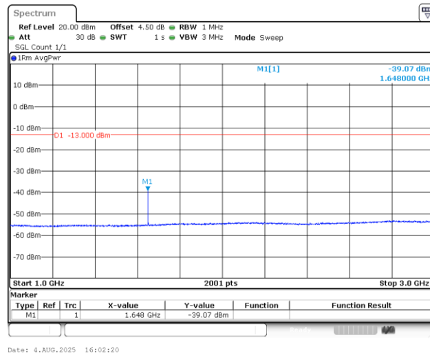
Band5_3MHz_QPSK_20415_1RB#0_1000~3000_1000~3000
