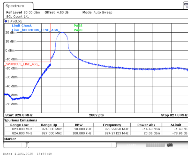
Band5_3MHz_QPSK_20415_1RB#0
