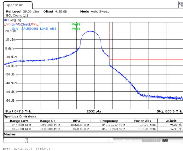
Band5_1.4MHz_QPSK_20643_1RB#5
