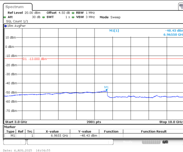
Band5_3MHz_16QAM_20635_1RB#0_3000~10000_3000~10000
