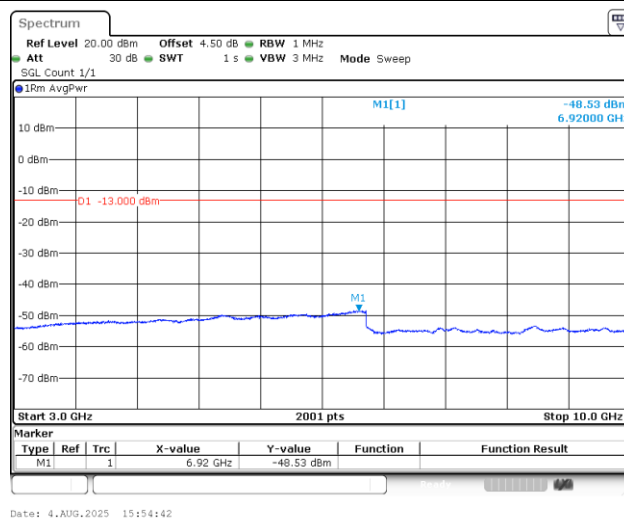
Band5_1.4MHz_QPSK_20525_1RB#0_3000~10000_3000~10000
