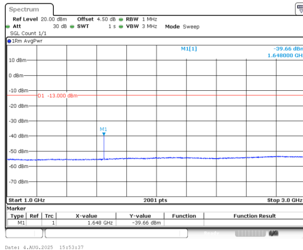
Band5_1.4MHz_QPSK_20407_1RB#0_1000~3000_1000~3000
