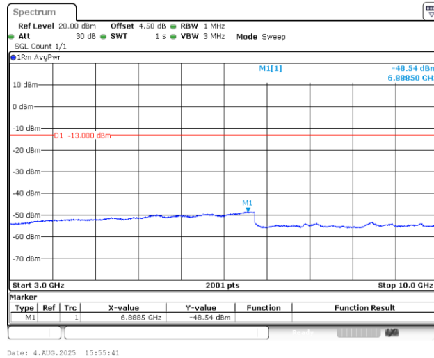
Band5_1.4MHz_QPSK_20643_1RB#0_3000~10000_3000~10000
