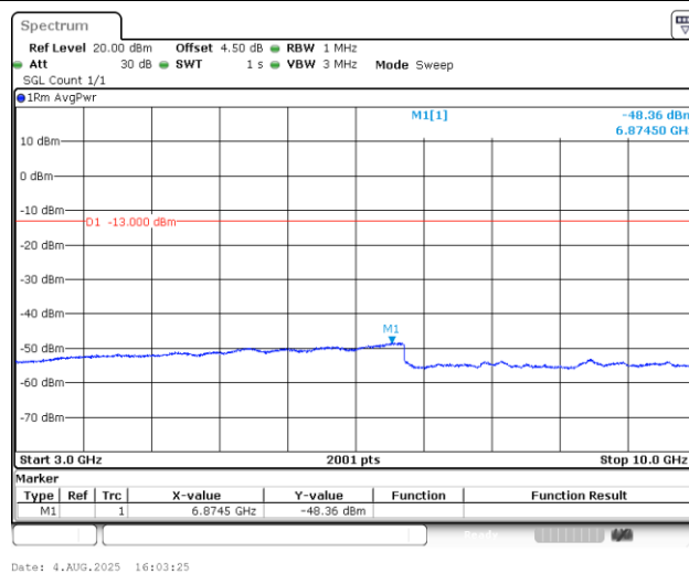
Band5_3MHz_QPSK_20525_1RB#0_3000~10000_3000~10000
