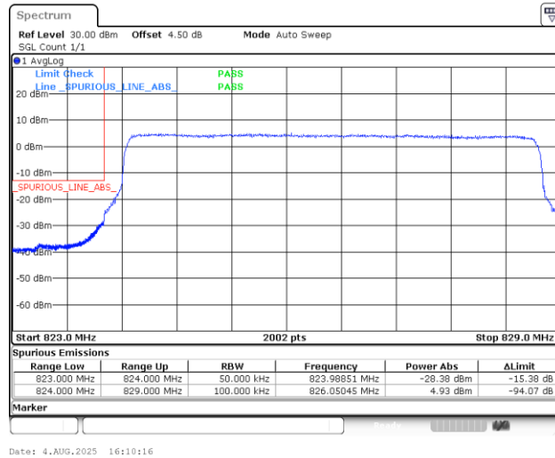
Band5_5MHz_16QAM_20425_25RB#0
