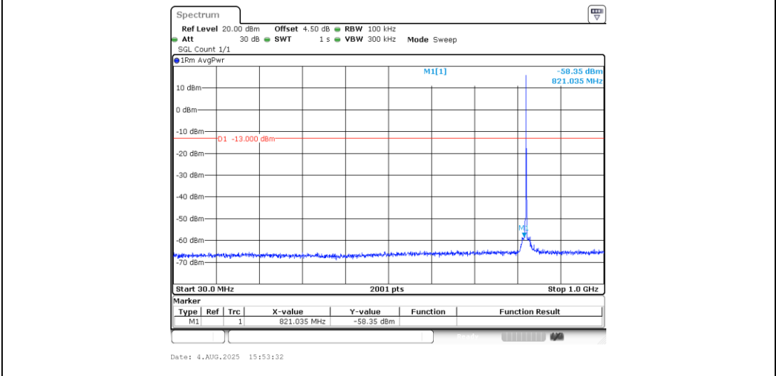
Band5_1.4MHz_QPSK_20407_1RB#0_30~1000_30~1000
