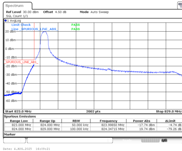
Band5_5MHz_QPSK_20425_1RB#0
