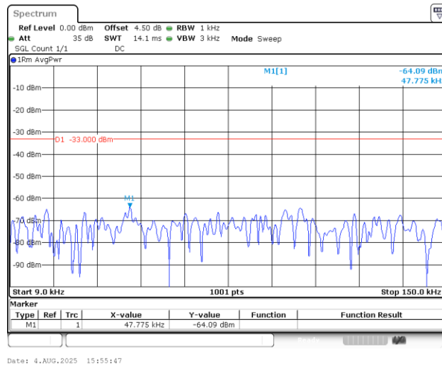
Band5_1.4MHz_16QAM_20643_1RB#0_0.009~0.15_0.009~0.15
