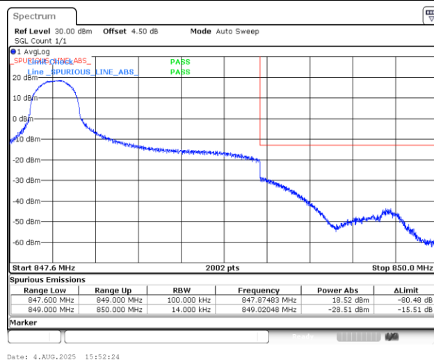
Band5_1.4MHz_16QAM_20643_1RB#0
