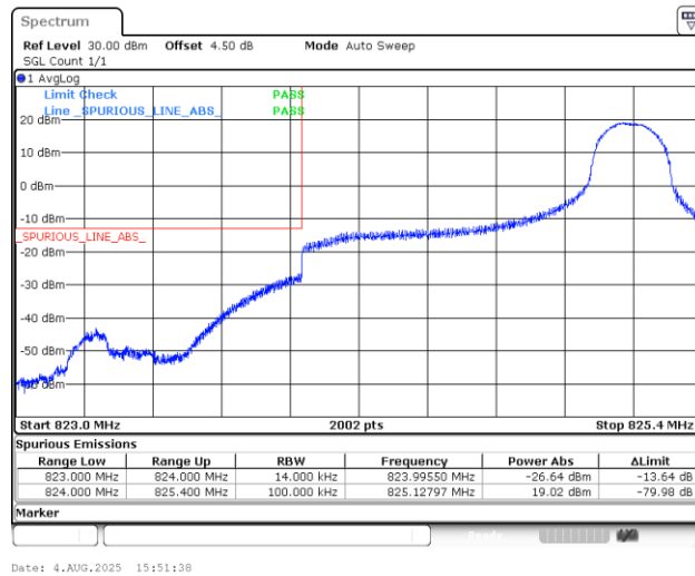
Band5_1.4MHz_16QAM_20407_1RB#5
