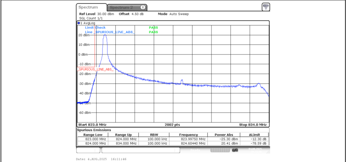
Band5_10MHz_16QAM_20450_1RB#0
