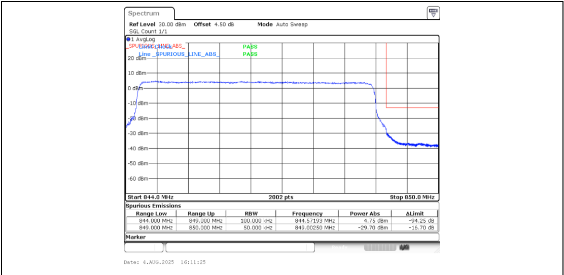
Band5_5MHz_16QAM_20625_25RB#0
