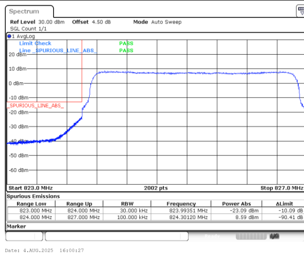
Band5_3MHz_QPSK_20415_15RB#0
