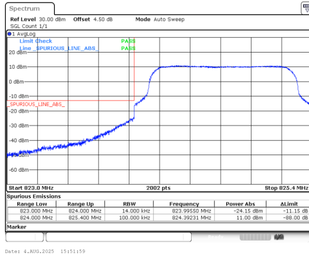
Band5_1.4MHz_16QAM_20407_6RB#0
