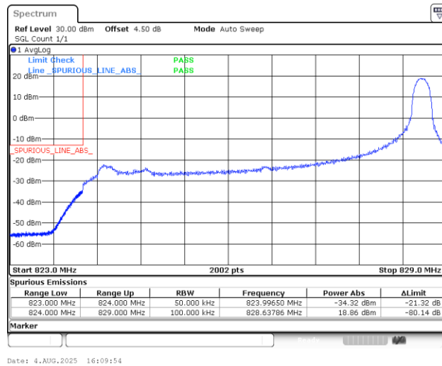
Band5_5MHz_16QAM_20425_1RB#24
