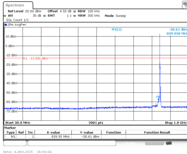
Band5_3MHz_16QAM_20635_1RB#0_30~1000_30~1000
