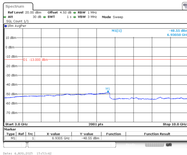
Band5_1.4MHz_QPSK_20407_1RB#0_3000~10000_3000~10000
