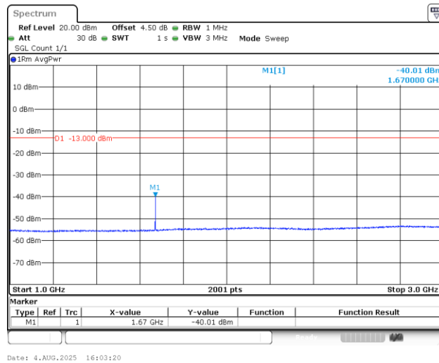
Band5_3MHz_QPSK_20525_1RB#0_1000~3000_1000~3000
