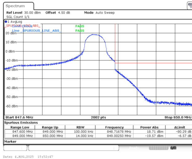
Band5_1.4MHz_16QAM_20643_1RB#5
