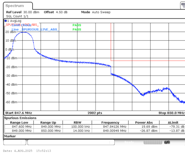
Band5_1.4MHz_QPSK_20643_1RB#0
