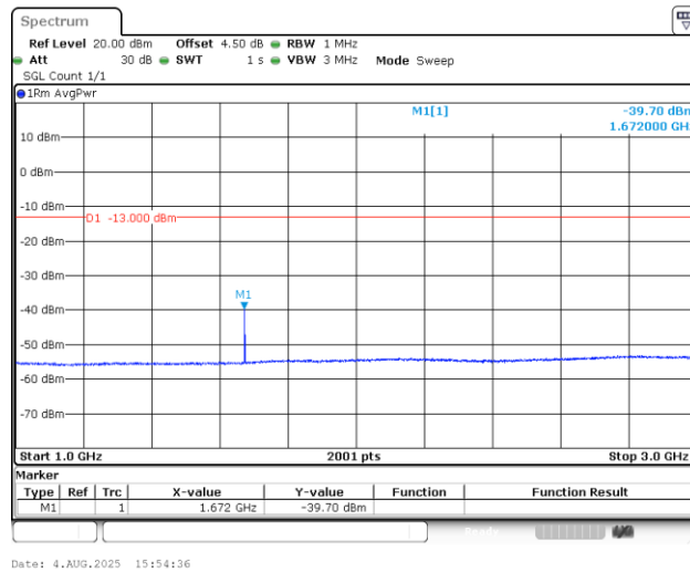
Band5_1.4MHz_QPSK_20525_1RB#0_1000~3000_1000~3000
