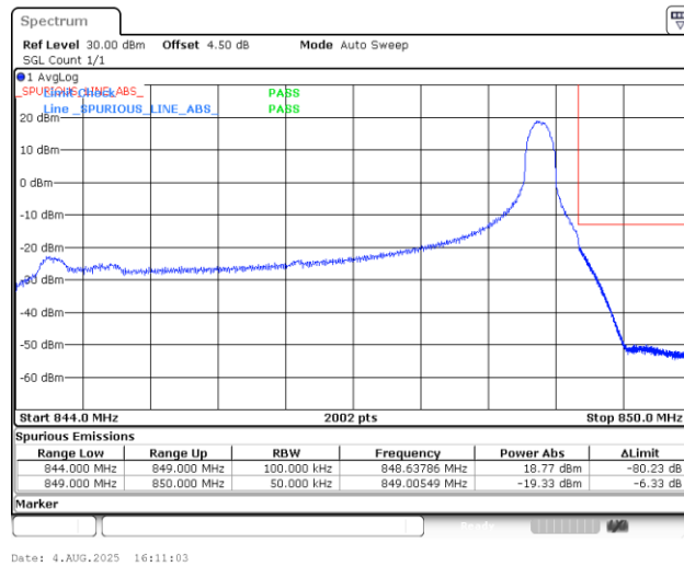
Band5_5MHz_16QAM_20625_1RB#24
