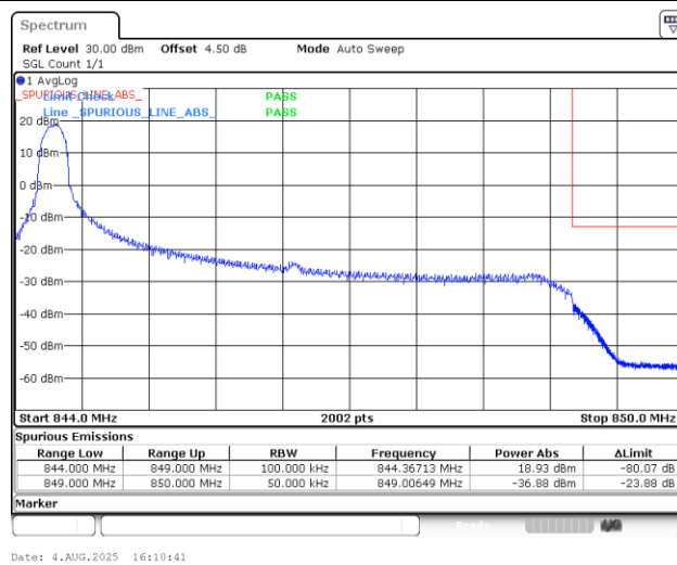
Band5_5MHz_16QAM_20625_1RB#0
