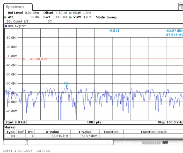
Band5_3MHz_16QAM_20415_1RB#0_0.009~0.15_0.009~0.15
