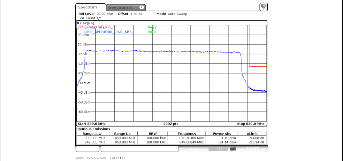
Band5_10MHz_QPSK_20600_50RB#0
