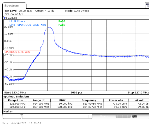
Band5_3MHz_16QAM_20415_1RB#0
