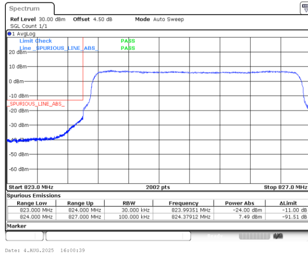
Band5_3MHz_16QAM_20415_15RB#0
