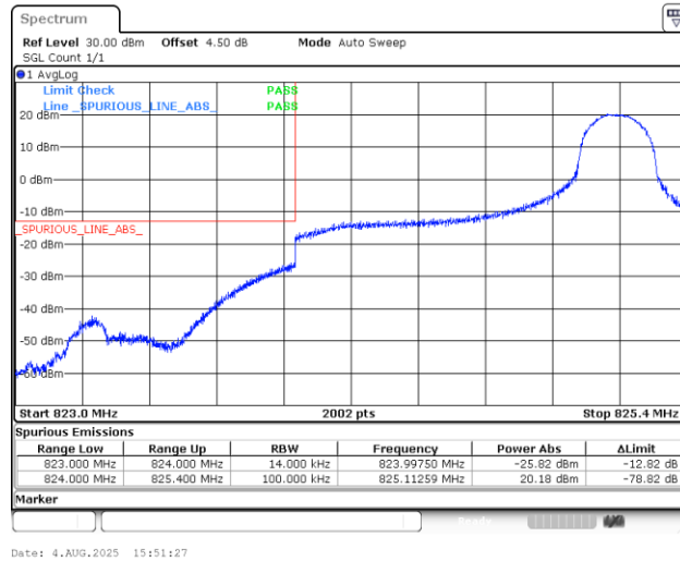
Band5_1.4MHz_QPSK_20407_1RB#5
