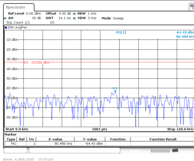
Band5_1.4MHz_QPSK_20643_1RB#0_0.009~0.15_0.009~0.15
