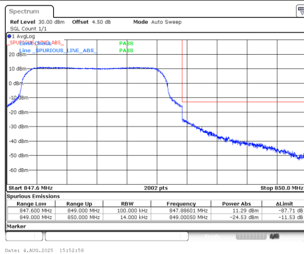
Band5_1.4MHz_QPSK_20643_6RB#0
