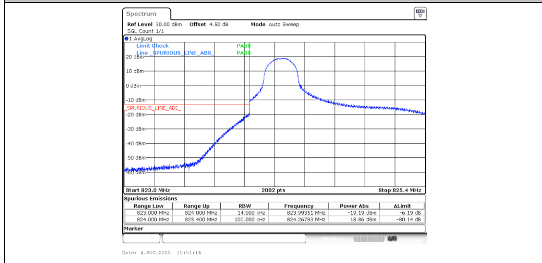
Band5_1.4MHz_16QAM_20407_1RB#0
