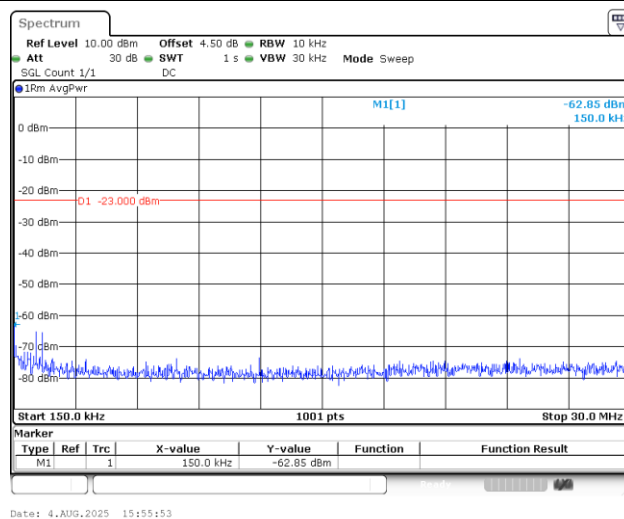
Band5_1.4MHz_16QAM_20643_1RB#0_0.15~30_0.15~30
