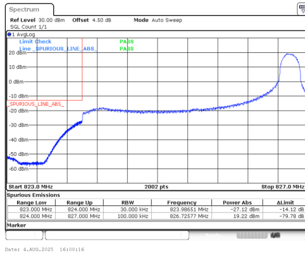
Band5_3MHz_16QAM_20415_1RB#14
