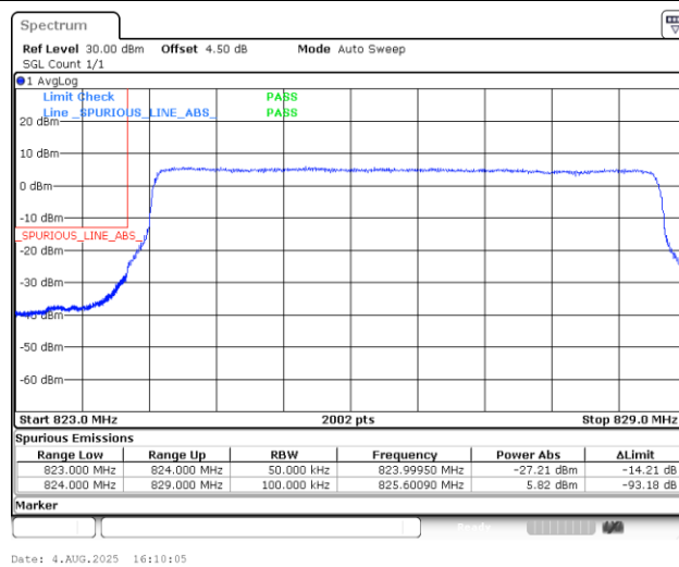
Band5_5MHz_QPSK_20425_25RB#0
