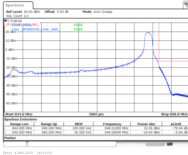
Band5_5MHz_QPSK_20625_1RB#24
