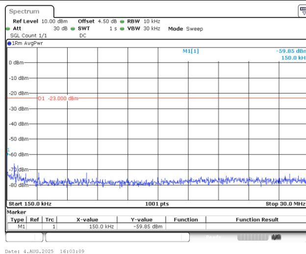
Band5_3MHz_QPSK_20525_1RB#0_0.15~30_0.15~30
