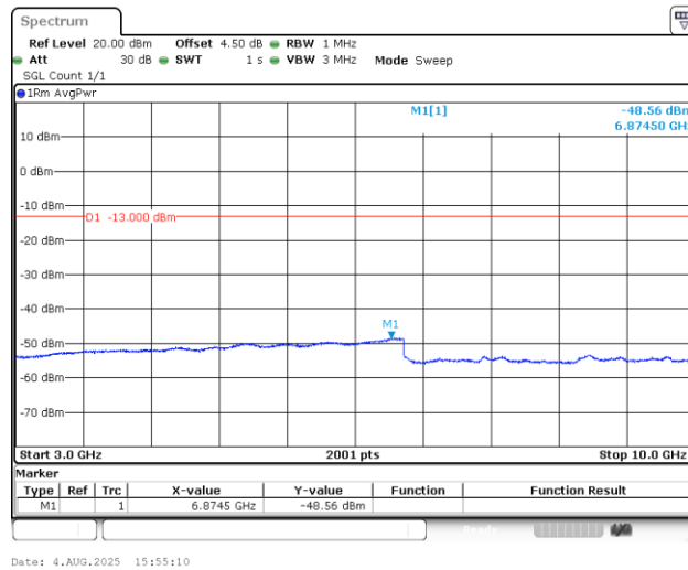
Band5_1.4MHz_16QAM_20525_1RB#0_3000~10000_3000~10000
