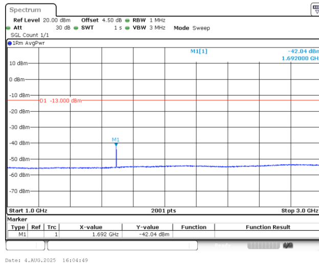
Band5_3MHz_16QAM_20635_1RB#0_1000~3000_1000~3000
