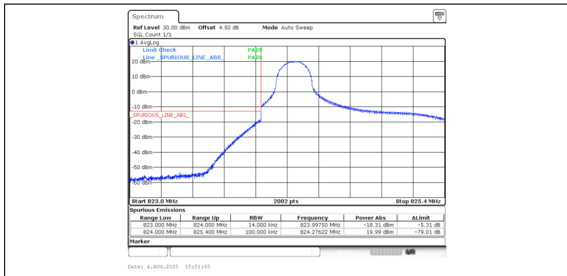
Band5_1.4MHz_QPSK_20407_1RB#0
