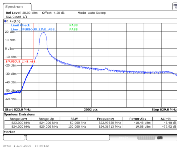
Band5_5MHz_16QAM_20425_1RB#0
