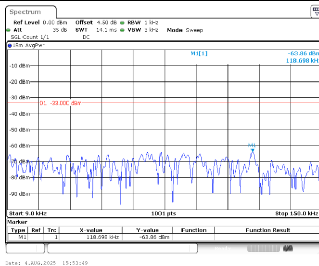
Band5_1.4MHz_16QAM_20407_1RB#0_0.009~0.15_0.009~0.15
