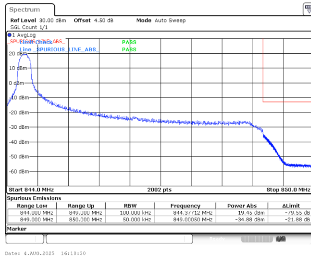
Band5_5MHz_QPSK_20625_1RB#0
