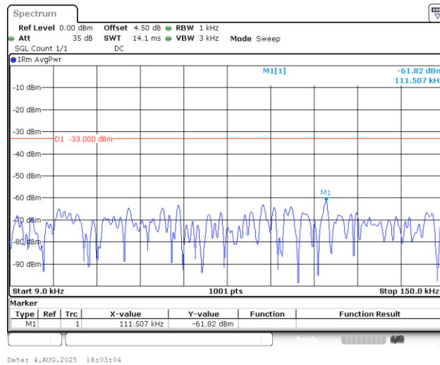
Band5_3MHz_QPSK_20525_1RB#0_0.009~0.15_0.009~0.15
