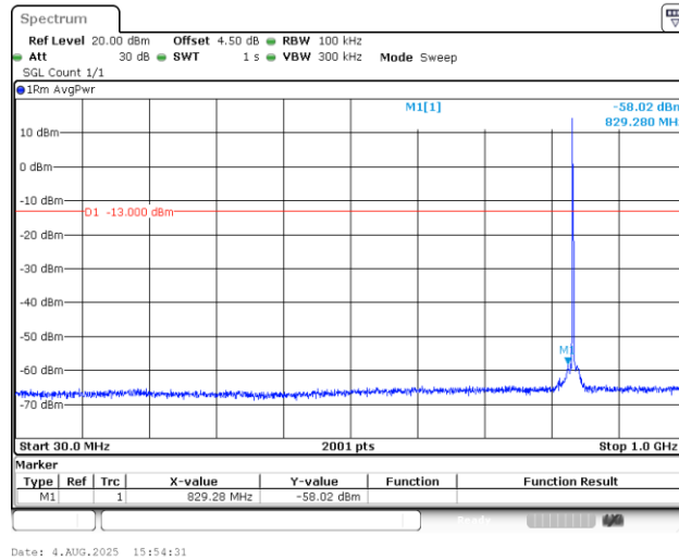
Band5_1.4MHz_QPSK_20525_1RB#0_30~1000_30~1000
