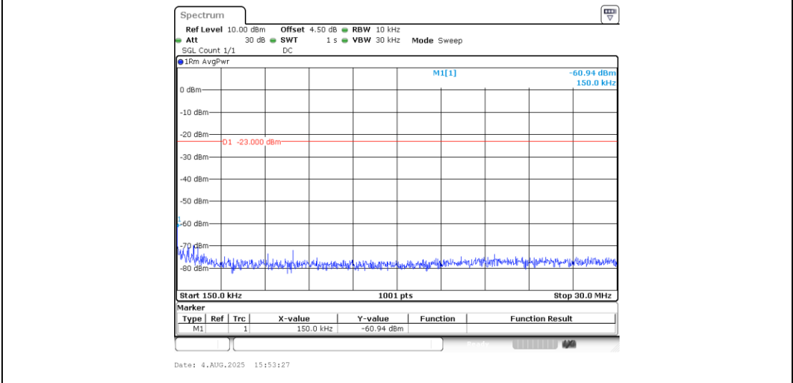
Band5_1.4MHz_QPSK_20407_1RB#0_0.15~30_0.15~30
