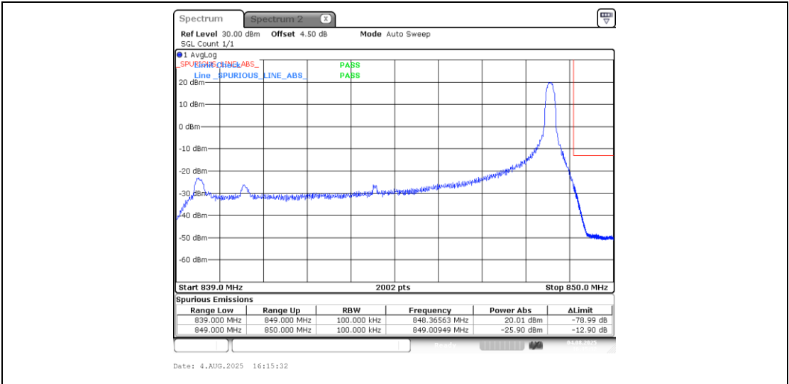
Band5_10MHz_16QAM_20600_1RB#49
