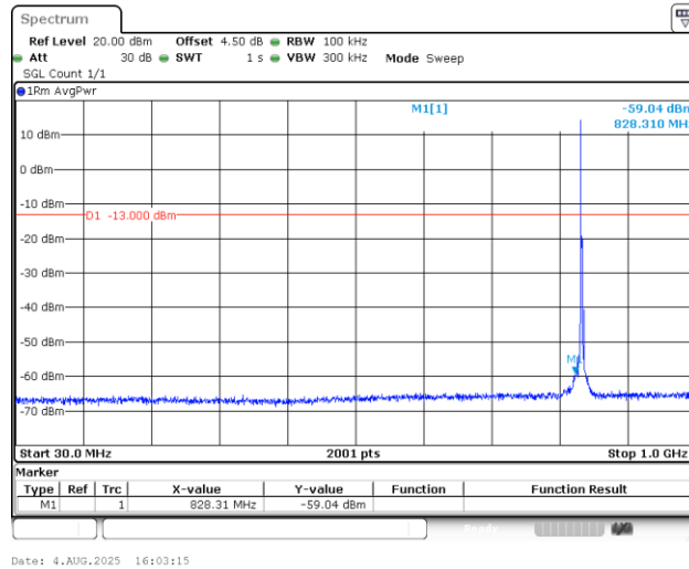
Band5_3MHz_QPSK_20525_1RB#0_30~1000_30~1000
