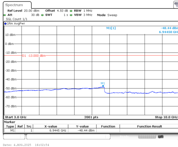
Band5_3MHz_16QAM_20415_1RB#0_3000~10000_3000~10000
