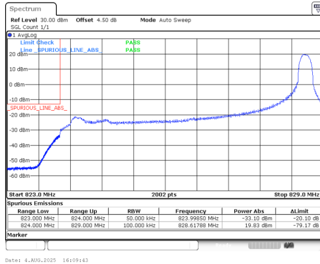
Band5_5MHz_QPSK_20425_1RB#24
