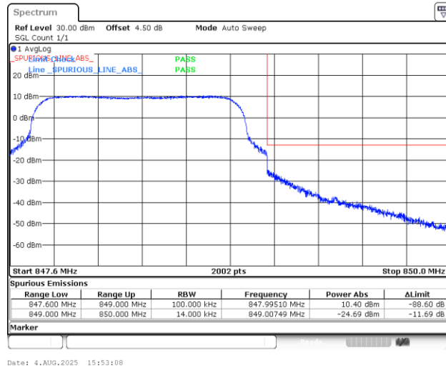
Band5_1.4MHz_16QAM_20643_6RB#0
