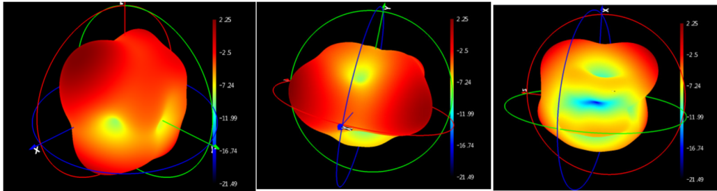
Gain—WIFI5.8G—5480MHz
