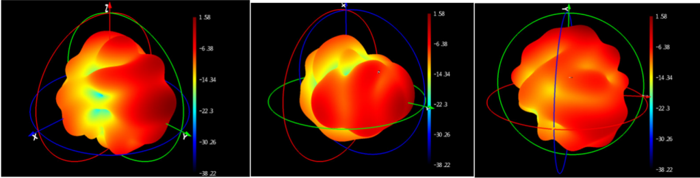
Gain—wifi—5480MHz
