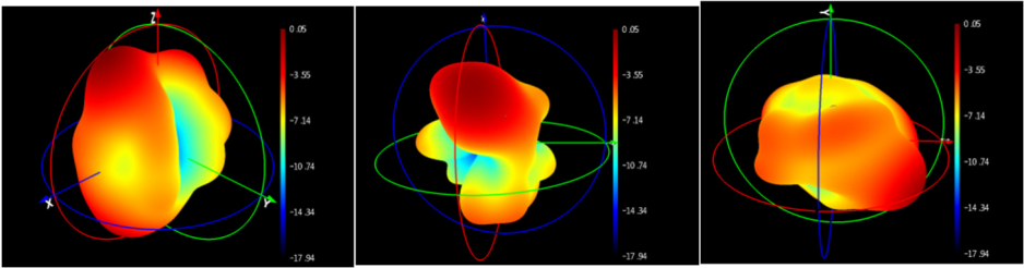
Gain—wifi—5480MHz
