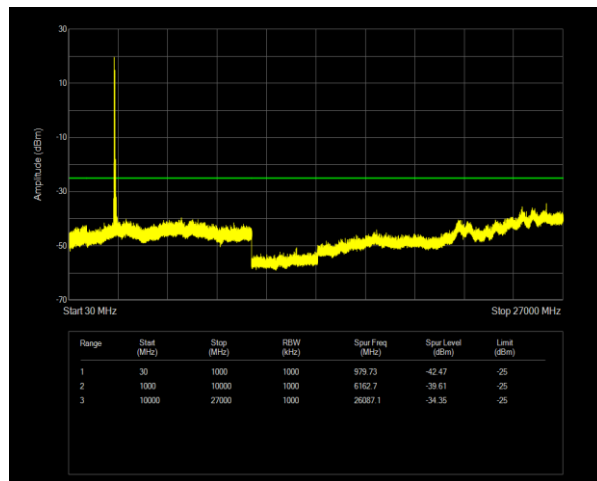
41C QPSK PCC BW=20MHz Ch=39750 RB=1@0,SCC BW=20MHz Ch=39948 RB=1@99
