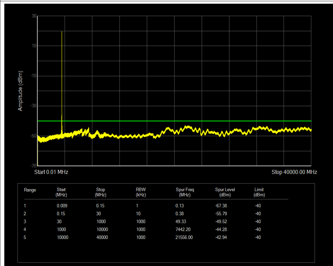
Band48 QPSK BW=10MHz Channel=55290 RB Size=1 Position=#0
