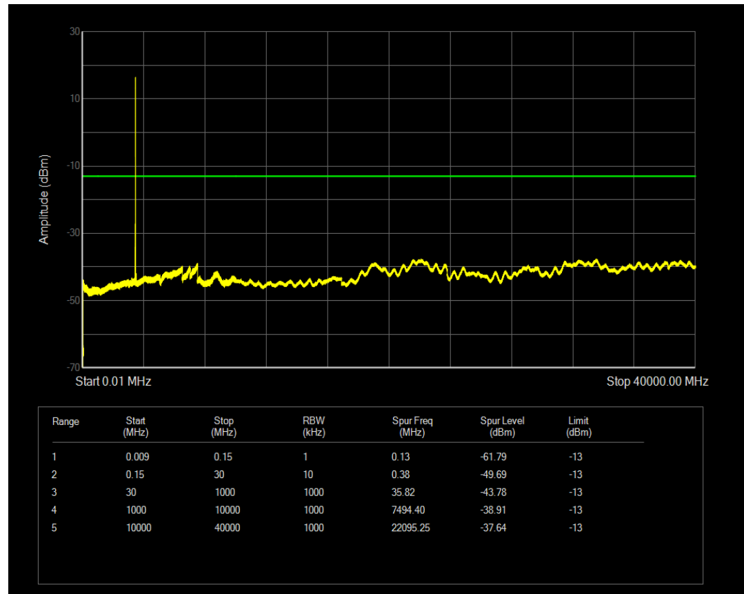
Band42(3450-3550) QPSK BW=15MHz Channel=42165 RB Size=1 Position=#0
