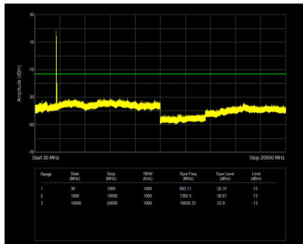
66C QPSK PCC BW=20MHz Ch=66536 RB=1@0,SCC BW=20MHz Ch=66734 RB=1@99
