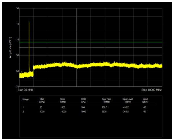
12B QPSK PCC BW=5MHz Ch=5038 RB=1@0,SCC BW=10MHz Ch=5110 RB=1@49
