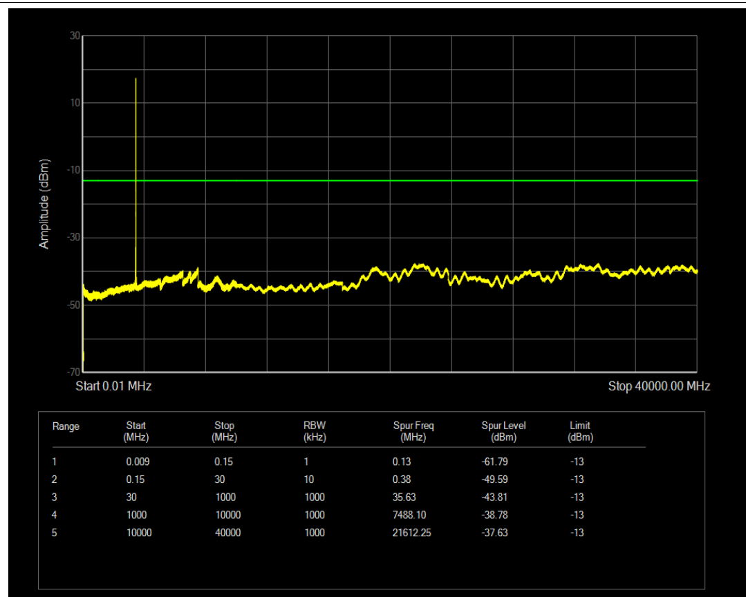
Band42(3450-3550) QPSK BW=10MHz Channel=42140 RB Size=1 Position=#0
