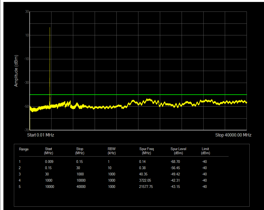
Band48 QPSK BW=5MHz Channel=56715 RB Size=1 Position=#0
