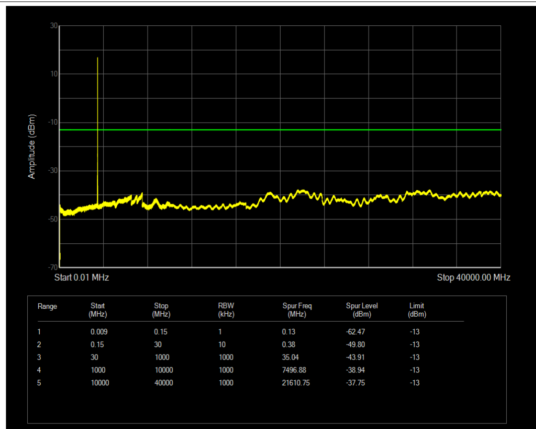
Band42(3450-3550) QPSK BW=20MHz Channel=42190 RB Size=1 Position=#0
