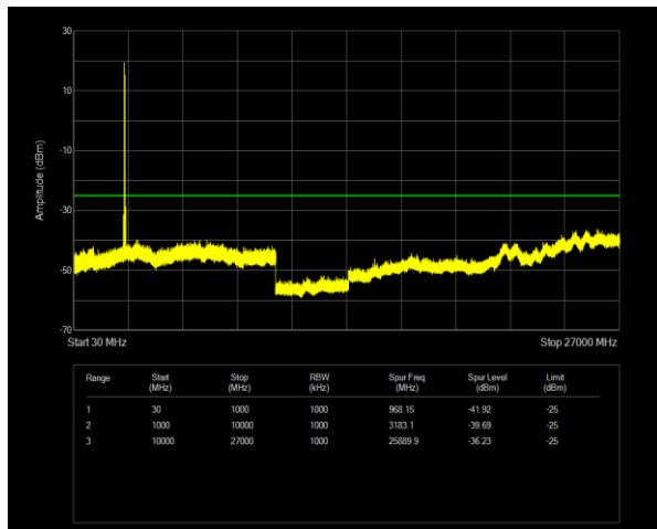
7C QPSK PCC BW=20MHz Ch=3001 RB=1@0,SCC BW=20MHz Ch=3199 RB=1@99
