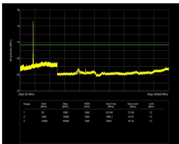
42C(3450-3550) QPSK PCC BW=20MHz Ch=42792 RB=1@0,SCC BW=20MHz Ch=42990 RB=1@99
