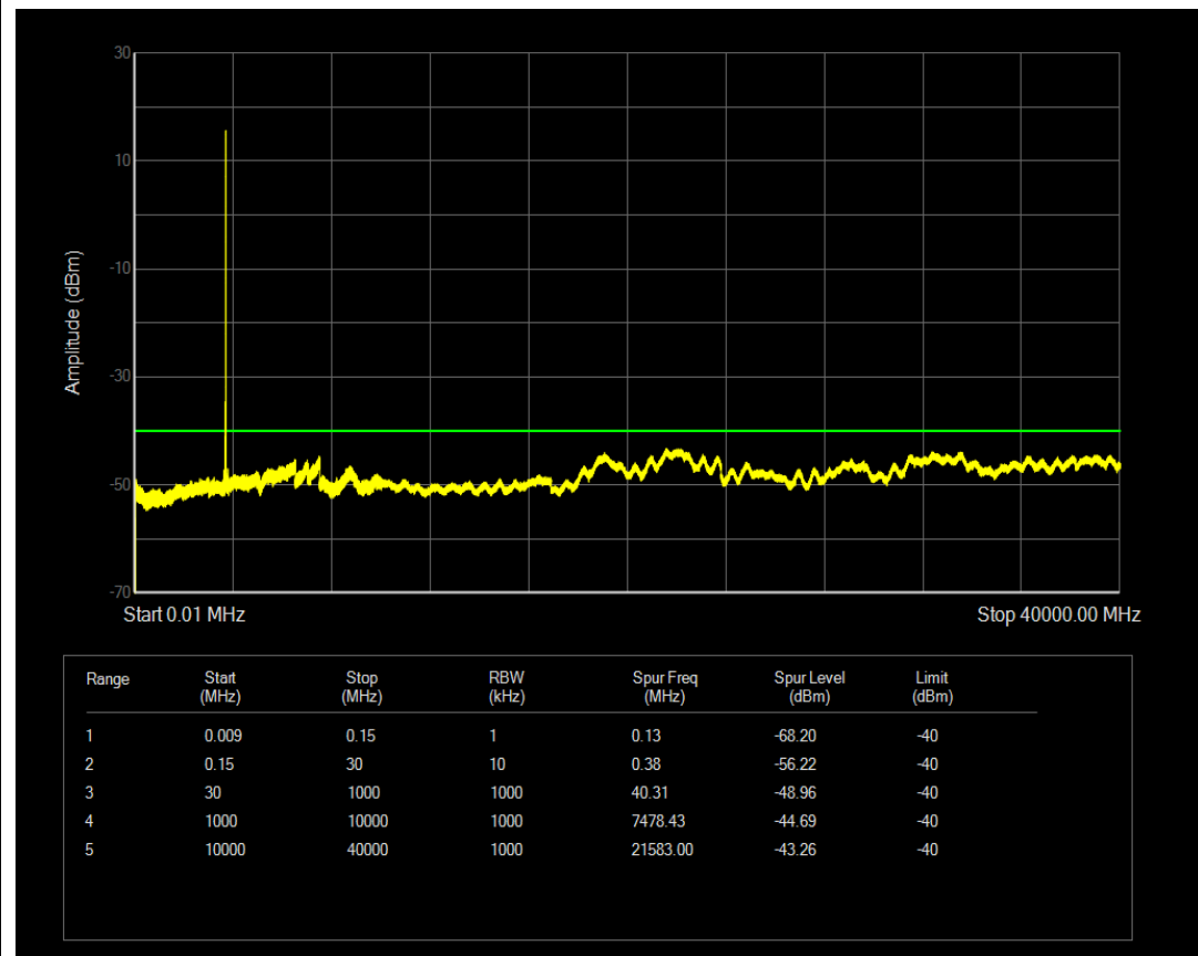
Band48 QPSK BW=15MHz Channel=56665 RB Size=1 Position=#0
