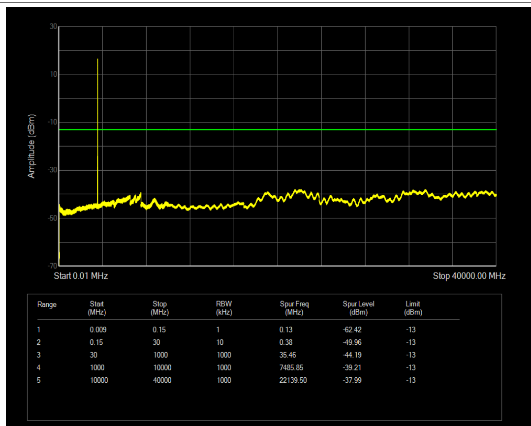
Band42(3450-3550) QPSK BW=20MHz Channel=42990 RB Size=1 Position=#0
