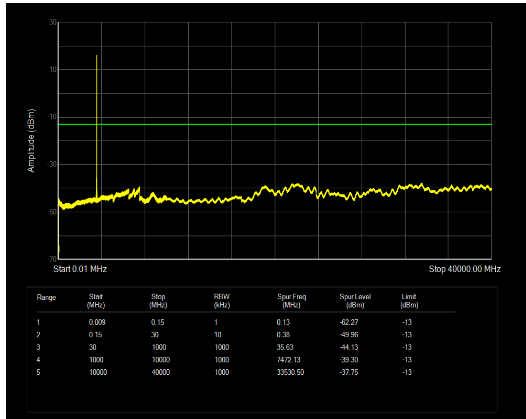
Band42(3450-3550) QPSK BW=15MHz Channel=43015 RB Size=1 Position=#0
