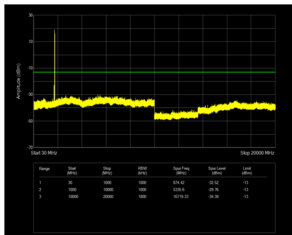
66C QPSK PCC BW=20MHz Ch=66838 RB=1@0,SCC BW=20MHz Ch=67036 RB=1@99
