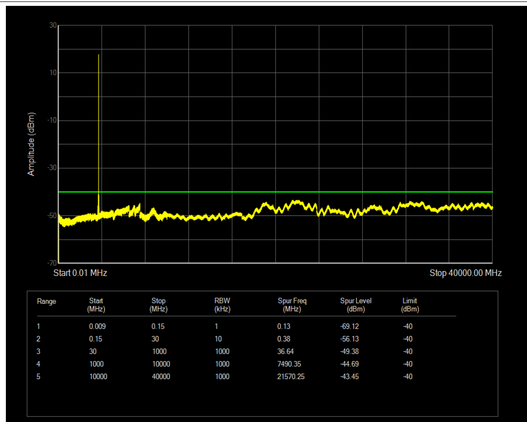
Band48 QPSK BW=10MHz Channel=56690 RB Size=1 Position=#0
