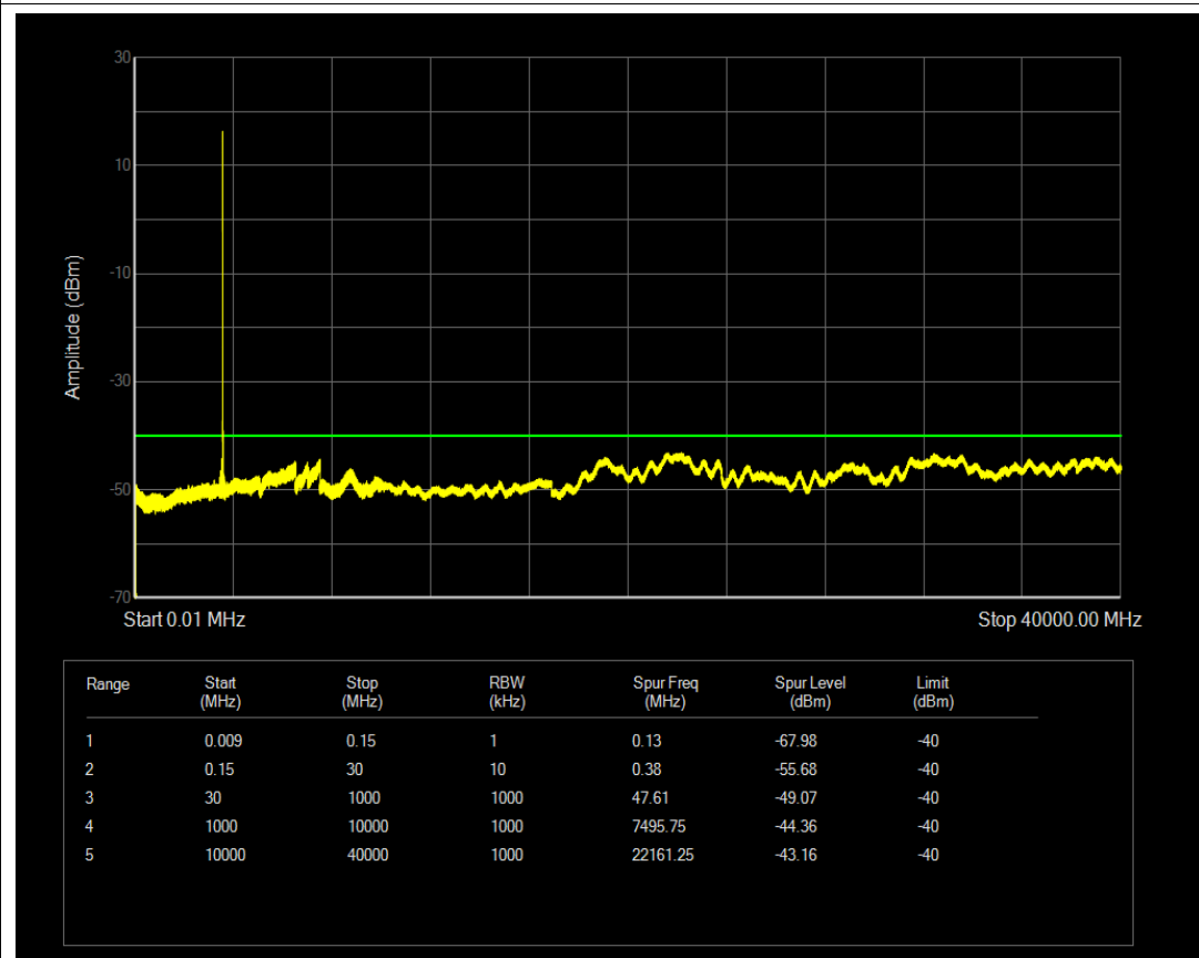
Band48 QPSK BW=20MHz Channel=55340 RB Size=1 Position=#0
