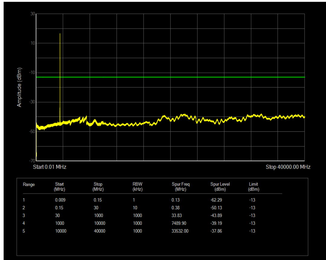
Band42(3450-3550) QPSK BW=5MHz Channel=43065 RB Size=1 Position=#0
