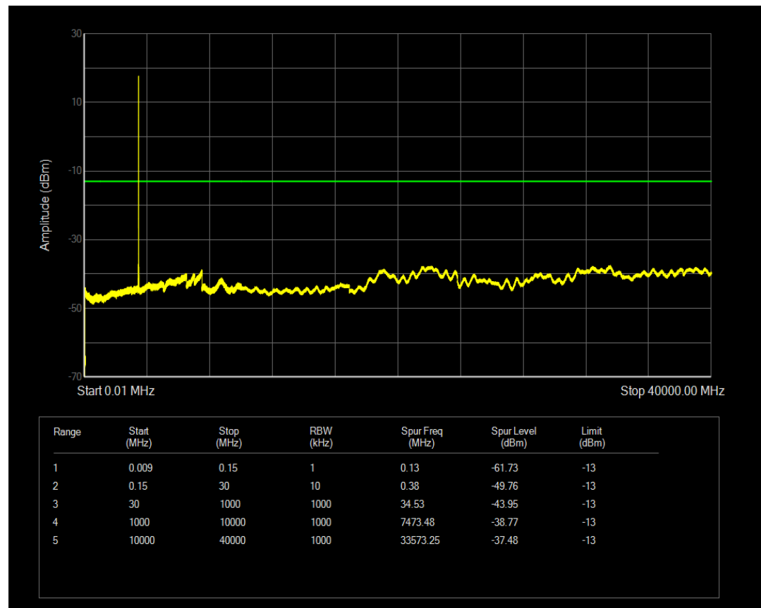
Band42(3450-3550) QPSK BW=5MHz Channel=42115 RB Size=1 Position=#0
