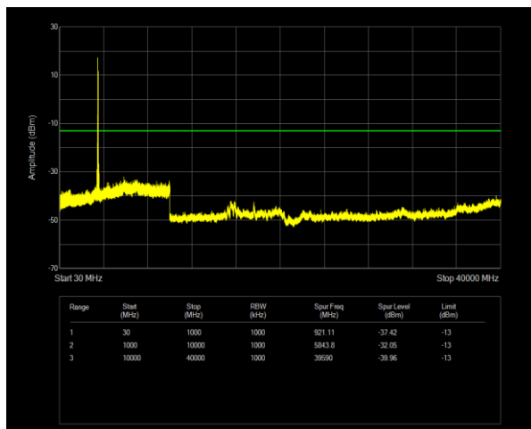
42C(3450-3550) QPSK PCC BW=20MHz Ch=42491 RB=1@0,SCC BW=20MHz Ch=42689 RB=1@99
