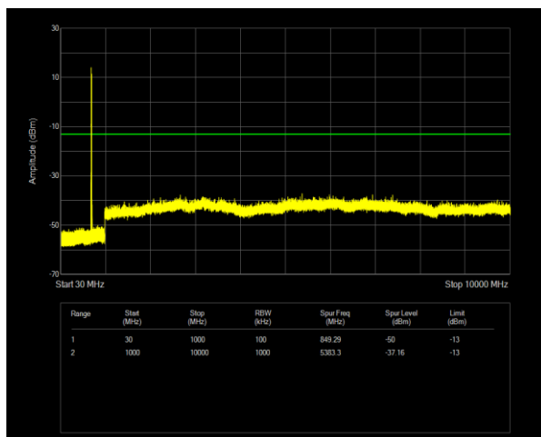
12B QPSK PCC BW=5MHz Ch=5058 RB=1@0,SCC BW=10MHz Ch=5130 RB=1@49
