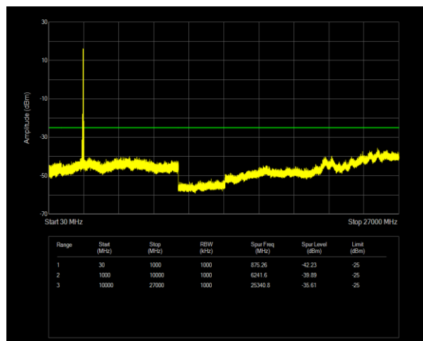
41C QPSK PCC BW=20MHz Ch=41292 RB=1@0,SCC BW=20MHz Ch=41490 RB=1@99
