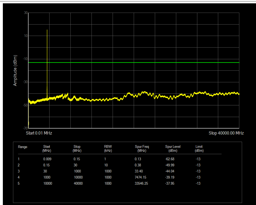
Band42(3450-3550) QPSK BW=10MHz Channel=43040 RB Size=1 Position=#0
