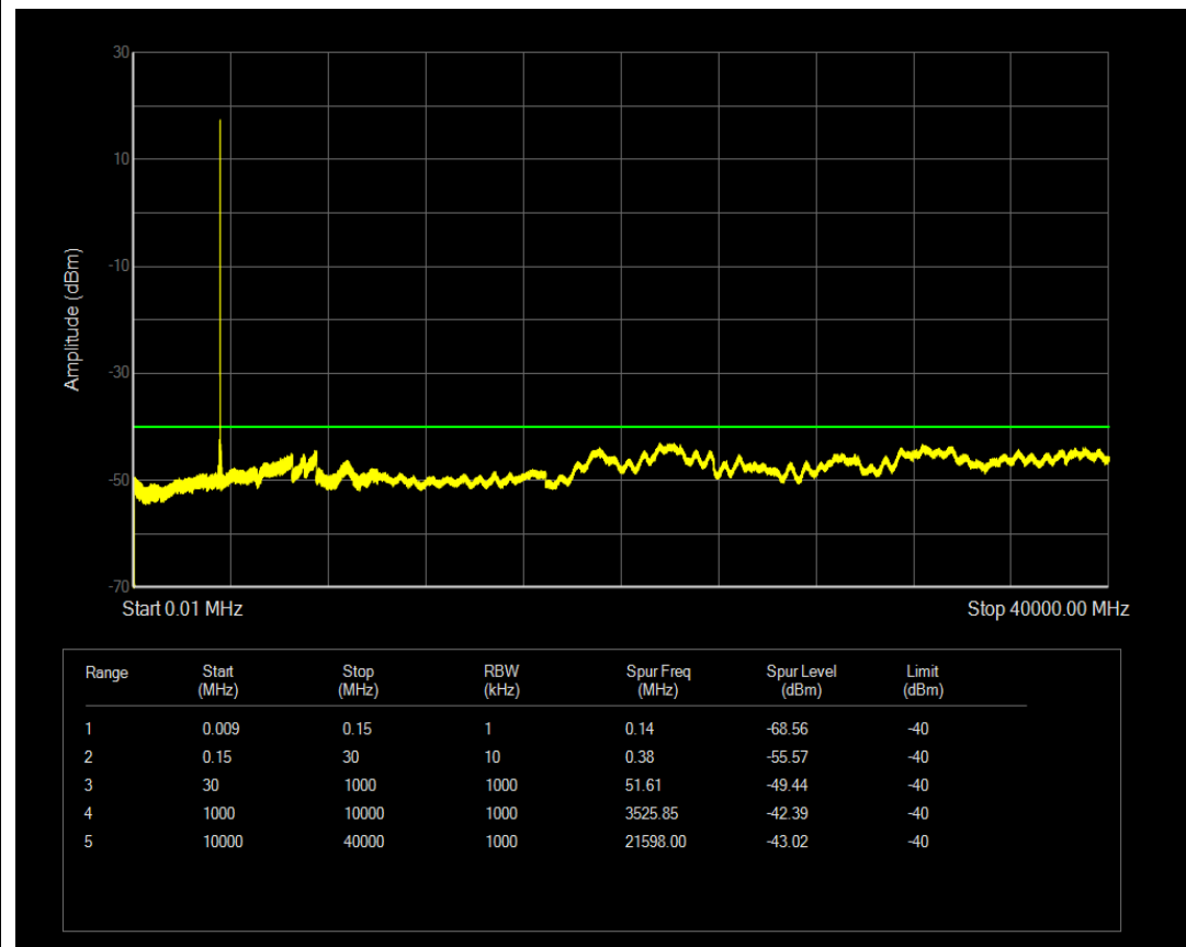
Band48 QPSK BW=5MHz Channel=55265 RB Size=1 Position=#0
