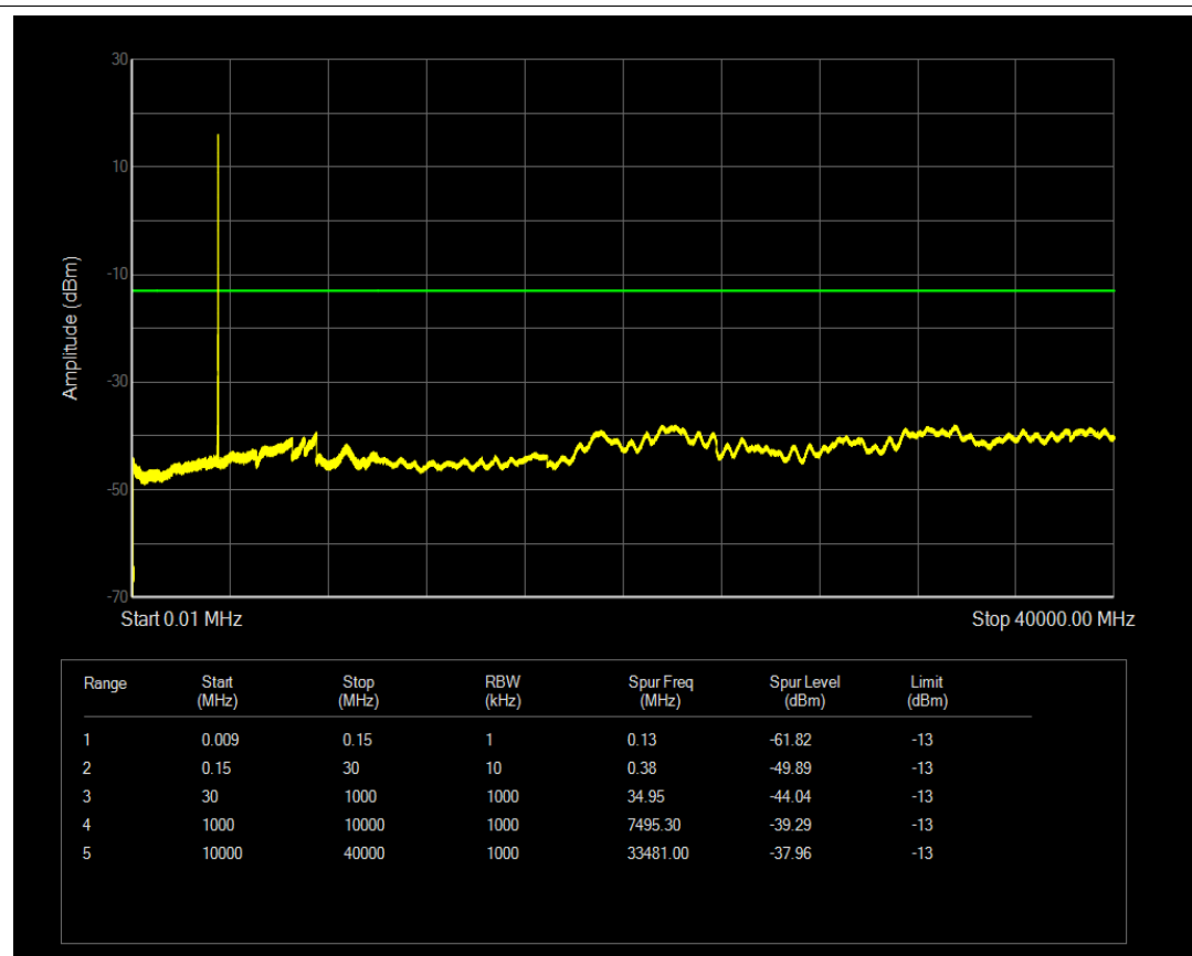
Band42(3450-3550) QPSK BW=15MHz Channel=42590 RB Size=1 Position=#0
