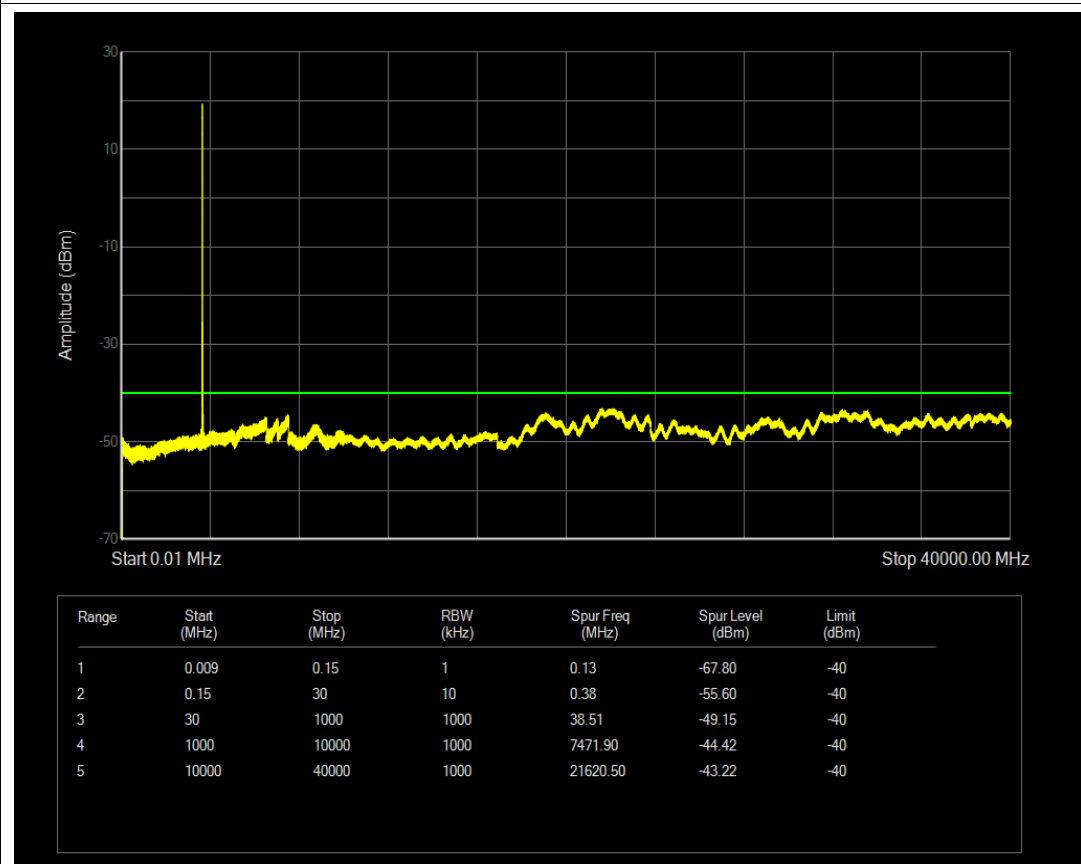
Band48 QPSK BW=5MHz Channel=55990 RB Size=1 Position=#0
