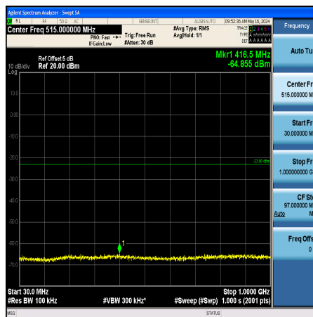
Band2_15MHz_QPSK_19125_1RB#0_30~1000_30~1000
