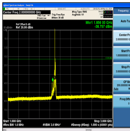
Band2_15MHz_QPSK_19125_1RB#0_1000~3000_1000~3000
