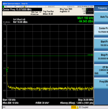
Band2_15MHz_QPSK_19125_1RB#0_0.15~30_0.15~30
