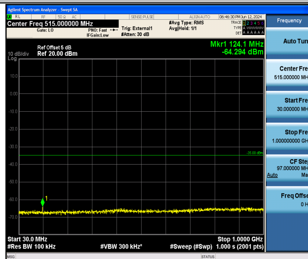
Band41_5MHz_QPSK_41565_1RB#0_30~1000_30~1000
