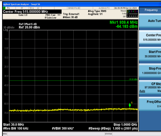
Band41_5MHz_QPSK_39675_1RB#0_30~1000_30~1000
