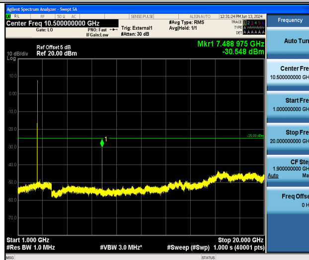
Band41_5MHz_QPSK_39675_1RB#0_1000~20000_1000~20000
