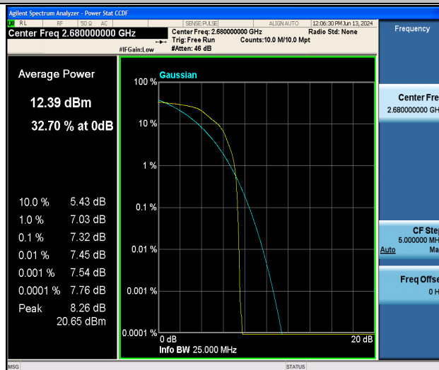
Band41-20MHz-16QAM-41490-1RB#0-PASS
