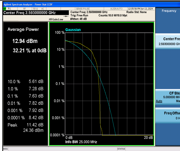
Band41-20MHz-16QAM-40620-1RB#0-PASS
