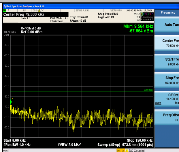
Band41_5MHz_16QAM_39675_1RB#0_0.009~0.15_0.009~0.15
