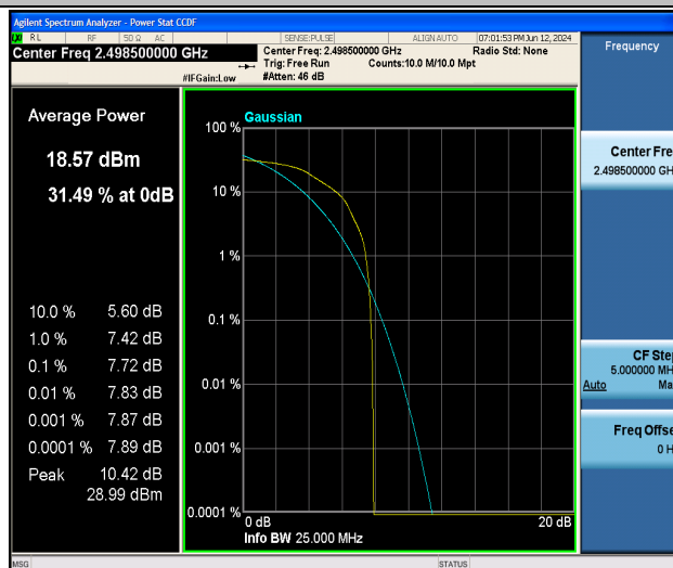
Band41-5MHz-16QAM-39675-1RB#0-PASS
