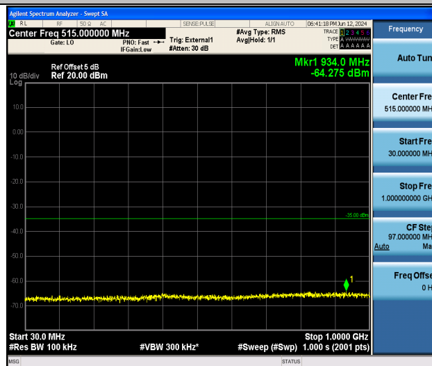
Band41_5MHz_16QAM_39675_1RB#0_30~1000_30~1000
