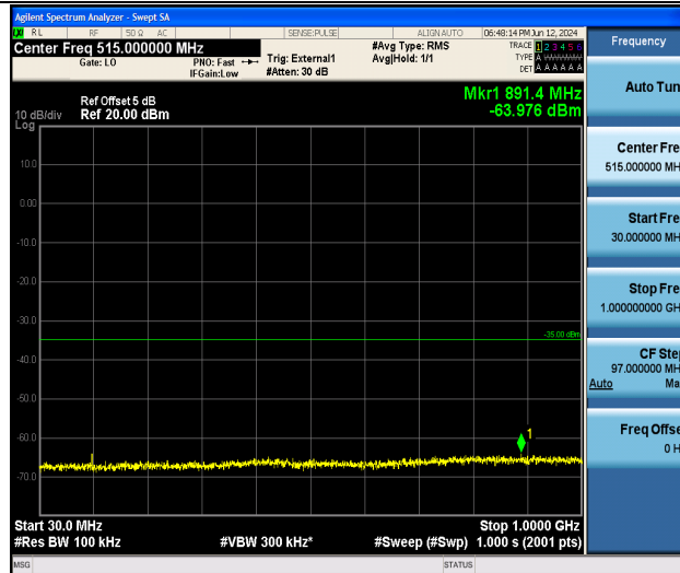
Band41_5MHz_16QAM_41565_1RB#0_30~1000_30~1000
