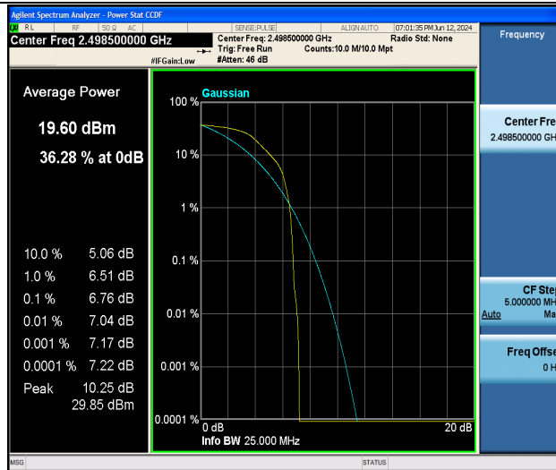
Band41-5MHz-QPSK-39675-1RB#0-PASS
