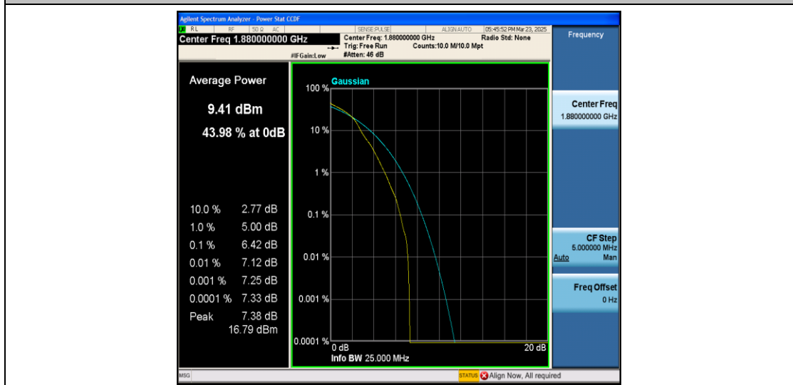
Band2-10MHz-16QAM-18900-1RB#0-PASS
