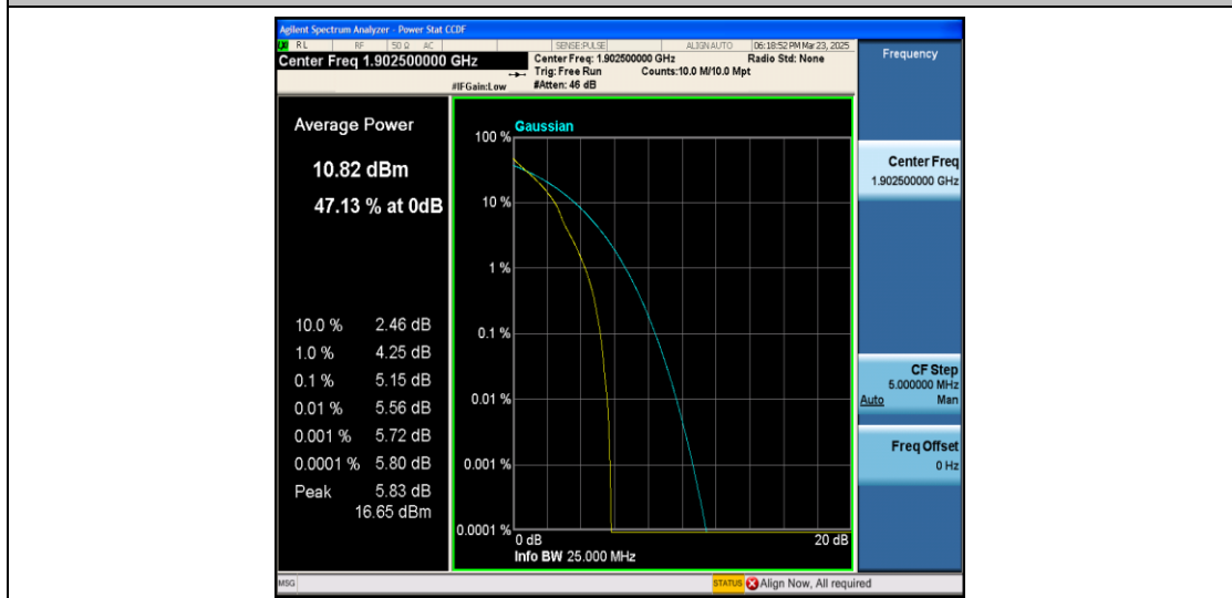
Band2-15MHz-QPSK-19125-1RB#0-PASS
