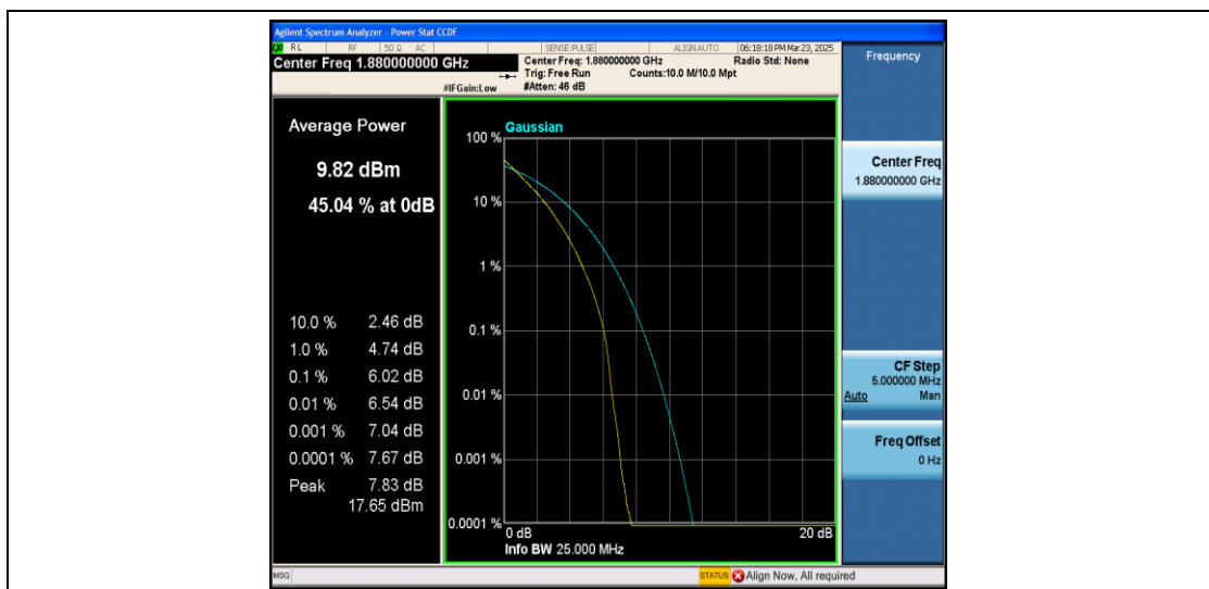
Band2-15MHz-QPSK-18900-75RB#0-PASS
