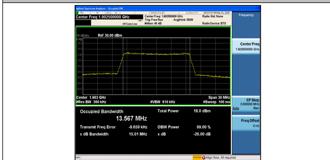
Band2-15MHz-16QAM-19125-75RB#0-PASS
