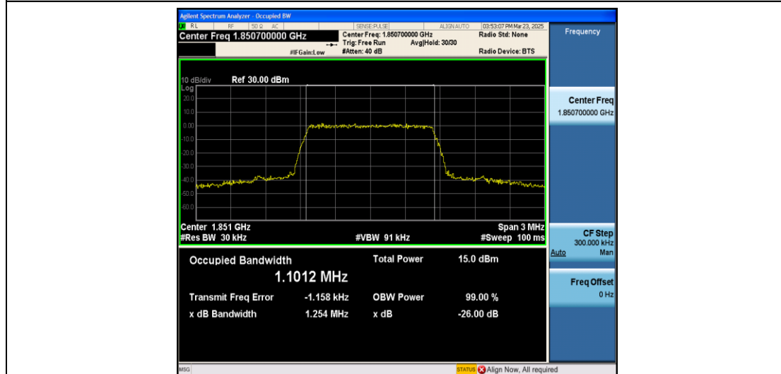
Band2-1.4MHz-16QAM-18607-6RB#0-PASS
