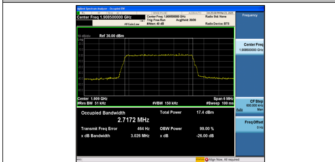
Band2-3MHz-QPSK-19185-15RB#0-PASS
