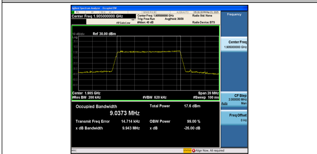
Band2-10MHz-16QAM-19150-50RB#0-PASS
