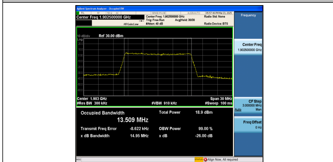
Band2-15MHz-QPSK-19125-75RB#0-PASS
