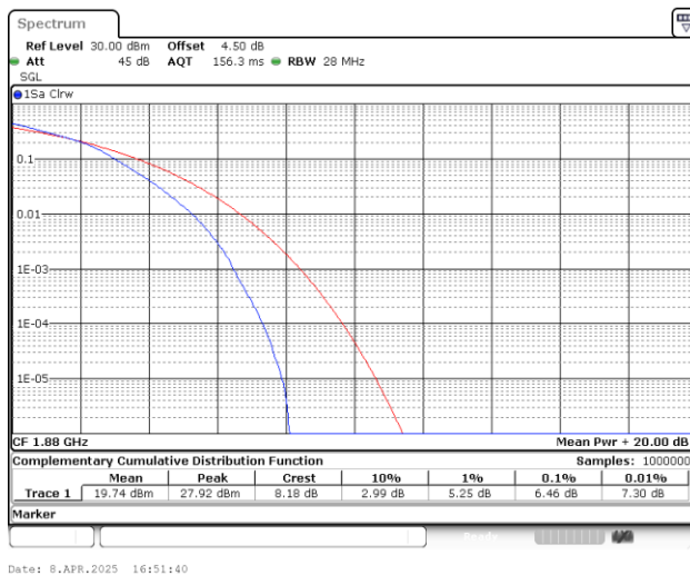
Band2-15MHz-16QAM-18900-75RB#0-PASS
