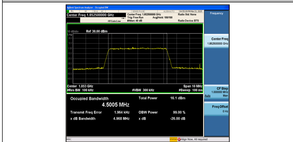
Band2-5MHz-16QAM-18625-25RB#0-PASS
