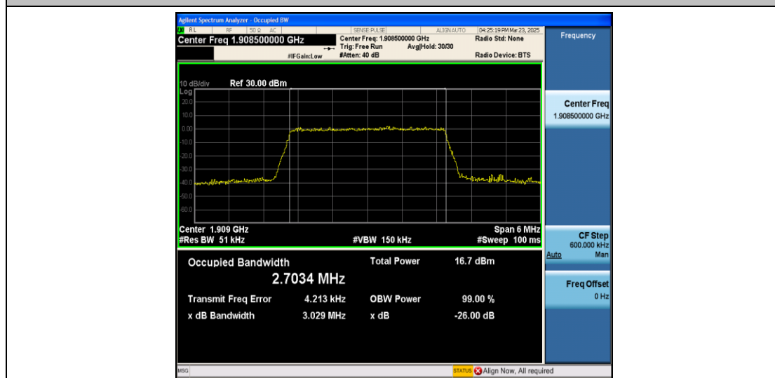
Band2-3MHz-16QAM-19185-15RB#0-PASS
