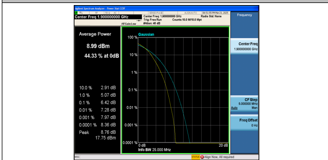
Band2-20MHz-16QAM-19100-100RB#0-PASS
