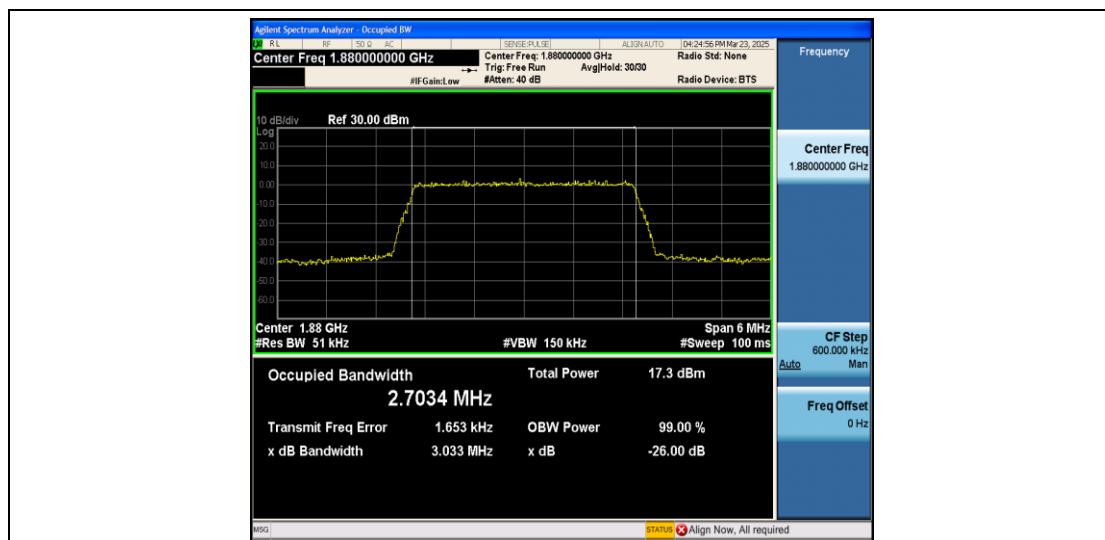
Band2-3MHz-16QAM-18900-15RB#0-PASS
