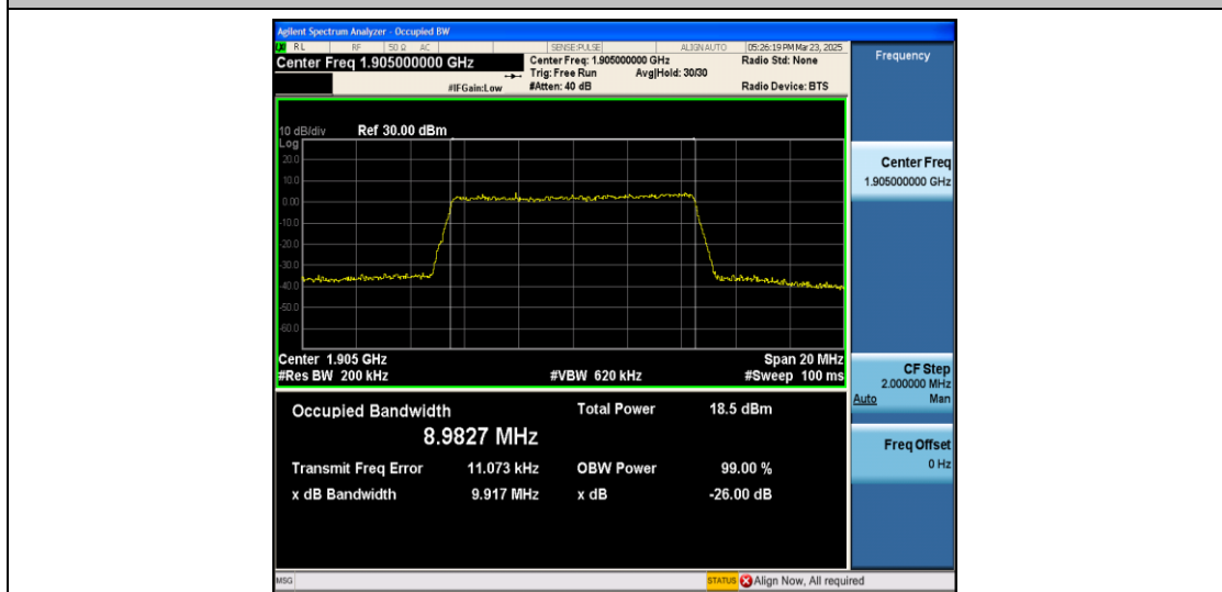
Band2-10MHz-QPSK-19150-50RB#0-PASS
