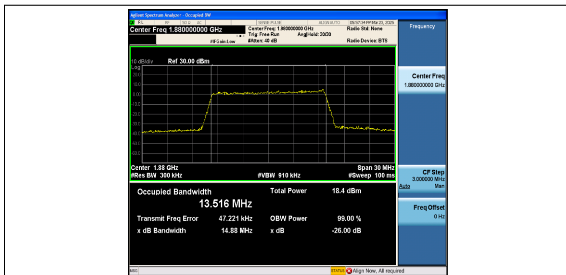
Band2-15MHz-16QAM-18900-75RB#0-PASS
