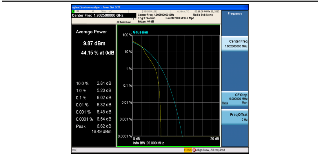
Band2-15MHz-16QAM-19125-1RB#0-PASS
