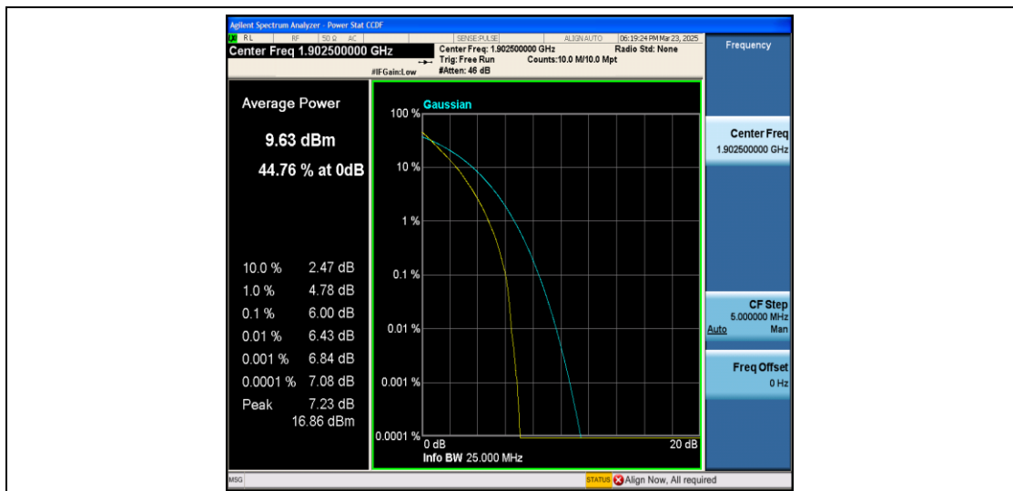
Band2-15MHz-QPSK-19125-75RB#0-PASS
