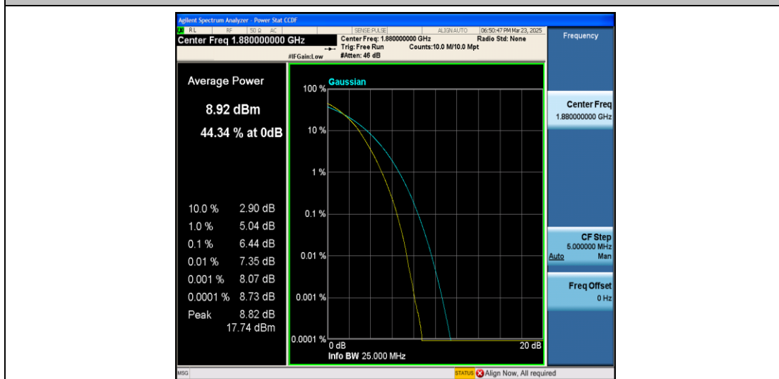
Band2-20MHz-16QAM-18900-100RB#0-PASS
