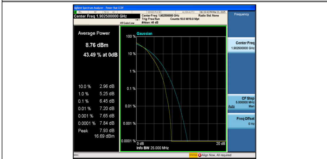
Band2-15MHz-16QAM-19125-75RB#0-PASS
