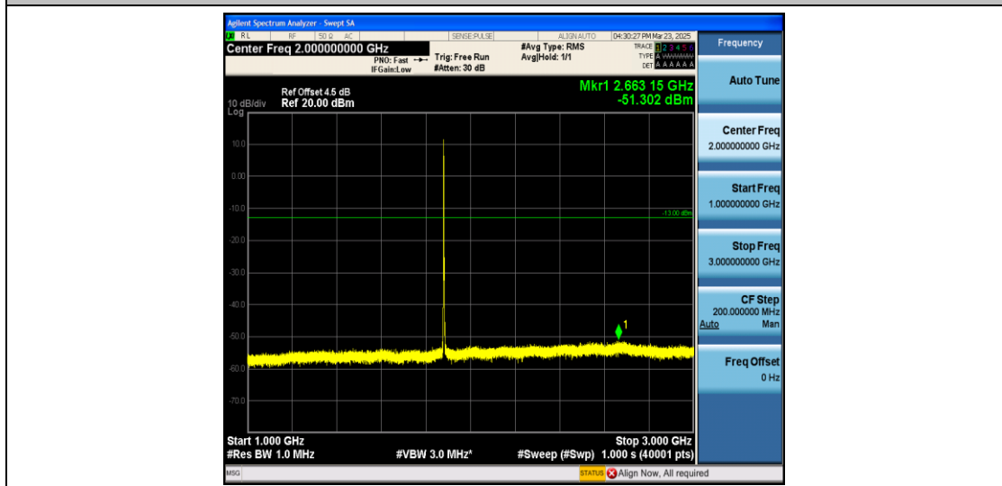
Band2_3MHz_QPSK_18900_1RB#0_1000~3000_1000~3000
