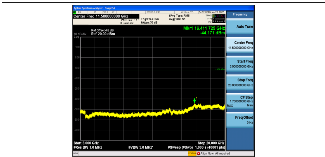
Band2_1.4MHz_16QAM_19193_1RB#0_3000~20000_3000~20000
