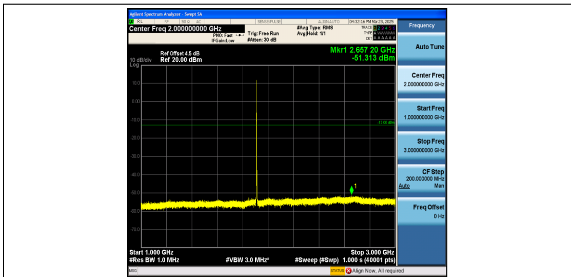
Band2_3MHz_QPSK_19185_1RB#0_1000~3000_1000~3000
