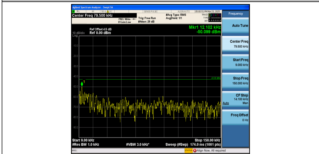
Band2_5MHz_QPSK_18900_1RB#0_0.009~0.15_0.009~0.15
