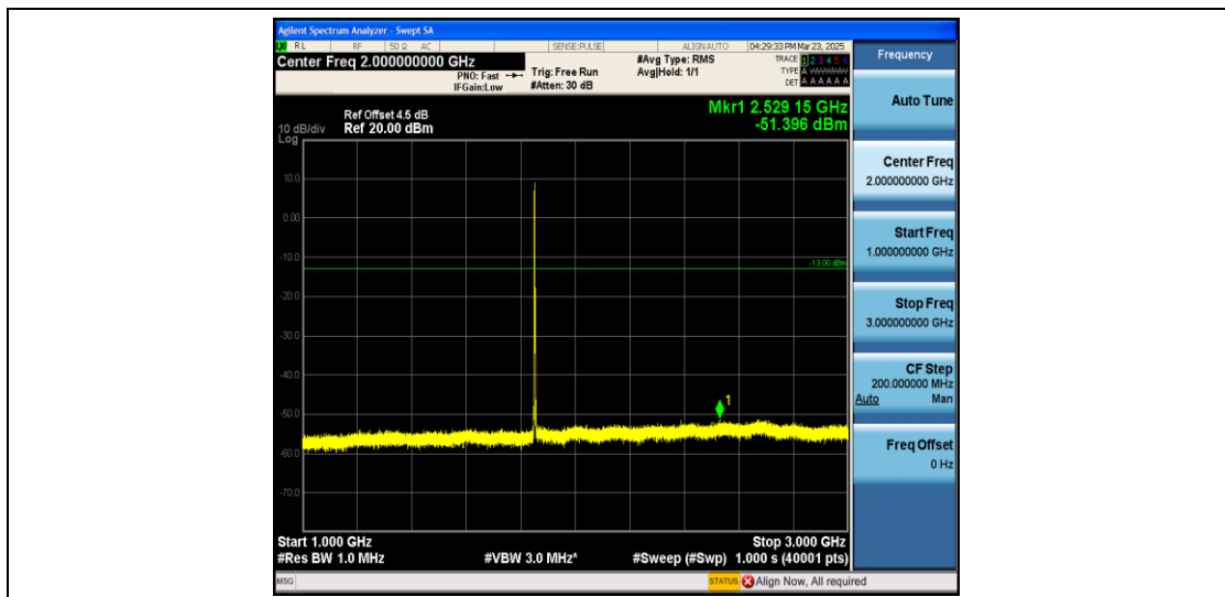
Band2_3MHz_16QAM_18615_1RB#0_1000~3000_1000~3000
