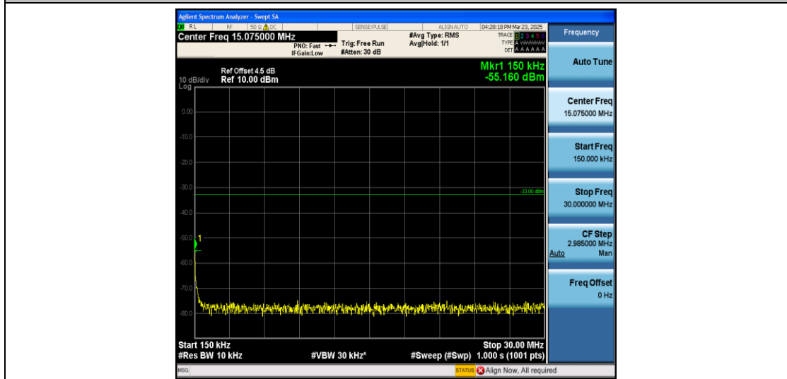
Band2_3MHz_QPSK_18615_1RB#0_0.15~30_0.15~30
