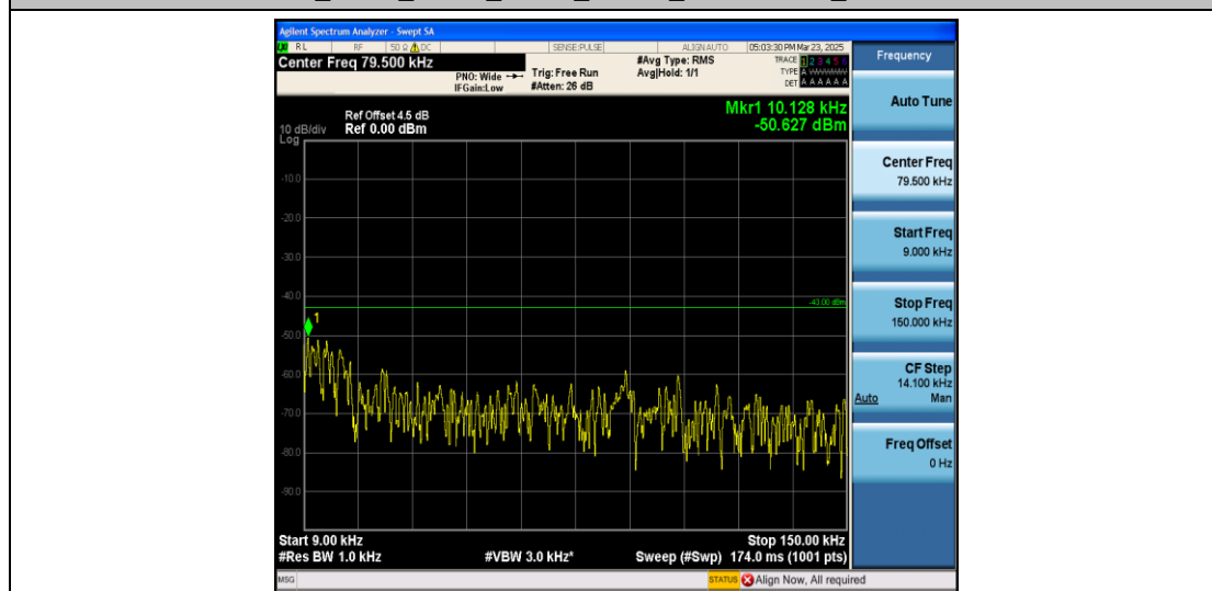
Band2_5MHz_16QAM_19175_1RB#0_0.009~0.15_0.009~0.15
