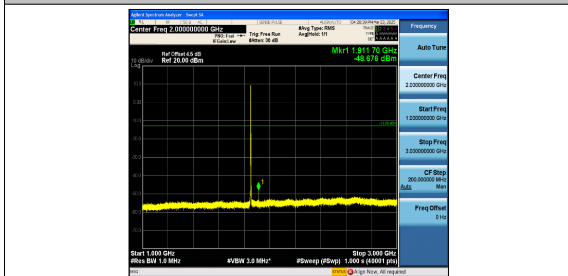
Band2_3MHz_QPSK_18615_1RB#0_1000~3000_1000~3000
