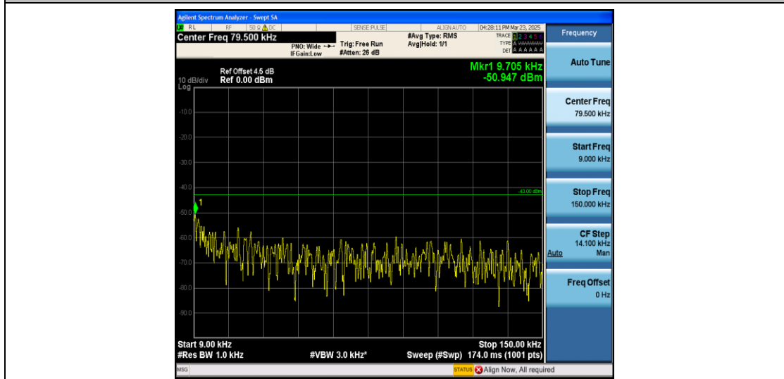
Band2_3MHz_QPSK_18615_1RB#0_0.009~0.15_0.009~0.15
