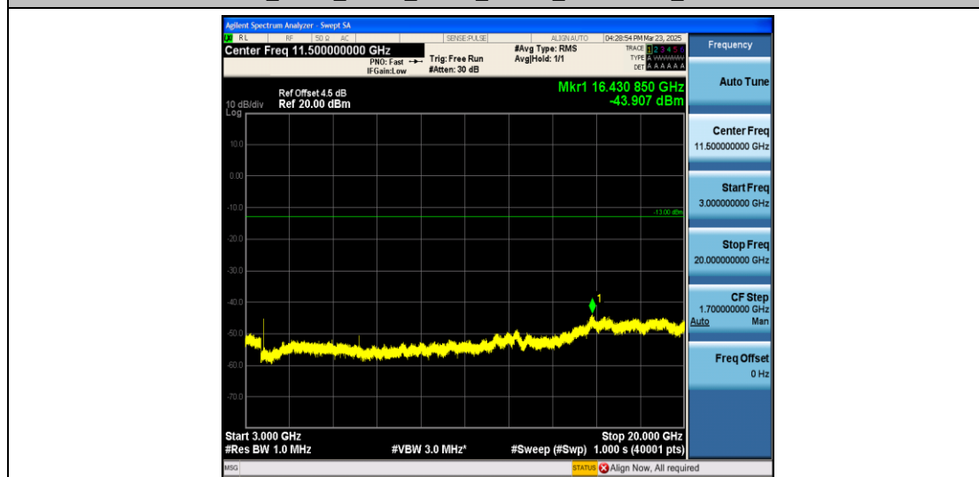
Band2_3MHz_QPSK_18615_1RB#0_3000~20000_3000~20000
