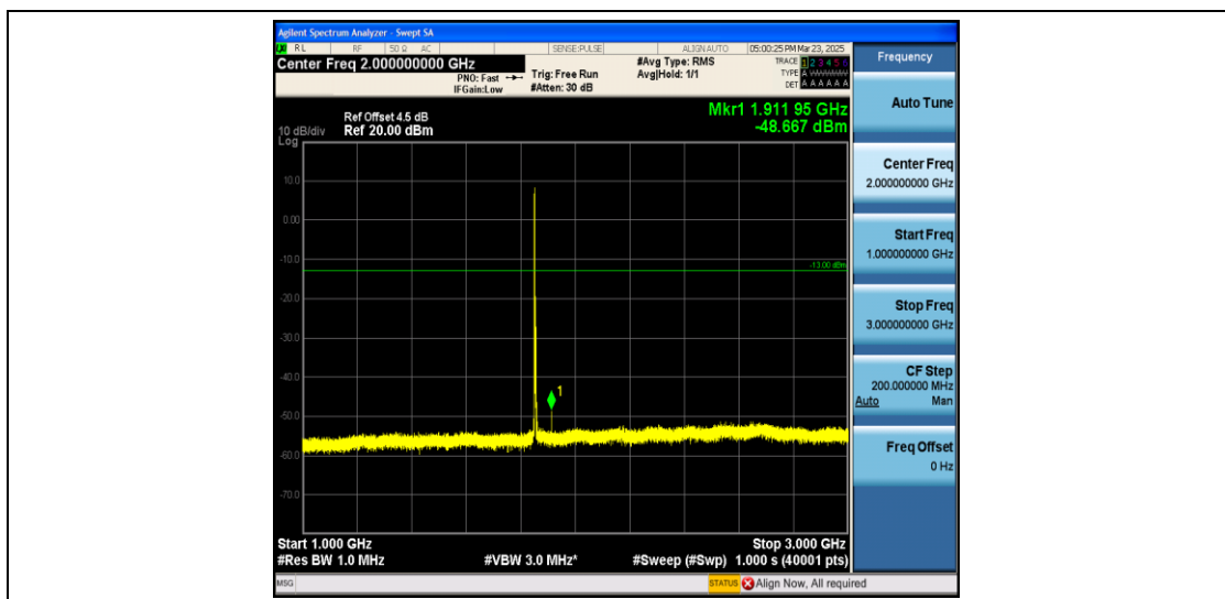
Band2_5MHz_16QAM_18625_1RB#0_1000~3000_1000~3000
