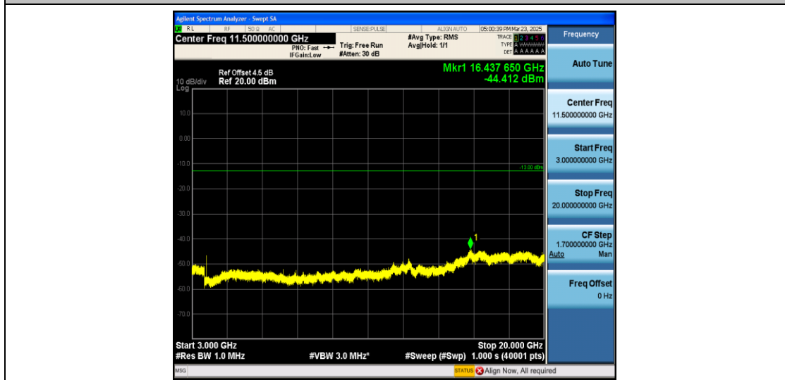
Band2_5MHz_16QAM_18625_1RB#0_3000~20000_3000~20000
