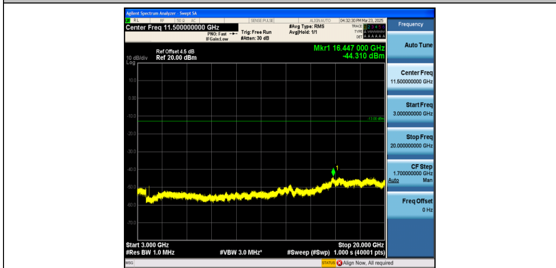
Band2_3MHz_QPSK_19185_1RB#0_3000~20000_3000~20000
