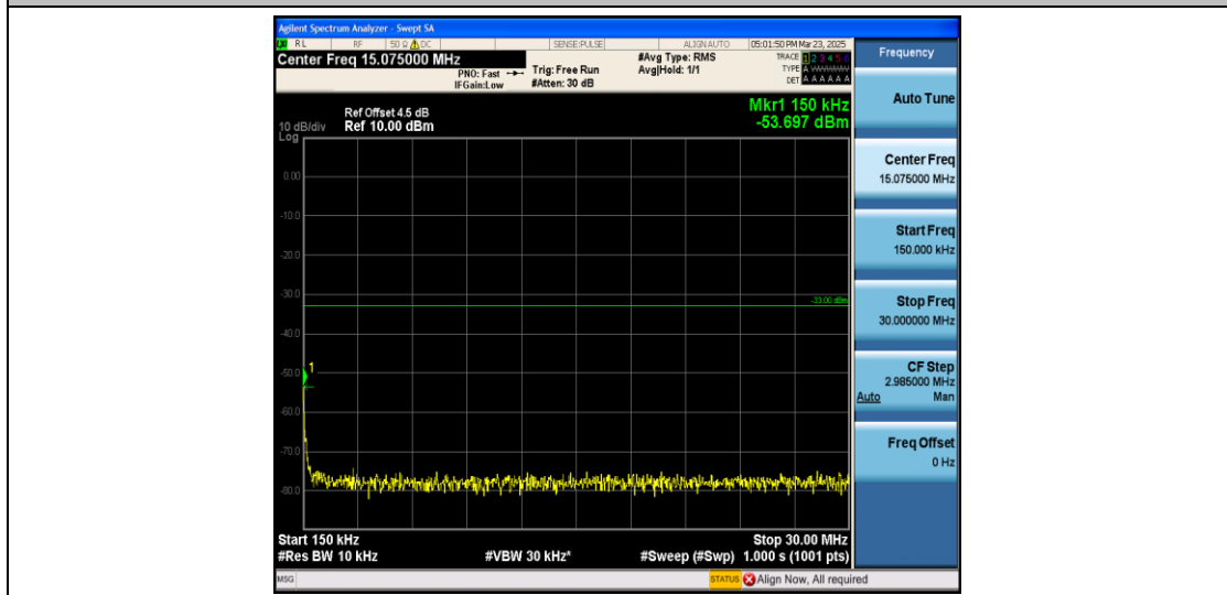
Band2_5MHz_16QAM_18900_1RB#0_0.15~30_0.15~30
