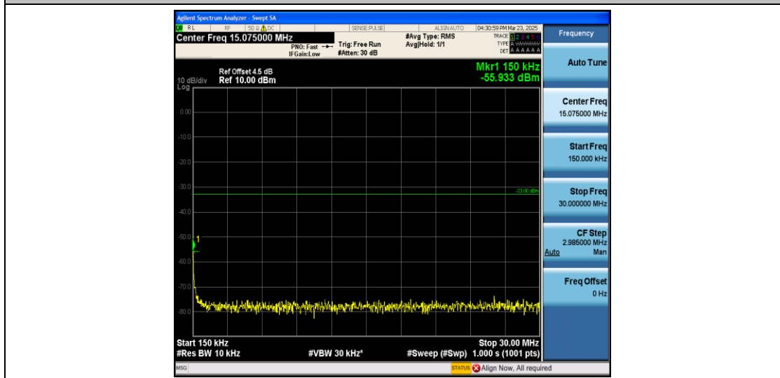
Band2_3MHz_16QAM_18900_1RB#0_0.15~30_0.15~30
