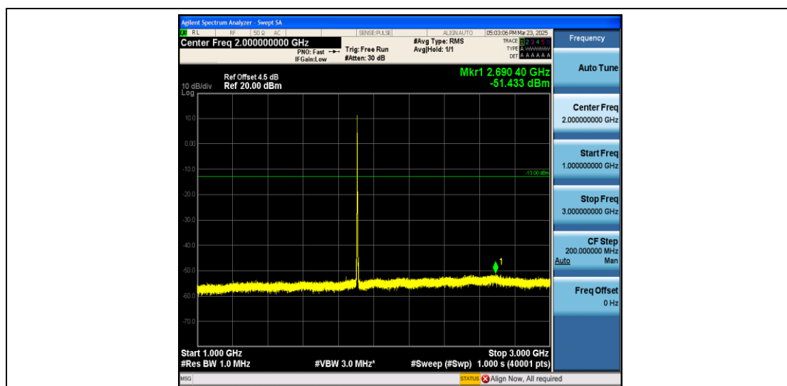
Band2_5MHz_QPSK_19175_1RB#0_1000~3000_1000~3000
