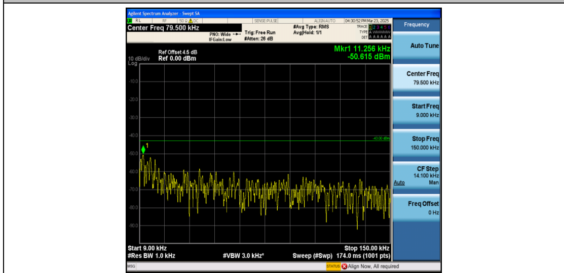
Band2_3MHz_16QAM_18900_1RB#0_0.009~0.15_0.009~0.15
