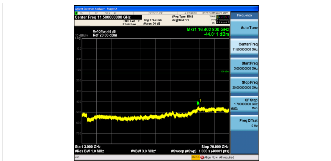
Band2_5MHz_QPSK_18900_1RB#0_3000~20000_3000~20000
