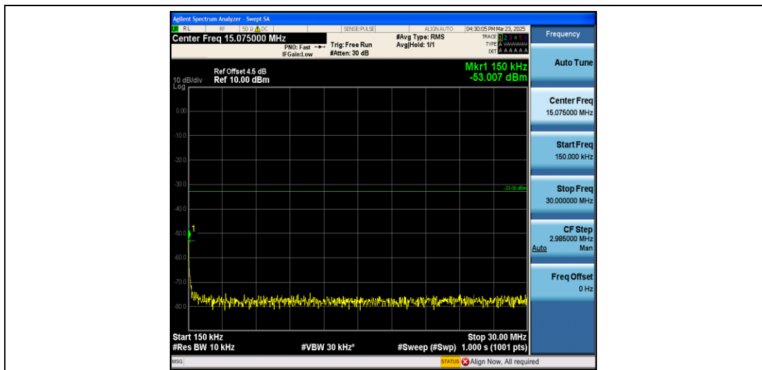
Band2_3MHz_QPSK_18900_1RB#0_0.15~30_0.15~30
