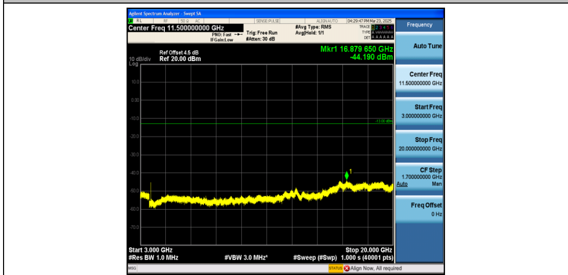
Band2_3MHz_16QAM_18615_1RB#0_3000~20000_3000~20000
