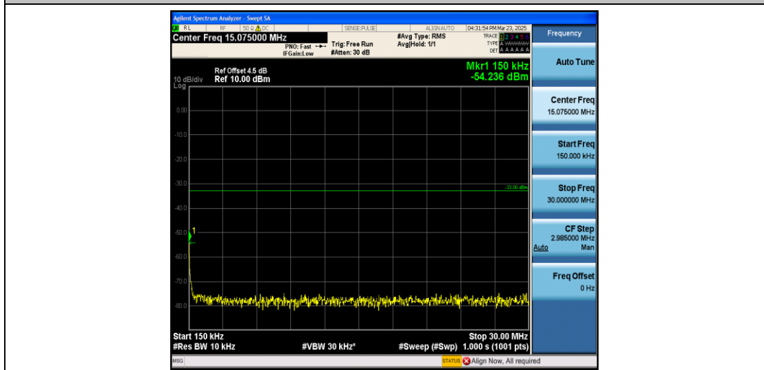
Band2_3MHz_QPSK_19185_1RB#0_0.15~30_0.15~30
