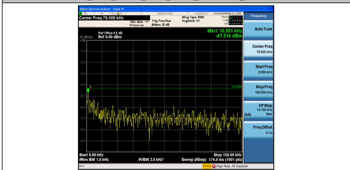
Band2_3MHz_QPSK_18900_1RB#0_0.009~0.15_0.009~0.15
