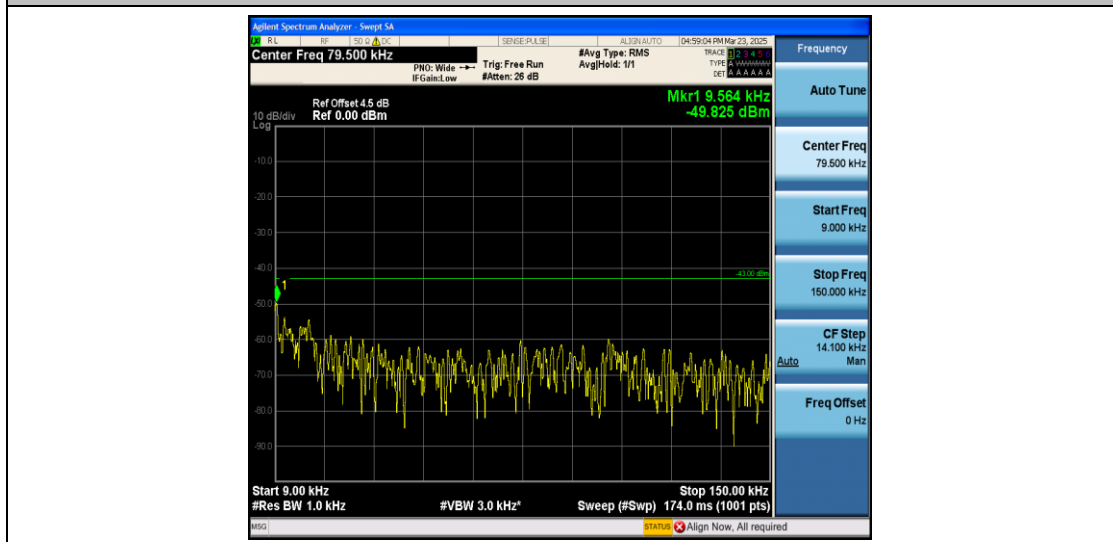
Band2_5MHz_QPSK_18625_1RB#0_0.009~0.15_0.009~0.15
