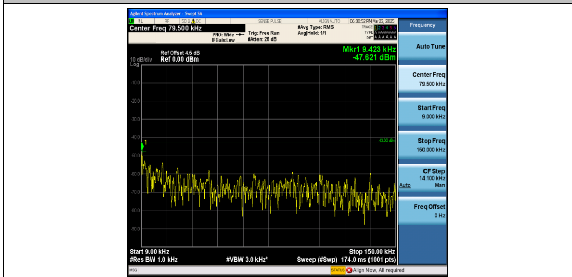
Band2_15MHz_QPSK_18675_1RB#0_0.009~0.15_0.009~0.15
