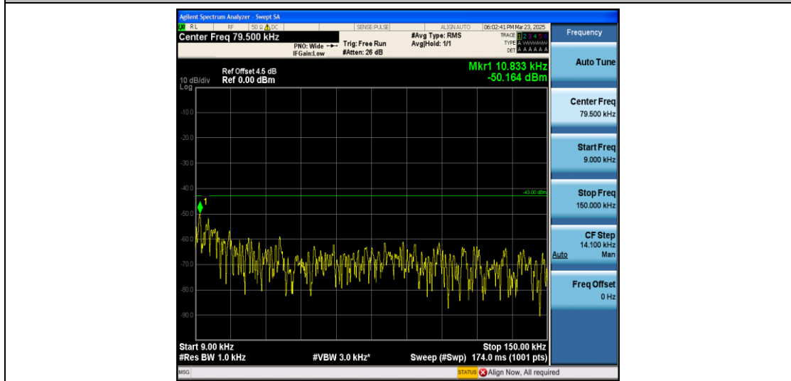
Band2_15MHz_QPSK_18900_1RB#0_0.009~0.15_0.009~0.15
