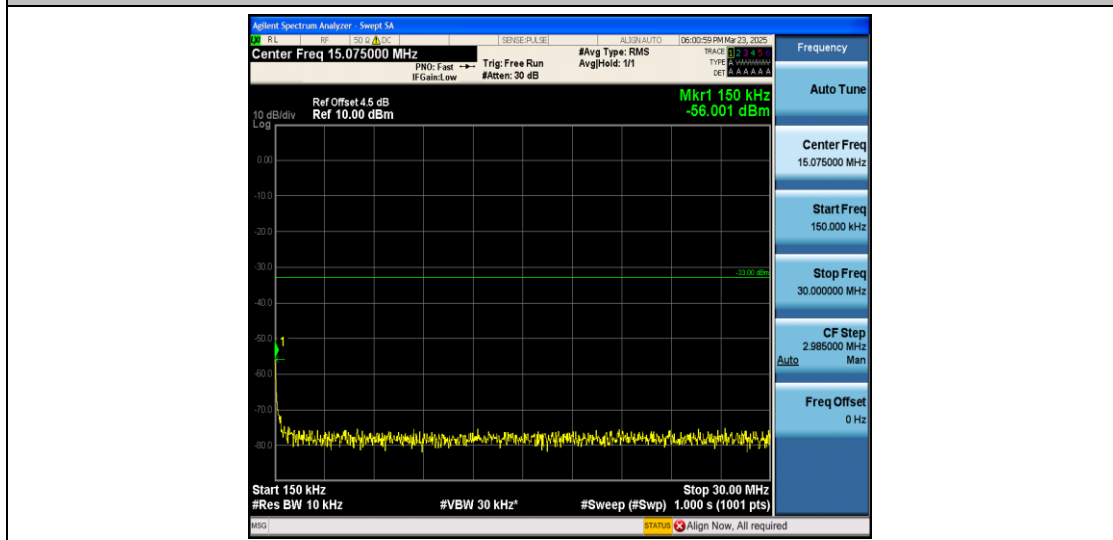
Band2_15MHz_QPSK_18675_1RB#0_0.15~30_0.15~30
