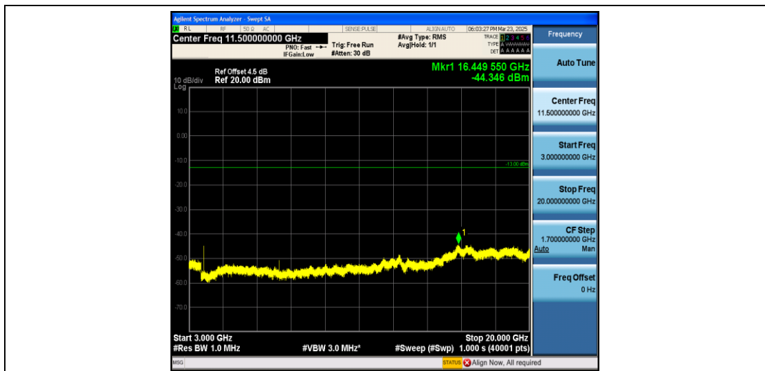
Band2_15MHz_QPSK_18900_1RB#0_3000~20000_3000~20000
