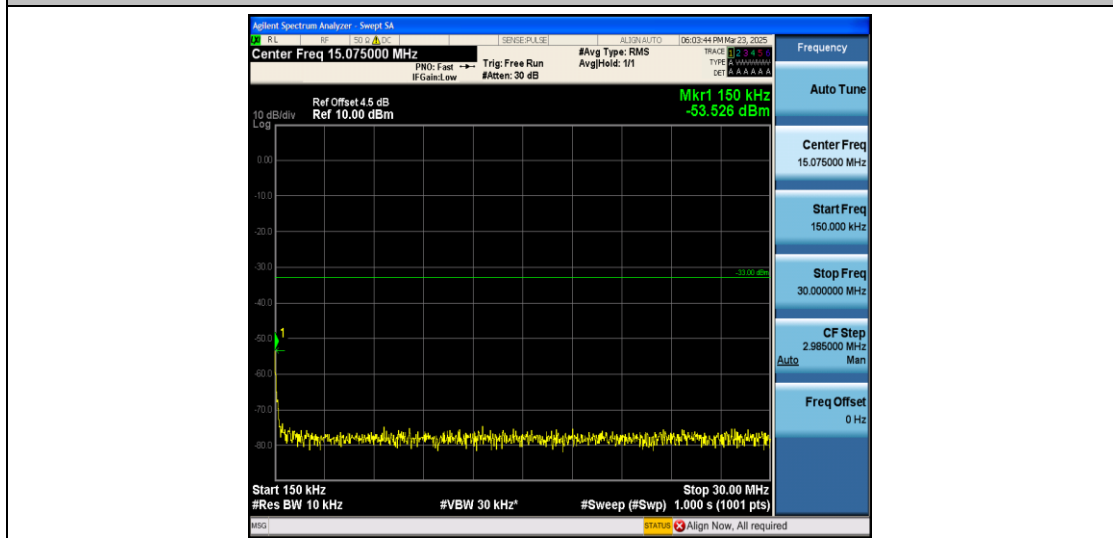
Band2_15MHz_16QAM_18900_1RB#0_0.15~30_0.15~30
