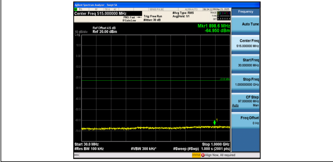
Band2_20MHz_16QAM_18700_1RB#0_30~1000_30~1000
