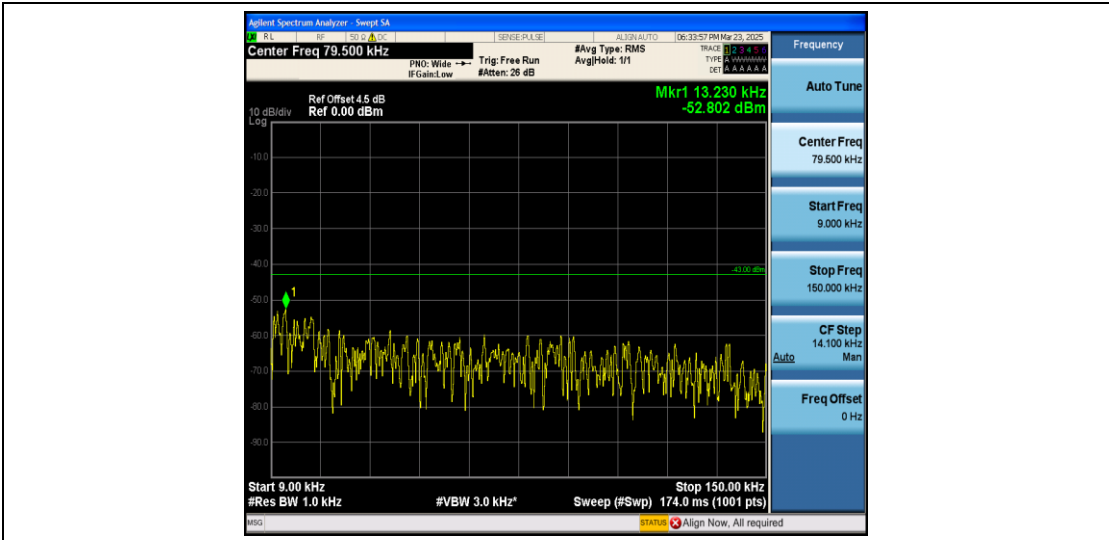
Band2_20MHz_16QAM_18700_1RB#0_0.009~0.15_0.009~0.15
