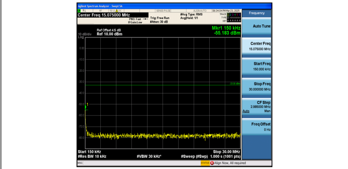
Band2_20MHz_16QAM_18700_1RB#0_0.15~30_0.15~30
