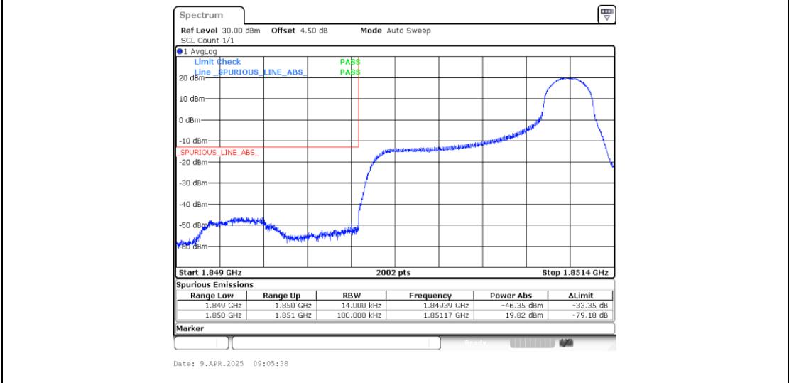
Band25_1.4MHz_16QAM_26047_1RB#5
