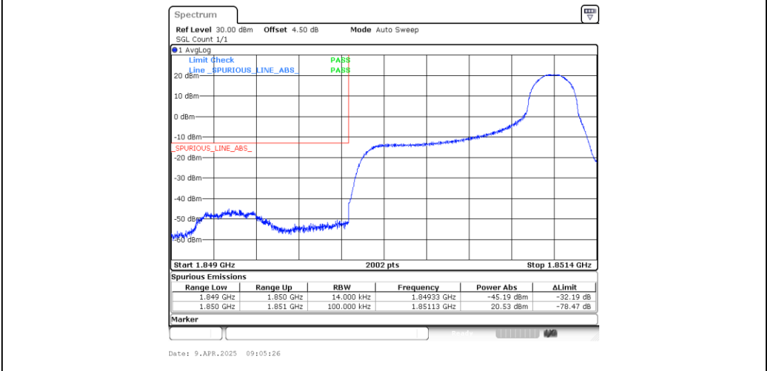
Band25_1.4MHz_QPSK_26047_1RB#5
