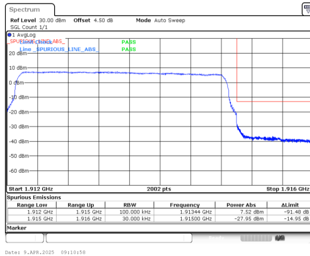
Band25_3MHz_16QAM_26675_15RB#0
