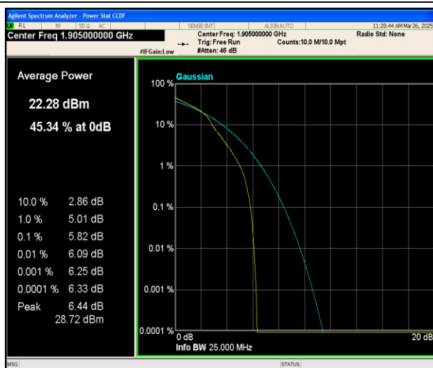
Band25-20MHz-16QAM-26590-1RB#0-PASS
