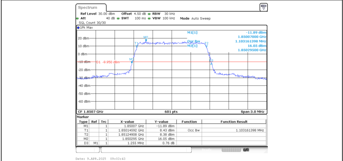
Band25-1.4MHz-16QAM-26047-6RB#0-PASS
