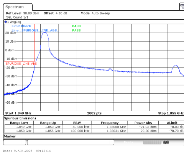
Band25_5MHz_QPSK_26065_1RB#0
