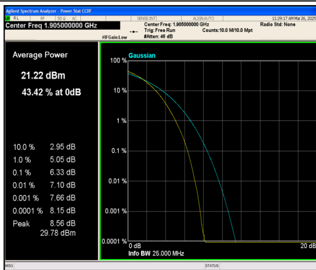
Band25-20MHz-16QAM-26590-100RB#0-PASS
