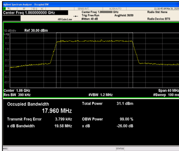
Band25-20MHz-QPSK-26140-100RB#0-PASS
