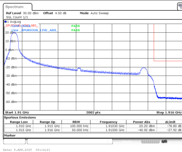
Band25_5MHz_QPSK_26665_1RB#0
