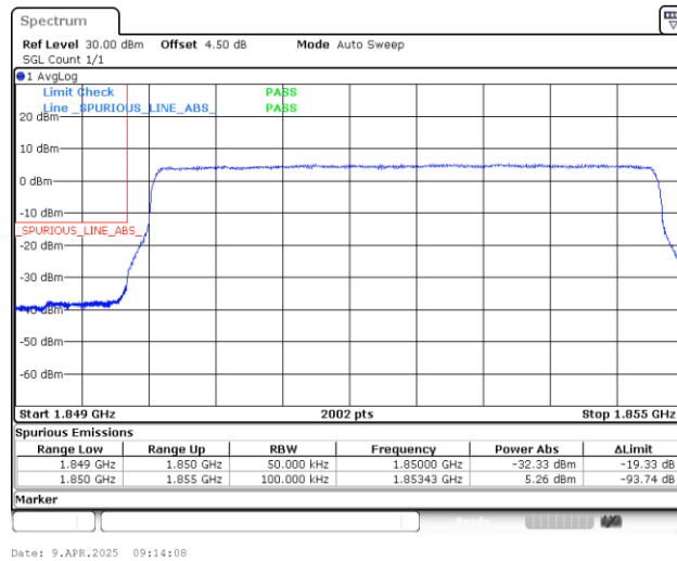
Band25_5MHz_16QAM_26065_25RB#0
