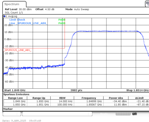
Band25_1.4MHz_QPSK_26047_6RB#0
