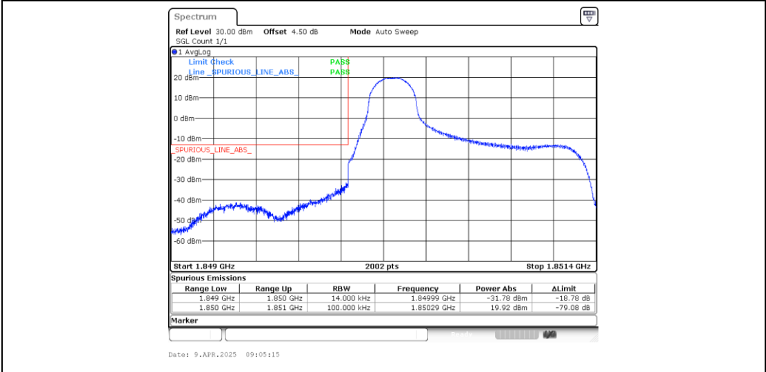
Band25_1.4MHz_16QAM_26047_1RB#0
