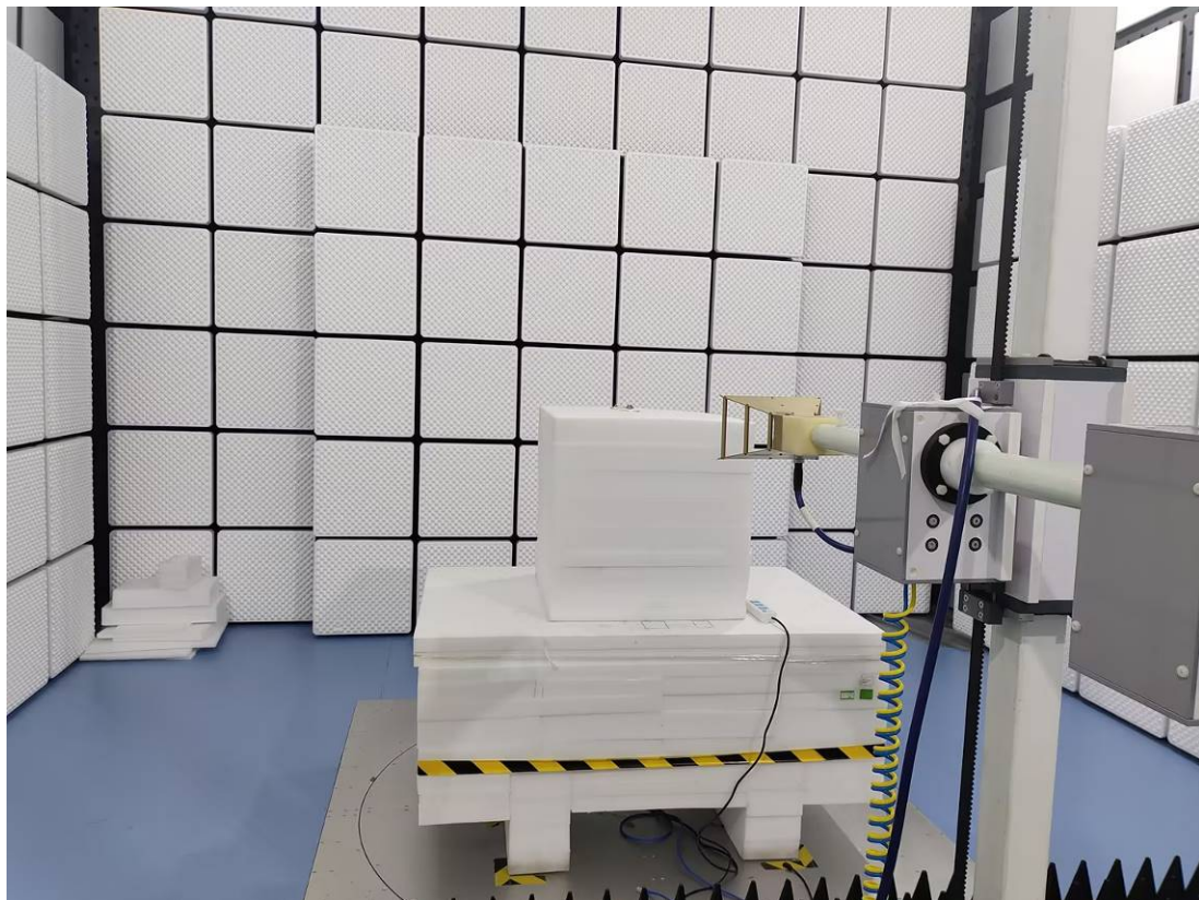
RE-Back View (3 GHz-18 GHz)
