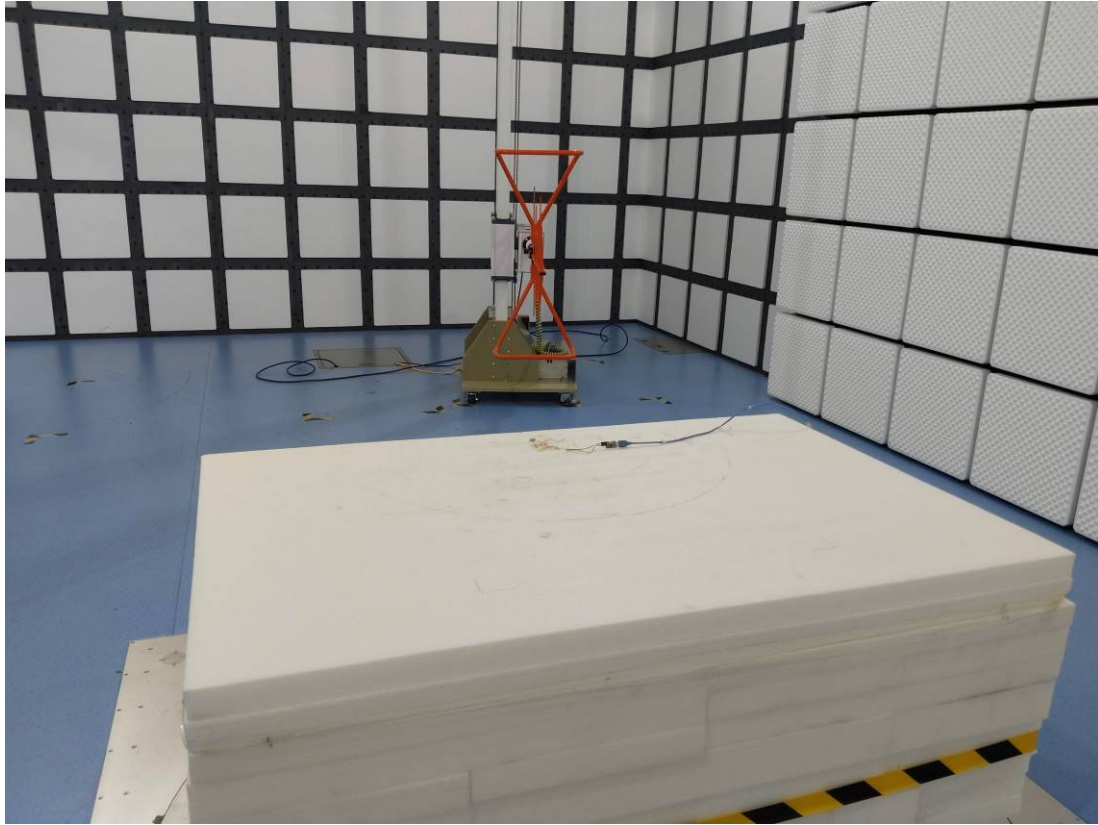
RE-Back View(30MHz~1GHz)
