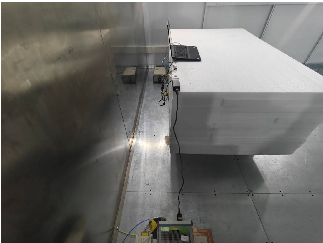
CE-Side View
