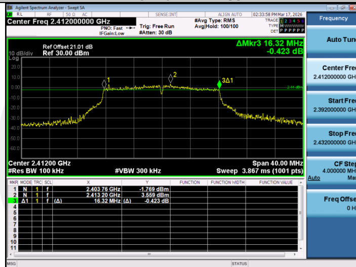
11G-Ant2-2412-PASS
