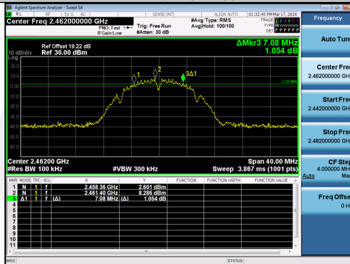
11B-Ant1-2462-PASS
