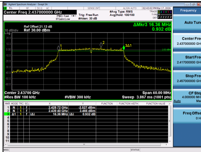
11G-Ant2-2437-PASS
