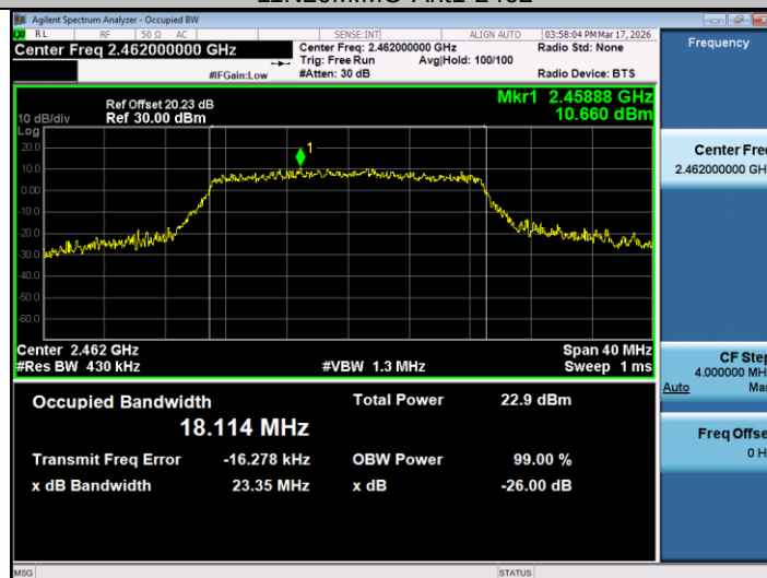
11N20MIMO-Ant2-2462
