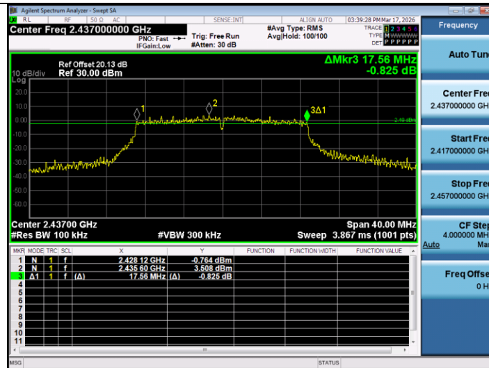
11N20MIMO-Ant2-2437-PASS
