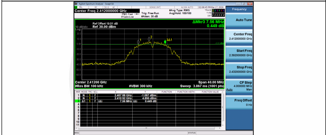
11B-Ant2-2412-PASS
