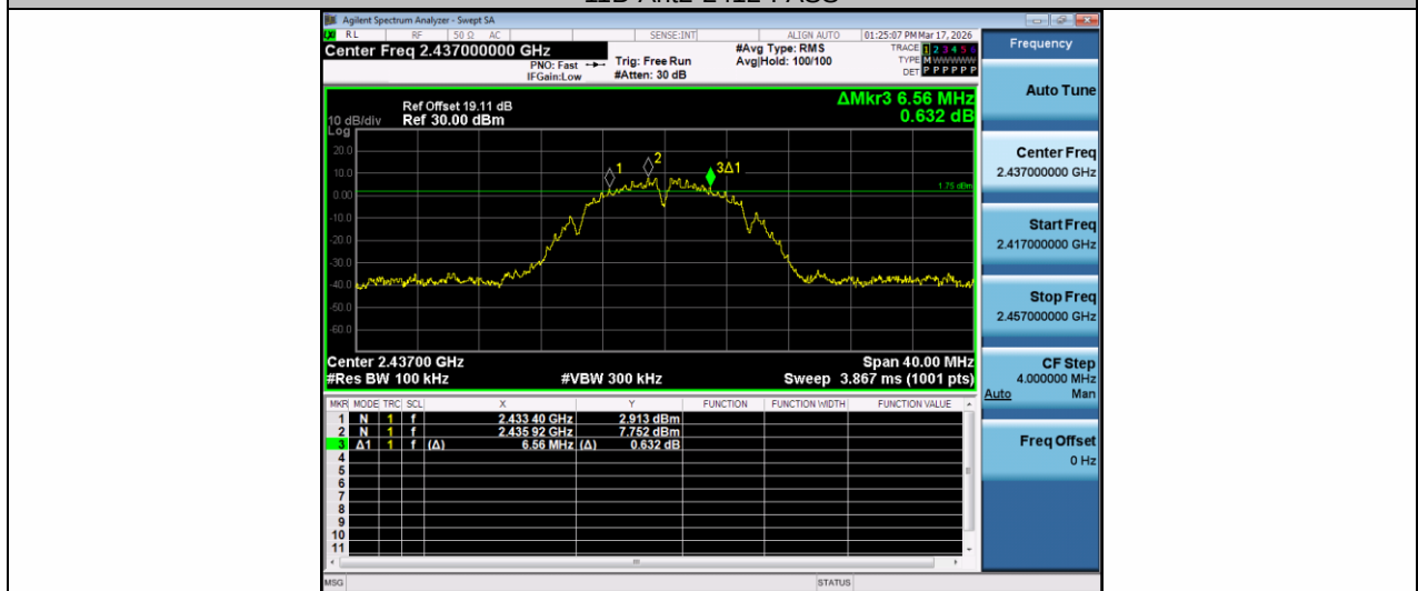
11B-Ant1-2437-PASS
