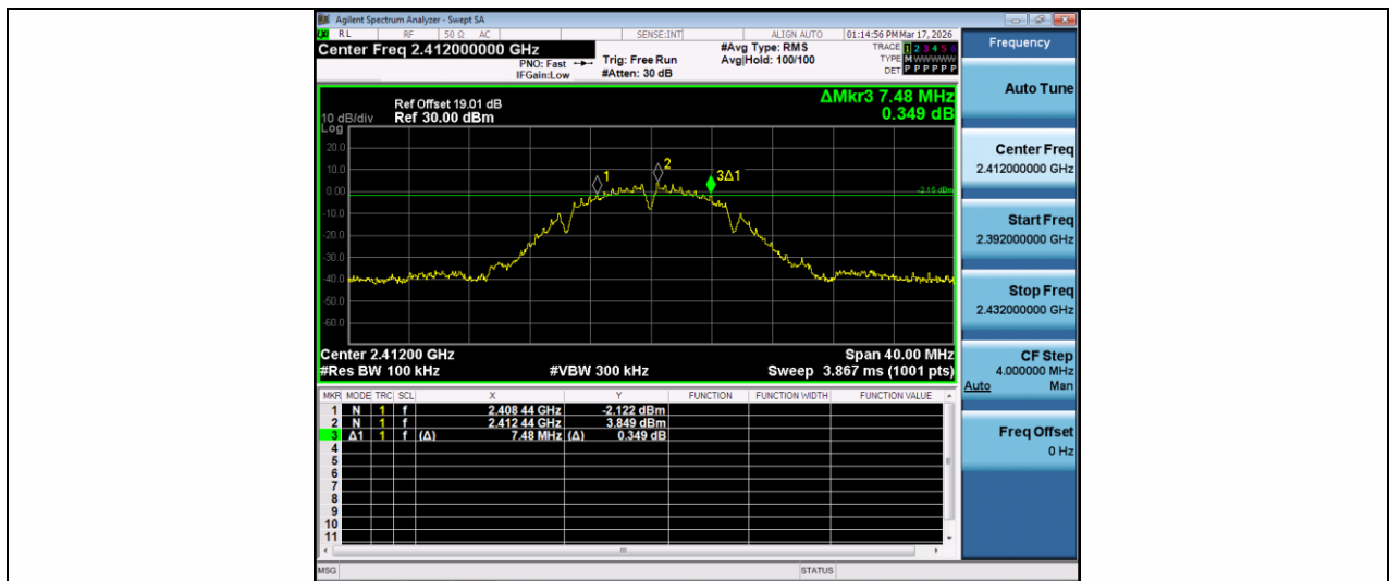
11B-Ant1-2412-PASS
