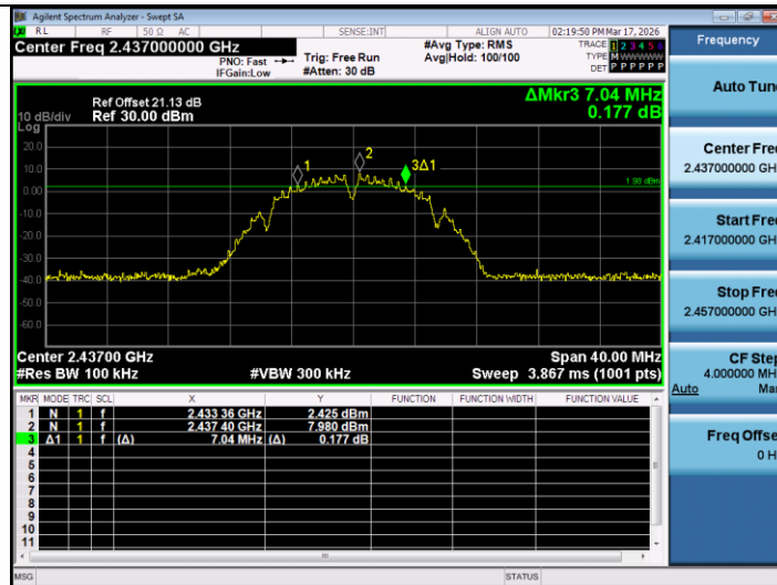
11B-Ant2-2437-PASS
