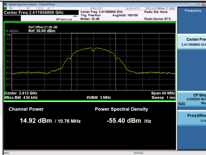
11B-Ant2-2412-PASS
