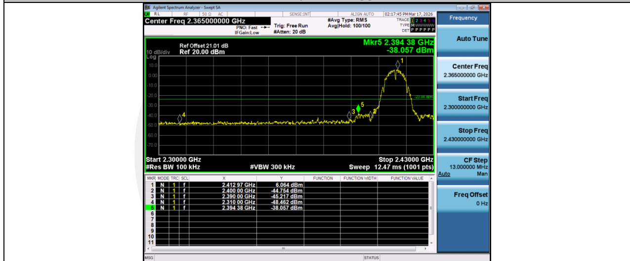
11B-Ant2-2412-PASS
