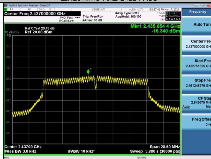
11N20MIMO-Ant1-2437-PASS
