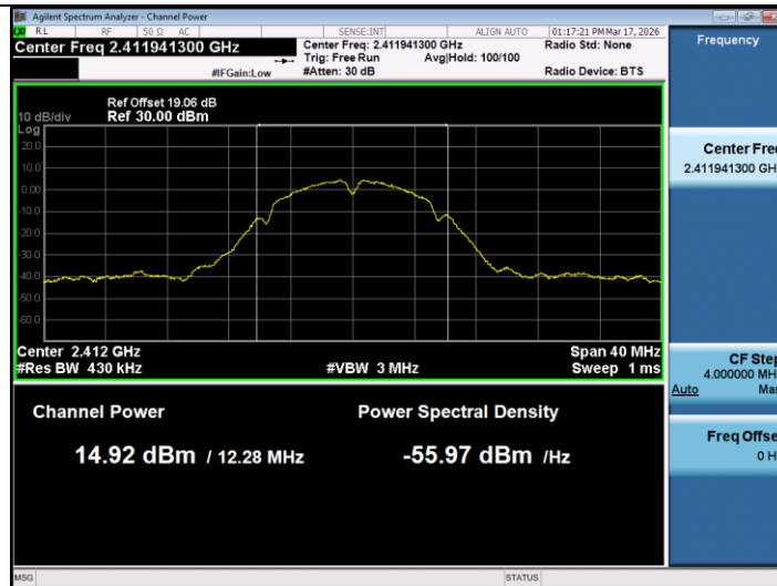
11B-Ant1-2412-PASS
