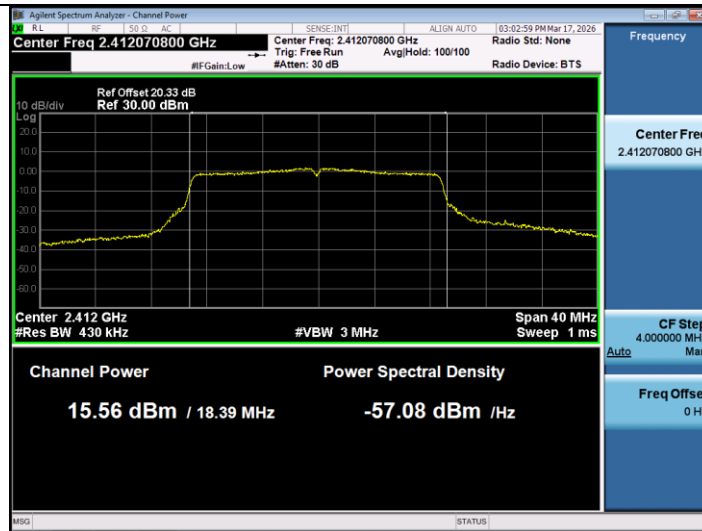
11N20MIMO-Ant1-2412-PASS
