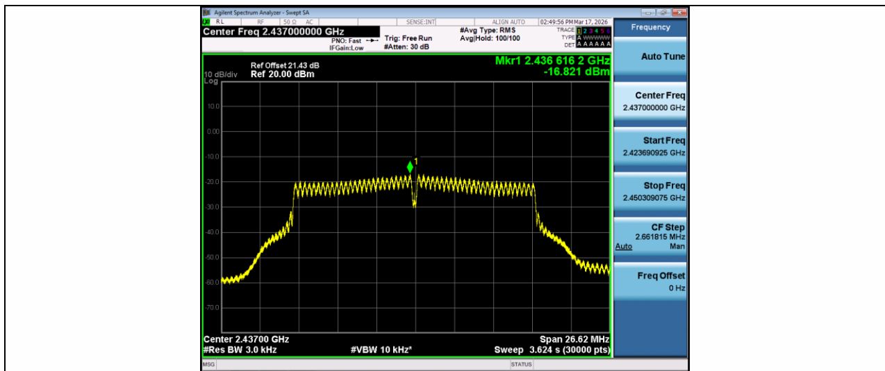
11G-Ant2-2437-PASS
