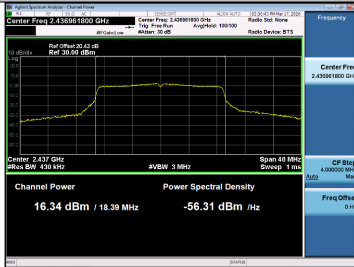
11N20MIMO-Ant1-2437-PASS
