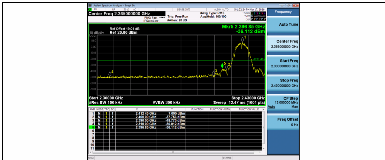
11B-Ant1-2412-PASS
