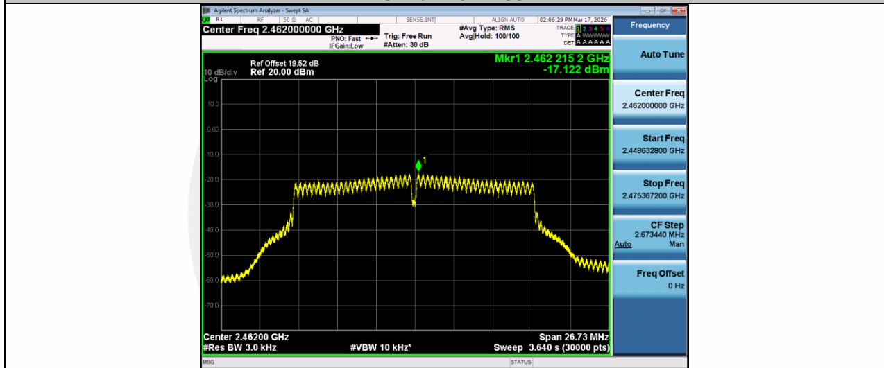
11G-Ant1-2462-PASS
