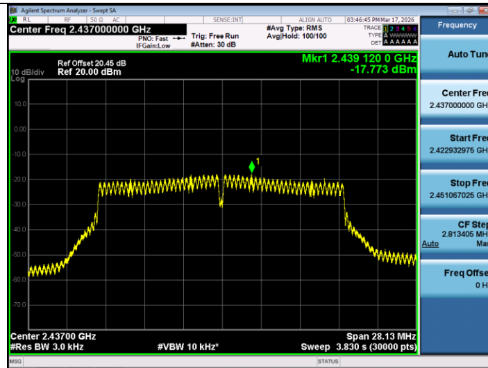
11N20MIMO-Ant2-2437-PASS
