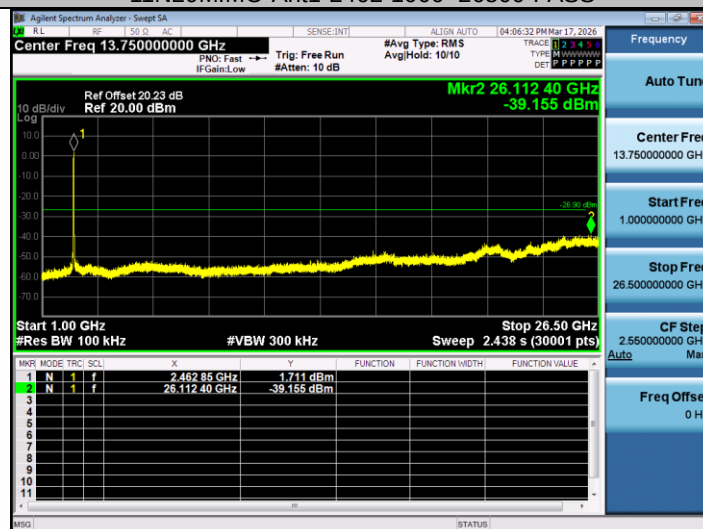
11N20MIMO-Ant2-2462-1000~26500-PASS
