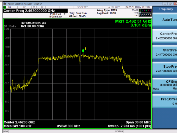
11N20MIMO-Ant2-2462-0~Reference-PASS
