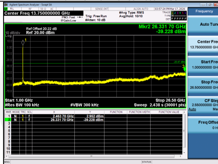
11N20MIMO-Ant1-2462-1000~26500-PASS
