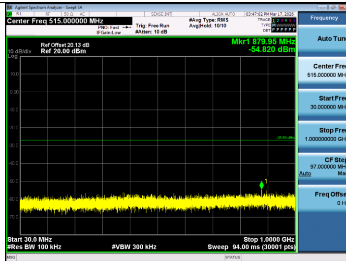
11N20MIMO-Ant2-2437-30~1000-PASS
