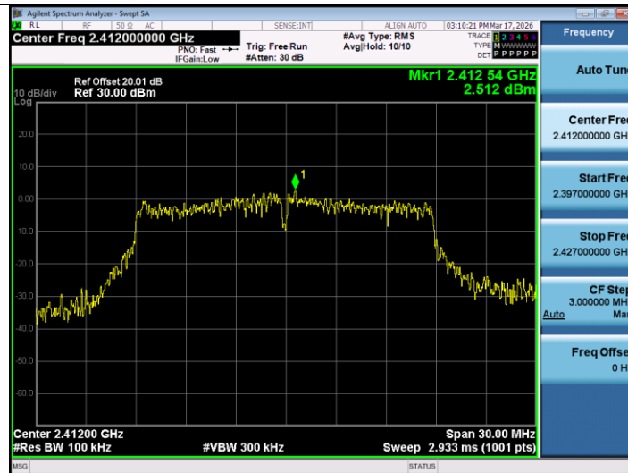
11N20MIMO-Ant1-2412-0~Reference-PASS
