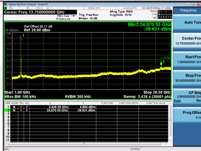
11N20MIMO-Ant1-2437-1000~26500-PASS
