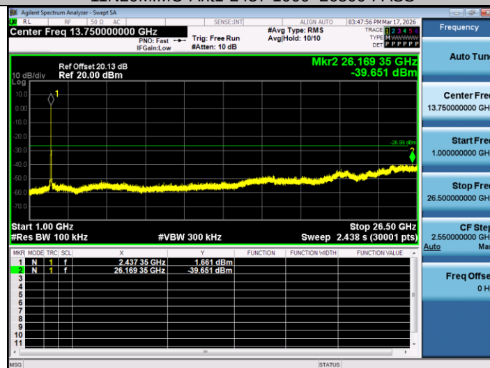
11N20MIMO-Ant2-2437-1000~26500-PASS
