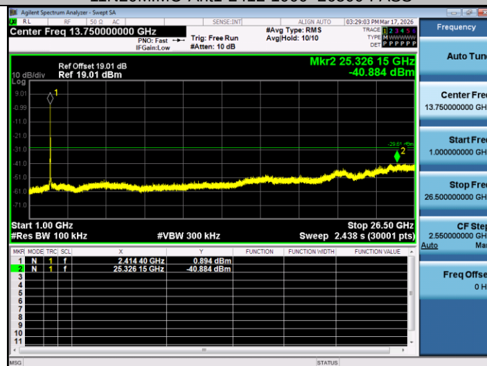
11N20MIMO-Ant2-2412-1000~26500-PASS
