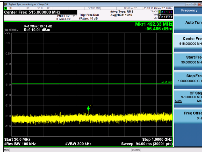
11N20MIMO-Ant2-2412-30~1000-PASS
