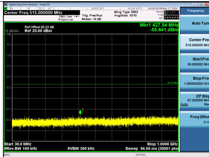
11N20MIMO-Ant2-2462-30~1000-PASS
