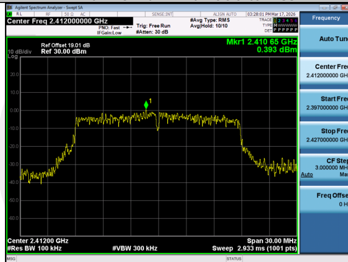
11N20MIMO-Ant2-2412-0~Reference-PASS
