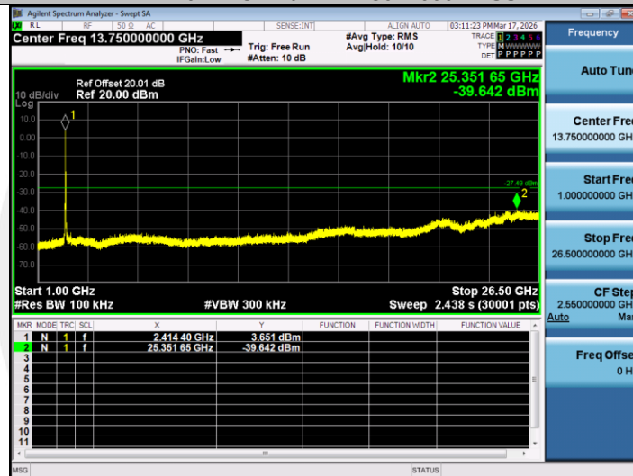
11N20MIMO-Ant1-2412-1000~26500-PASS
