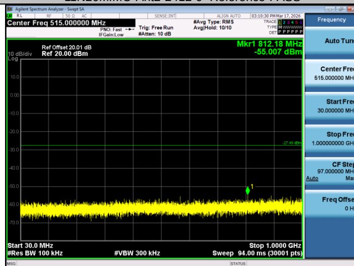
11N20MIMO-Ant1-2412-30~1000-PASS
