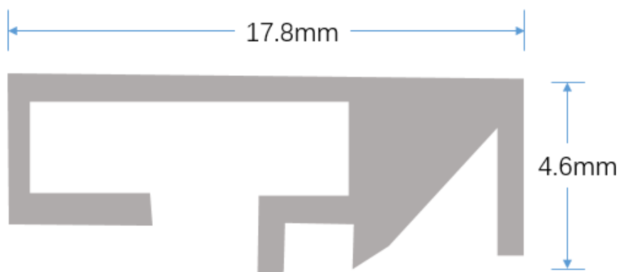
Antenna Size
