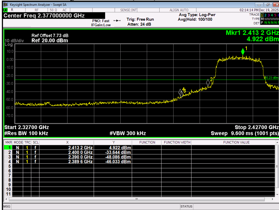
Band Edge NVNT 802.11n(HT20) 2412MHz Ant1 Emission
