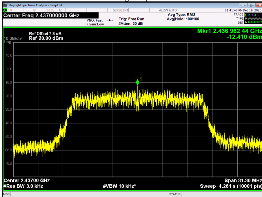
PSD NVNT 802.11g 6Mbps 2437MHz Ant1
