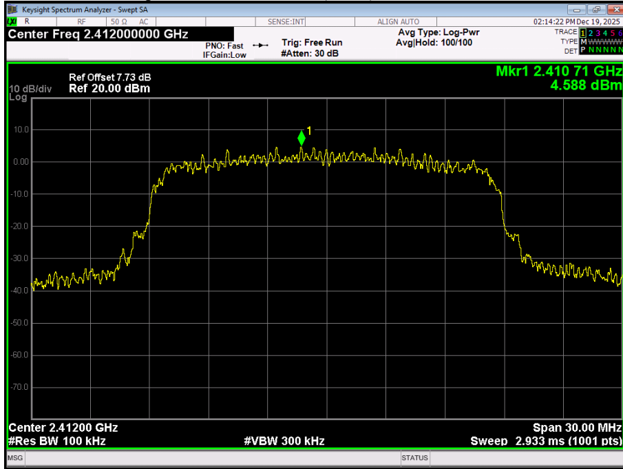
Tx. Spurious NVNT 802.11n(HT20) 2412MHz Ant1 Emission
