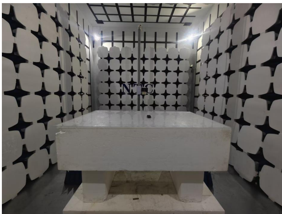
Photos of radiated emission test Above 1GHz
