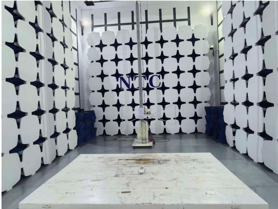
Photos of radiated emission test 30MHz – 1GHz
