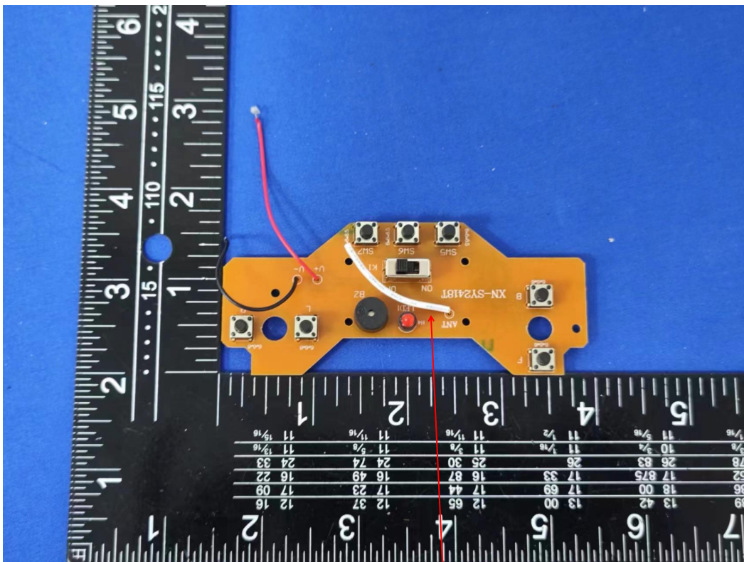
Internal antenna
