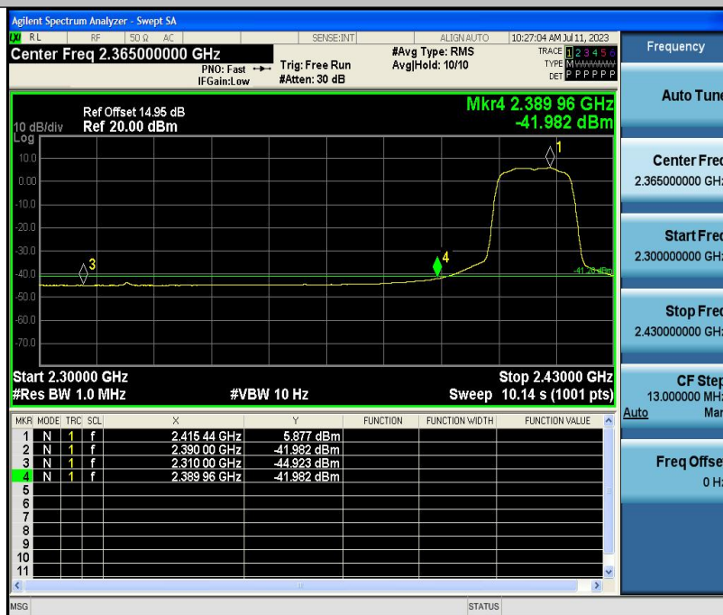
11G-Ant1-2412
