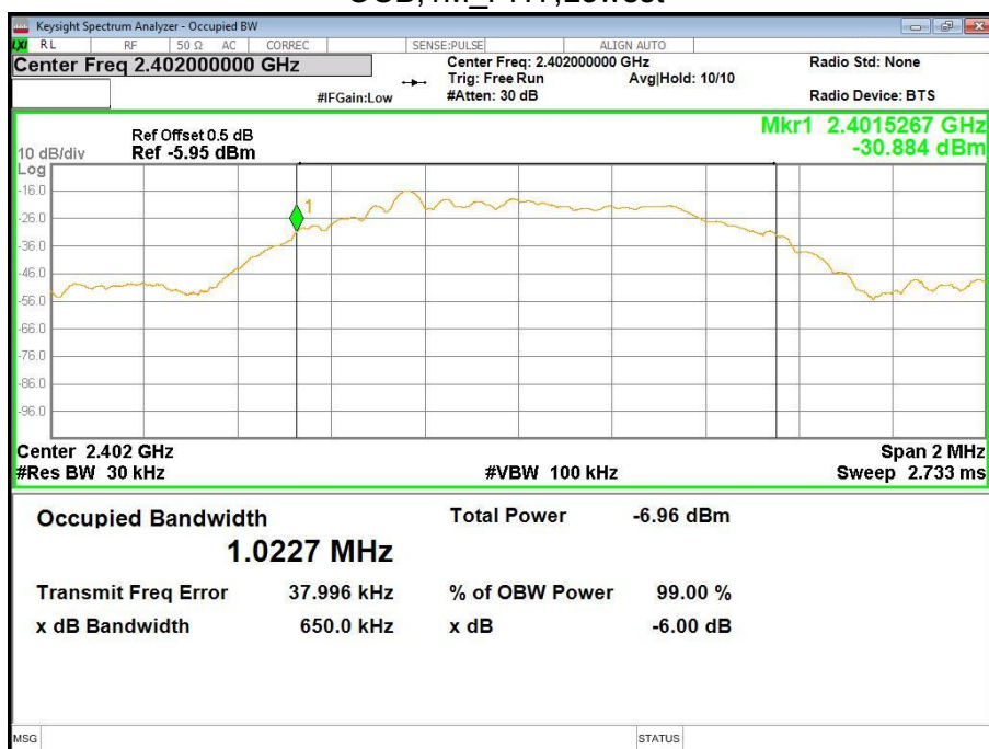
OCB,1M_PHY,Lowest
