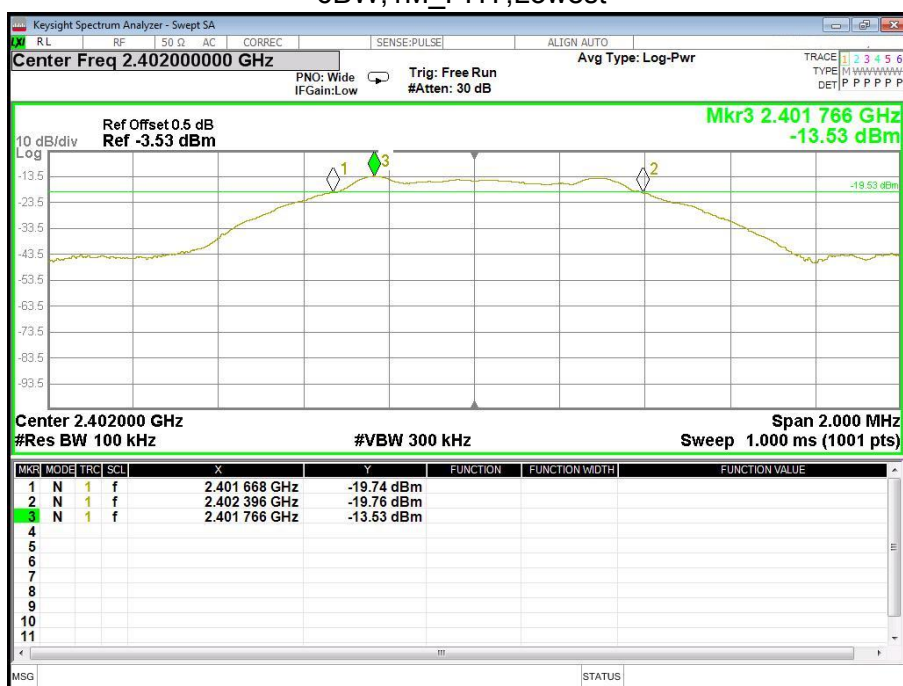
OCB,1M_PHY,Lowest
