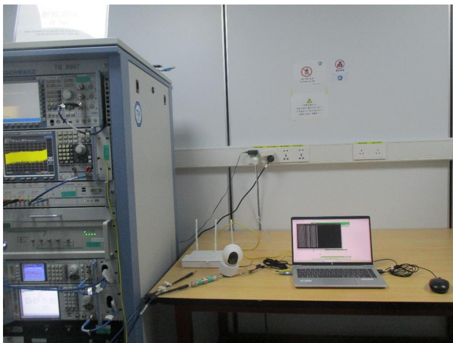
Dynamic Frequency Selection (DFS) test setup
