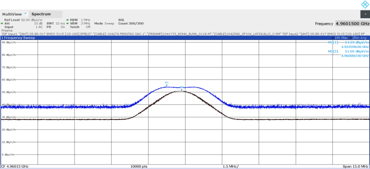
Fig. 43: Sample #2. Mode 1. Spurious Emission 4960 MHz. Channel High
