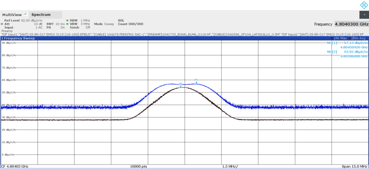
Fig. 39: Sample #2. Mode 1. Spurious Emission 4804 MHz. Channel Low
