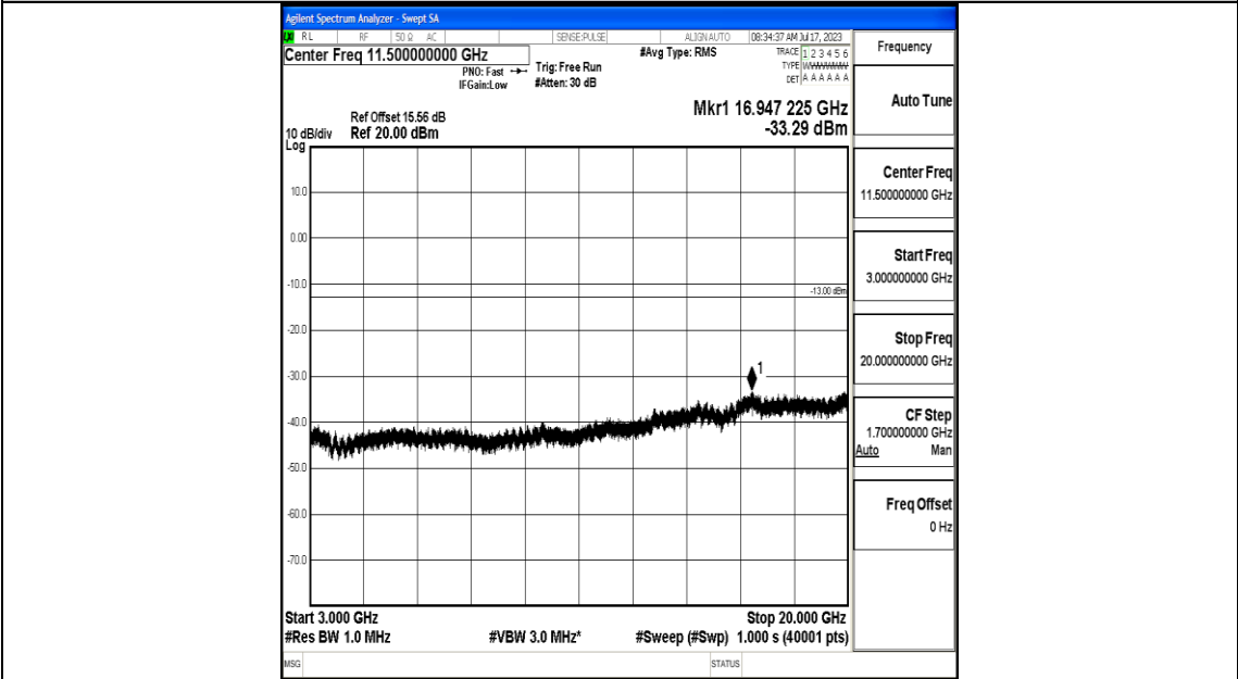
Band25_10MHz_QPSK_26090_1RB#0_3000~20000_3000~20000
