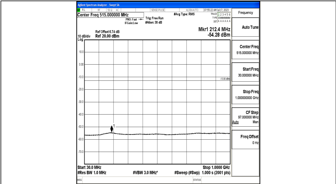
Band25_1.4MHz_16QAM_26683_1RB#0_30~1000_30~1000
