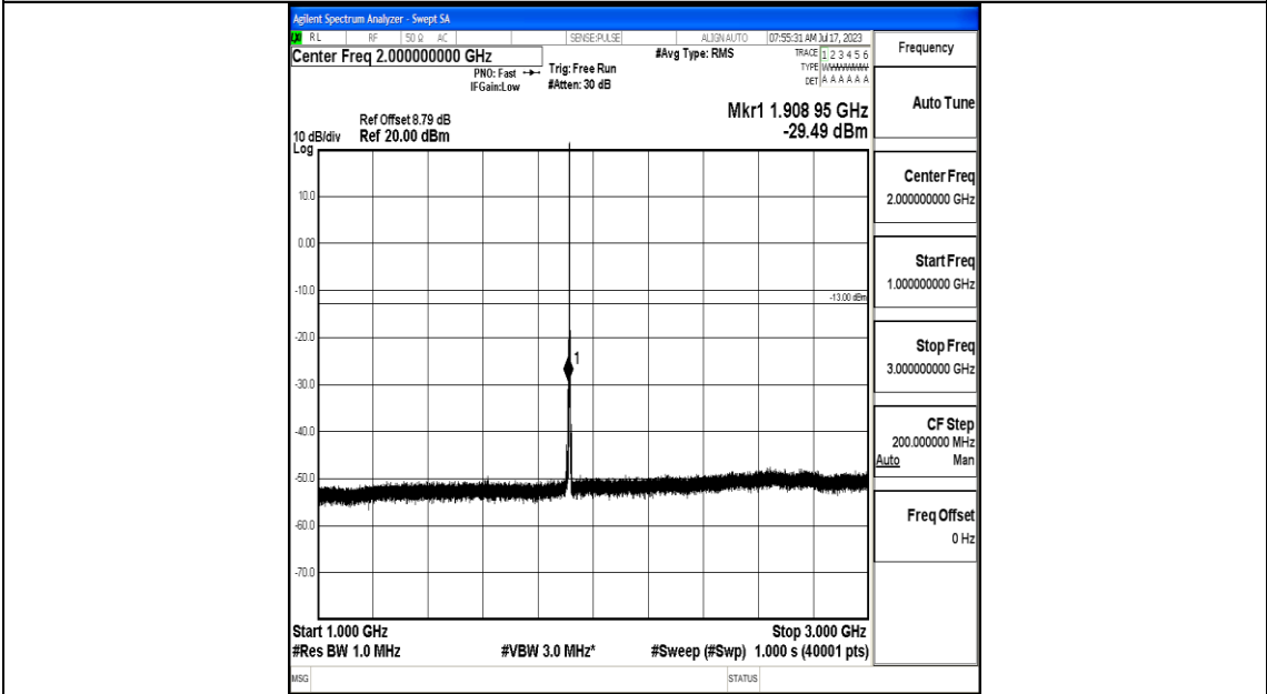
Band25_1.4MHz_16QAM_26683_1RB#0_1000~3000_1000~3000
