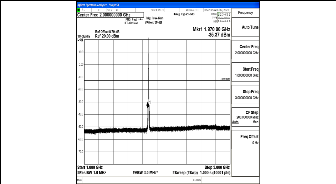
Band25_5MHz_16QAM_26365_1RB#0_1000~3000_1000~3000
