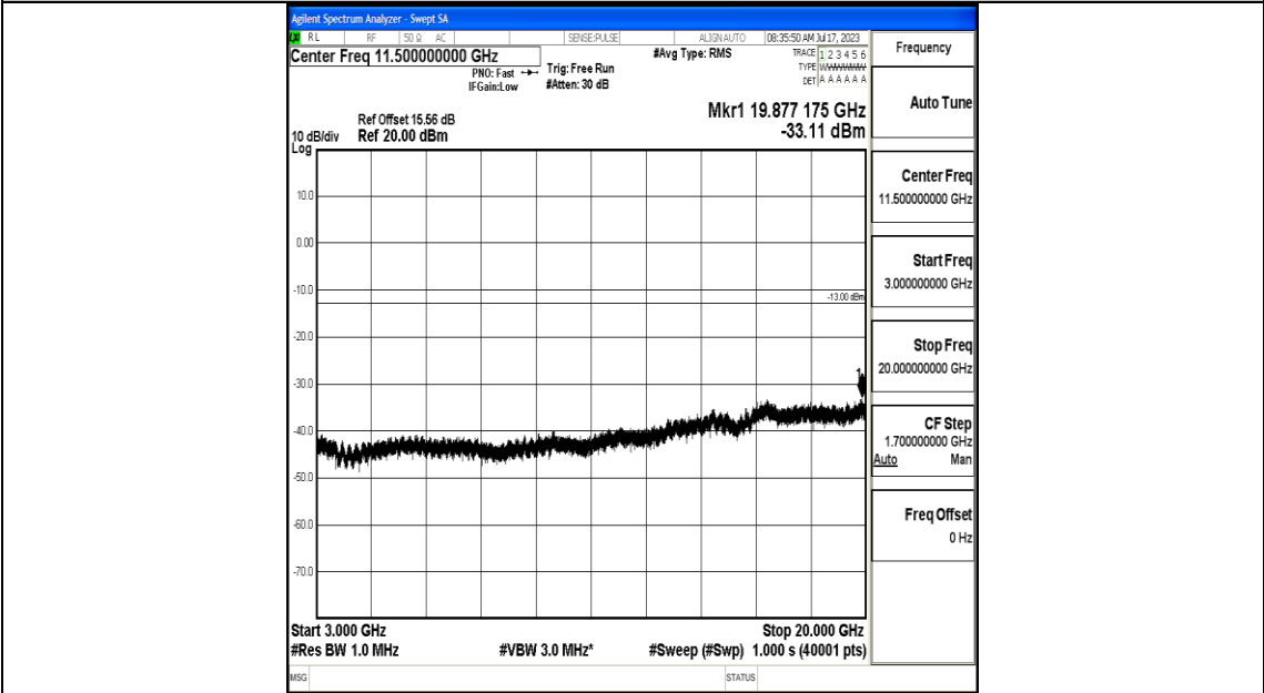
Band25_10MHz_QPSK_26365_1RB#0_3000~20000_3000~20000
