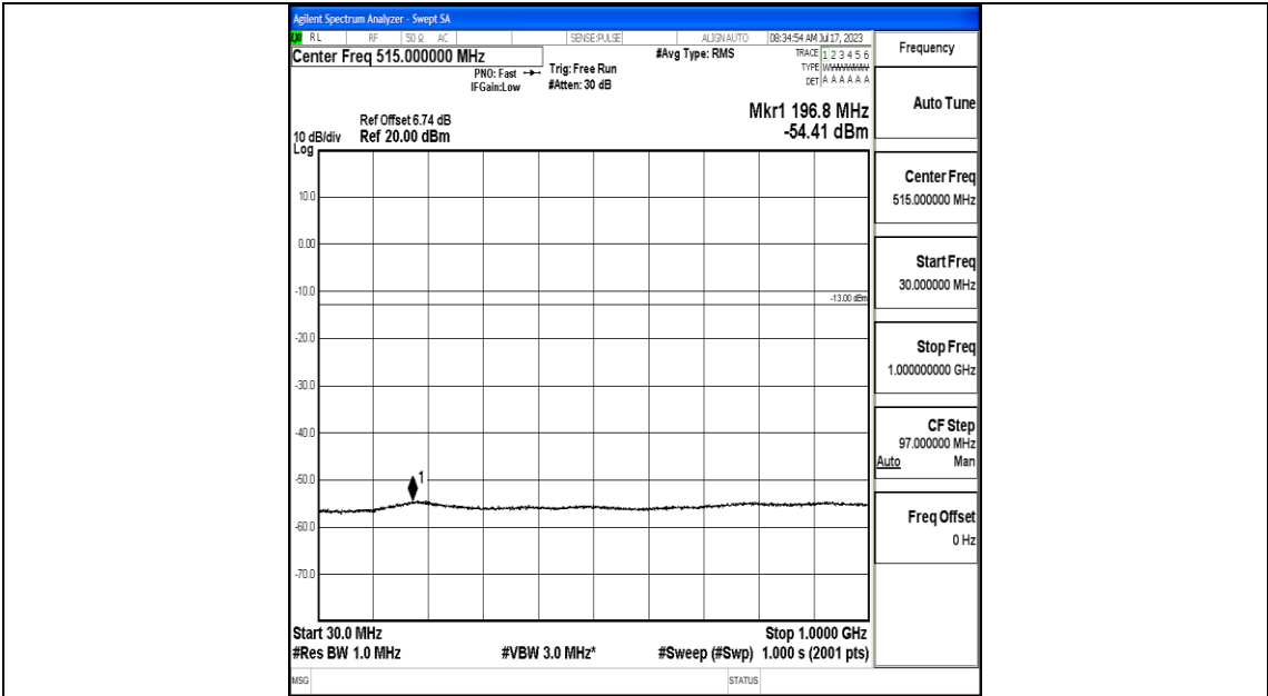
Band25_10MHz_16QAM_26090_1RB#0_30~1000_30~1000
