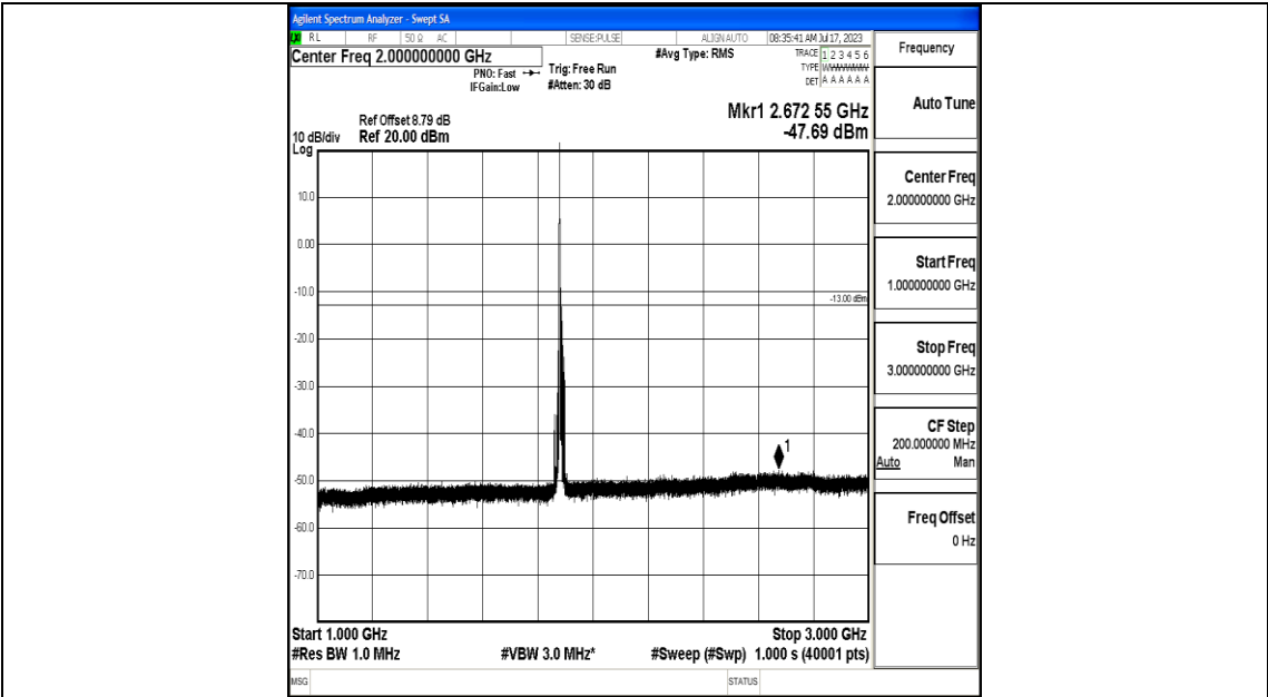
Band25_10MHz_QPSK_26365_1RB#0_1000~3000_1000~3000
