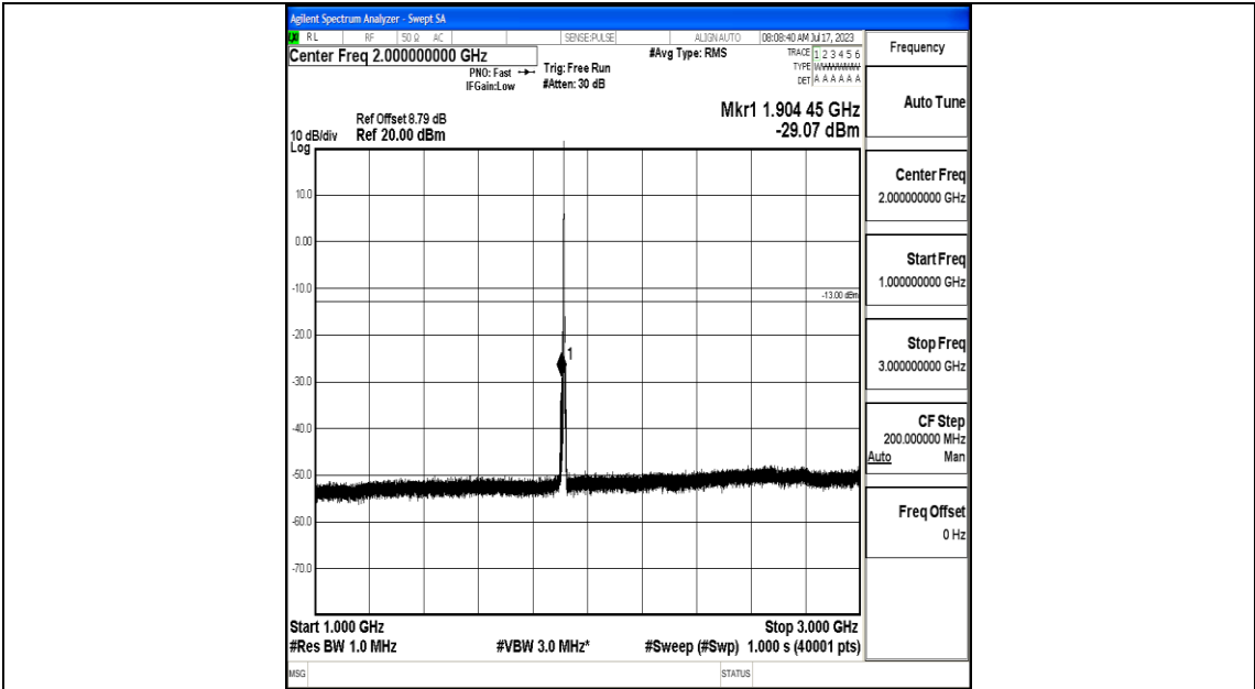
Band25_3MHz_QPSK_26675_1RB#0_1000~3000_1000~3000
