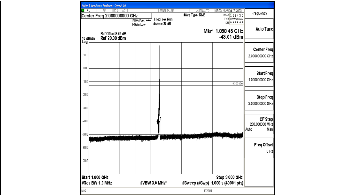
Band25_5MHz_QPSK_26665_1RB#0_1000~3000_1000~3000
