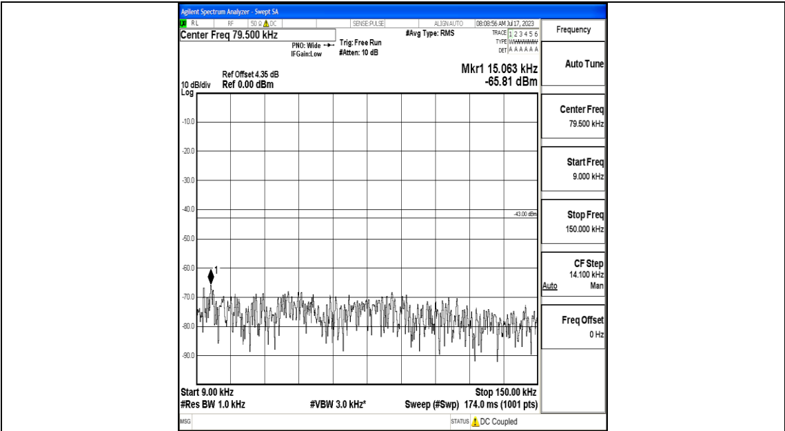
Band25_3MHz_16QAM_26675_1RB#0_0.009~0.15_0.009~0.15
