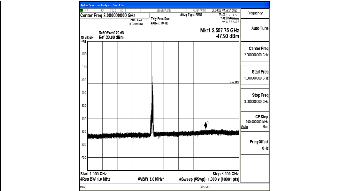
Band25_10MHz_QPSK_26090_1RB#0_1000~3000_1000~3000
