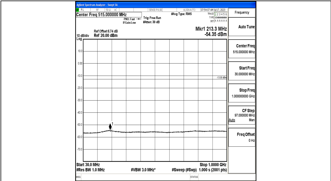
Band25_1.4MHz_16QAM_26365_1RB#0_30~1000_30~1000
