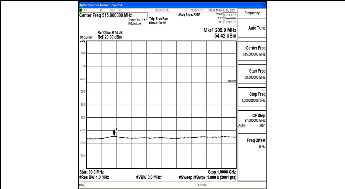
Band25_10MHz_QPSK_26090_1RB#0_30~1000_30~1000
