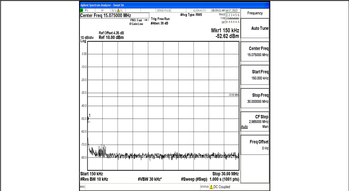
Band25_3MHz_16QAM_26675_1RB#0_0.15~30_0.15~30
