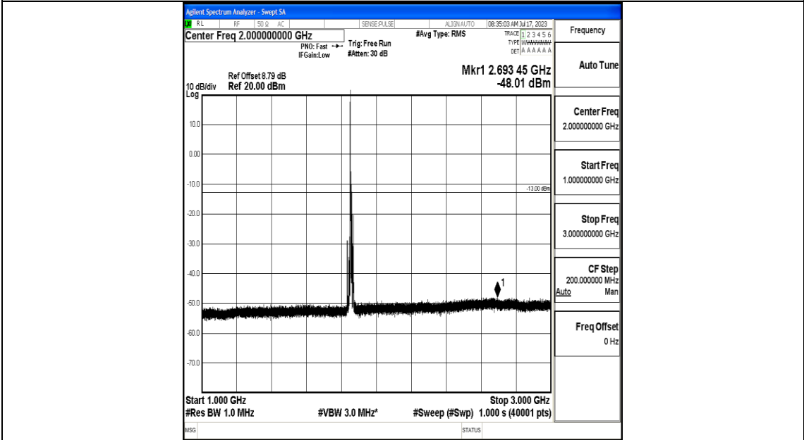
Band25_10MHz_16QAM_26090_1RB#0_1000~3000_1000~3000
