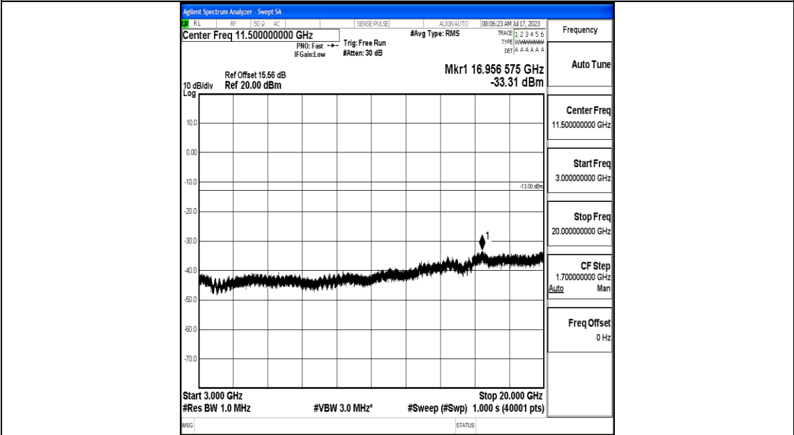
Band25_3MHz_QPSK_26055_1RB#0_3000~20000_3000~20000
