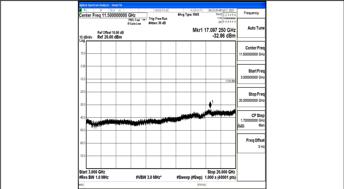
Band25_5MHz_QPSK_26665_1RB#0_3000~20000_3000~20000
