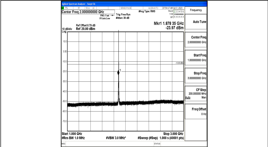
Band25_1.4MHz_16QAM_26365_1RB#0_1000~3000_1000~3000
