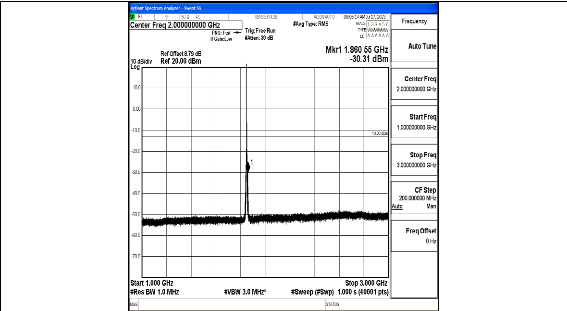
Band25_3MHz_QPSK_26055_1RB#0_1000~3000_1000~3000
