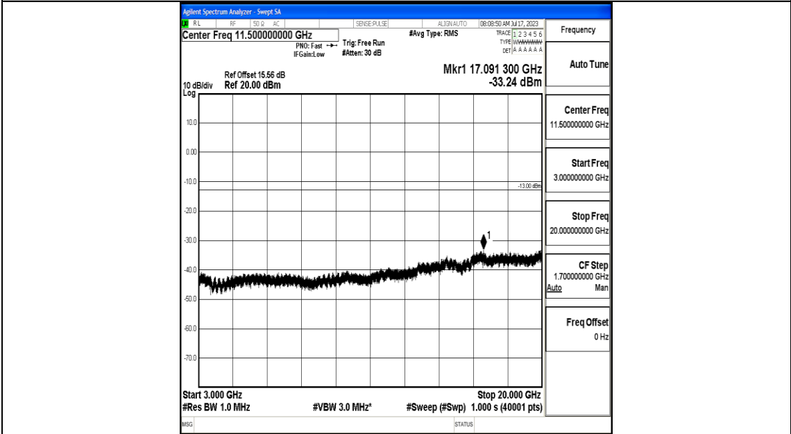
Band25_3MHz_QPSK_26675_1RB#0_3000~20000_3000~20000
