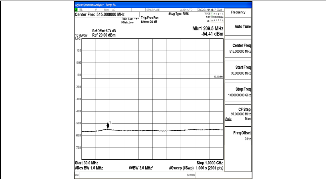
Band25_5MHz_16QAM_26365_1RB#0_30~1000_30~1000
