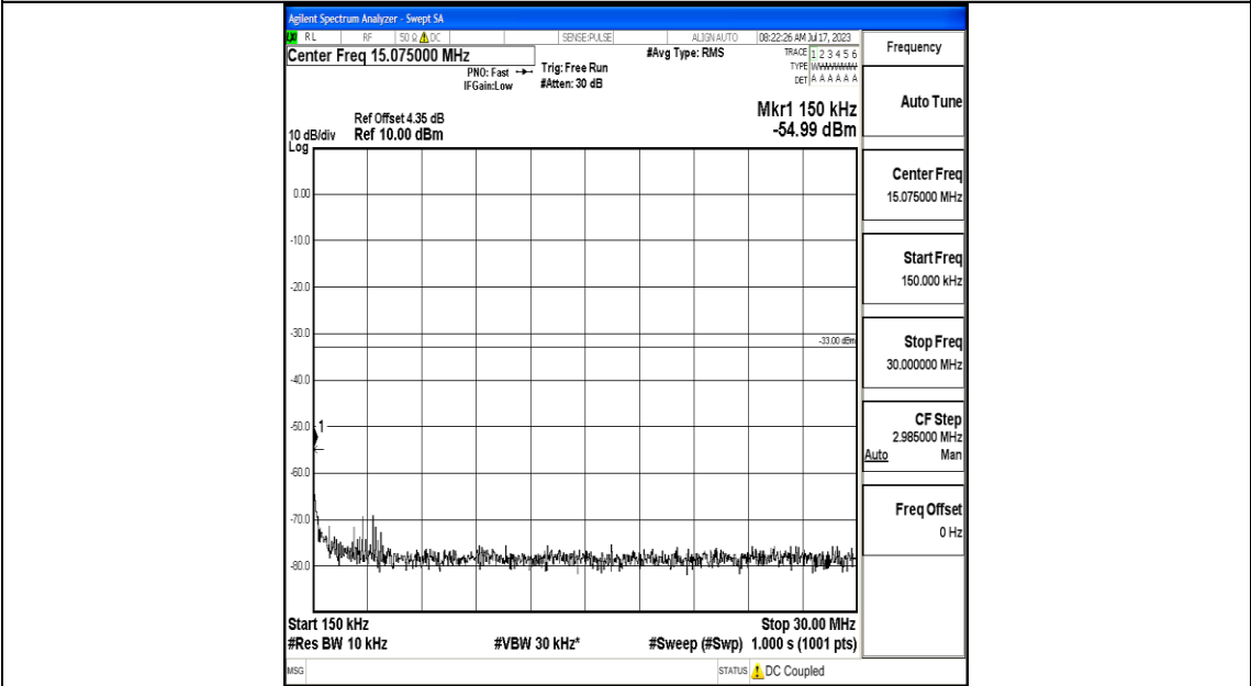
Band25_5MHz_16QAM_26365_1RB#0_0.15~30_0.15~30
