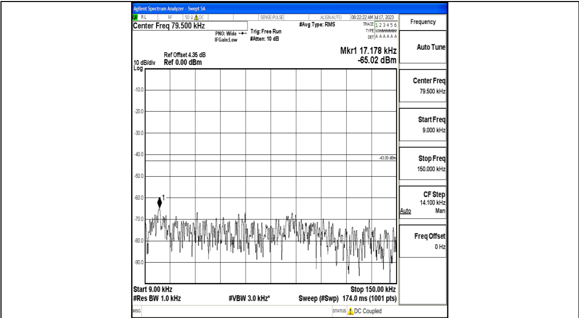
Band25_5MHz_16QAM_26365_1RB#0_0.009~0.15_0.009~0.15
