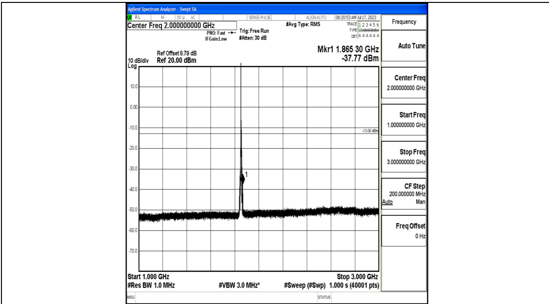
Band25_5MHz_QPSK_26065_1RB#0_1000~3000_1000~3000
